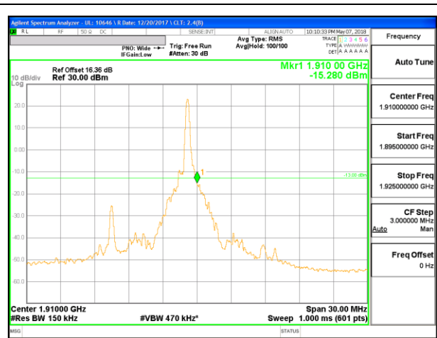
LTE B2 15MHz 16QAM High Channel RB1-74
