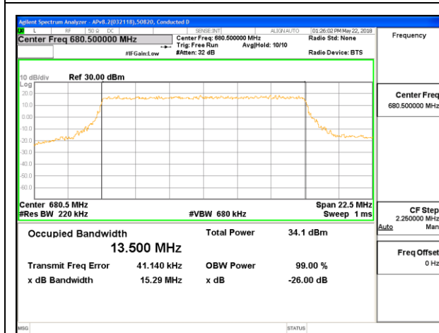
LTE B71 15MHz 64QAM Middle Channel RB75-0
