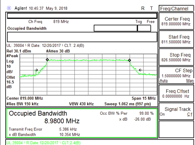
LTE B26 10MHz 64QAM Middle Channel RB25-0
