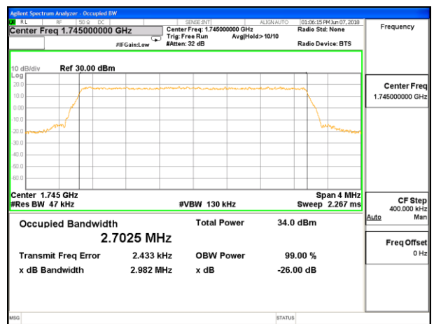
LTE B66 3MHz QPSK Middle Channel RB15-0 ID:39004
