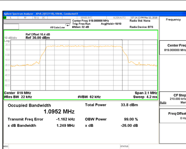
LTE B26 1.4MHz 16QAM Middle Channel RB6-0
