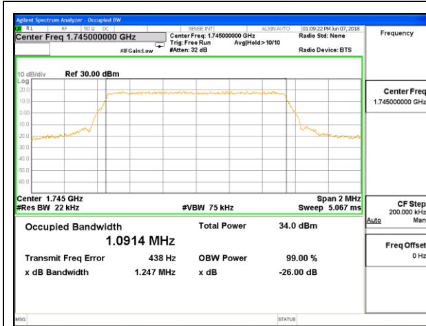
LTE B66 1.4MHz QPSK Middle Channel RB6-0 ID:39004
