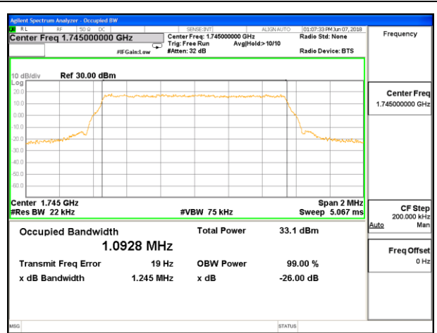
LTE B66 1.4MHz 16QAM Middle Channel RB6-0 ID:39004
