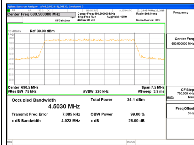
LTE B71 5MHz 64QAM Middle Channel RB25-0
