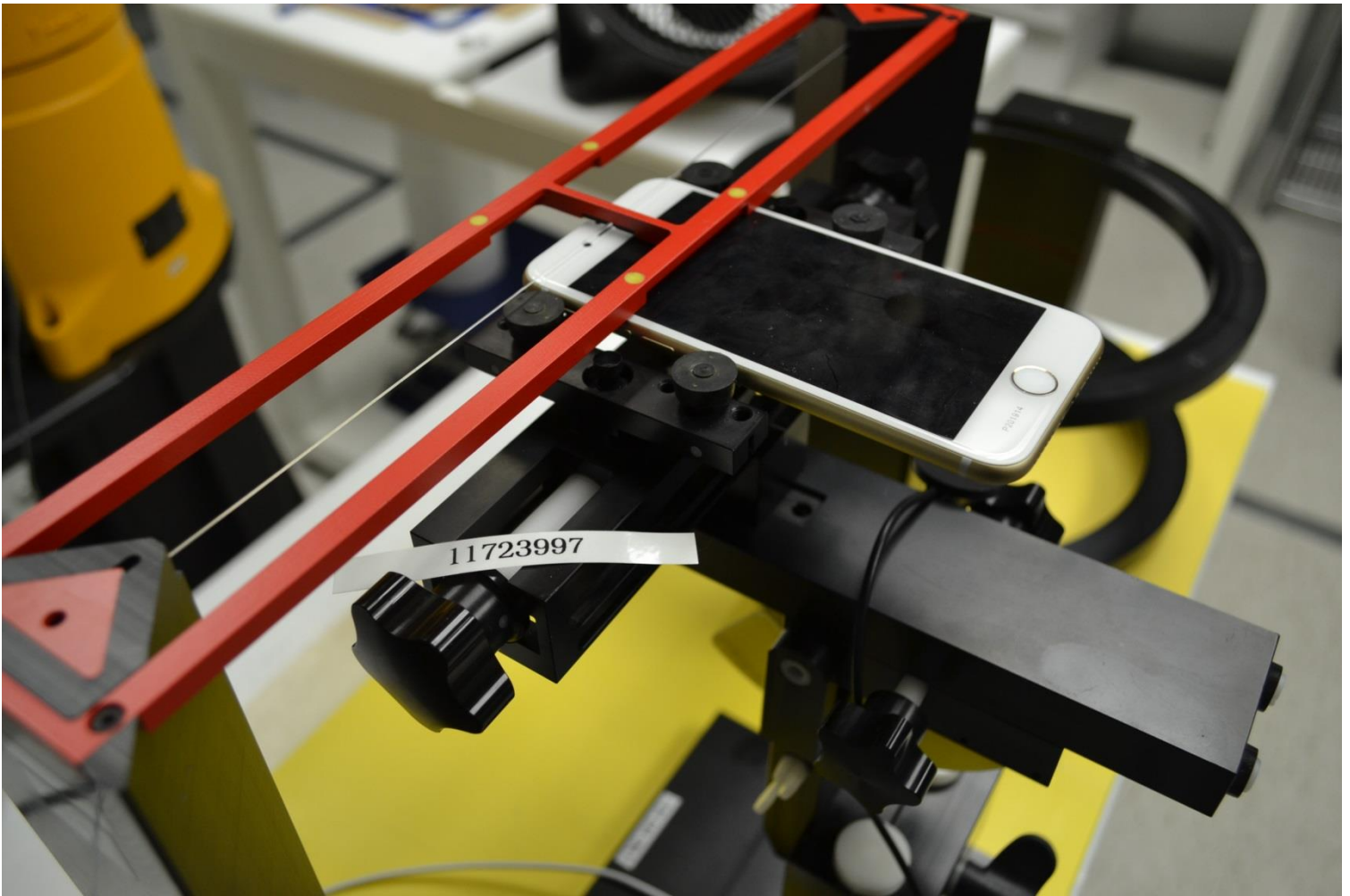
SETUP PHOTO Front View of the DUT
