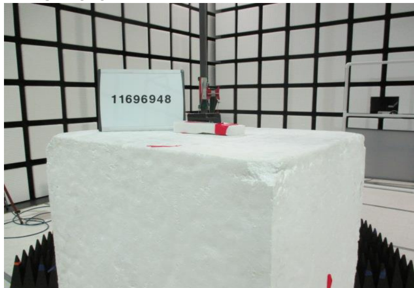
Y-AXIS PHOTO
