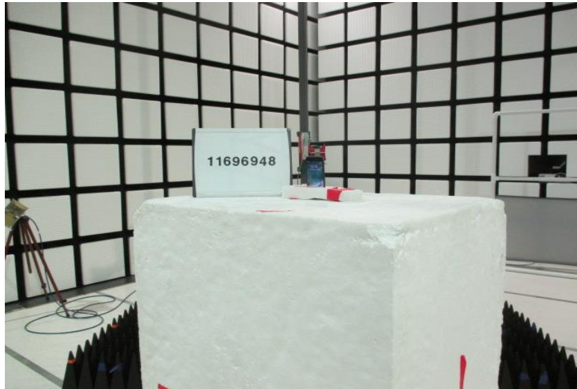
Z-AXIS PHOTO
