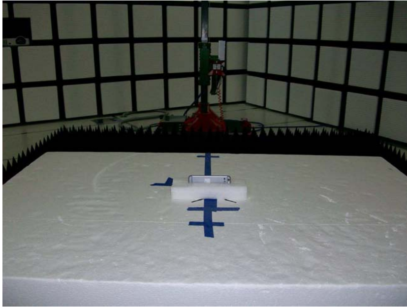
Y-AXIS PHOTO
