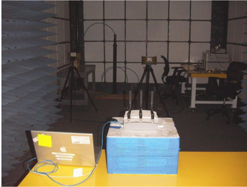
DFS BACK PHOTO (CLIENT MODE SETUP)
