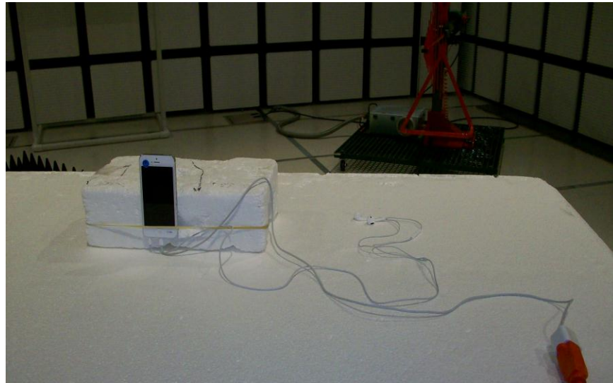
Z-AXIS PHOTO
