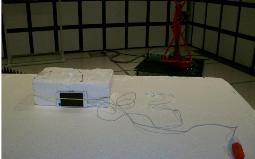
Y-AXIS PHOTO
