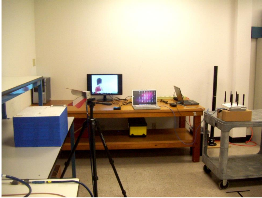
DFS FRONT PHOTO (FULL CLIENT-TO-CLIENT COMMUNICATIONS SETUP)
