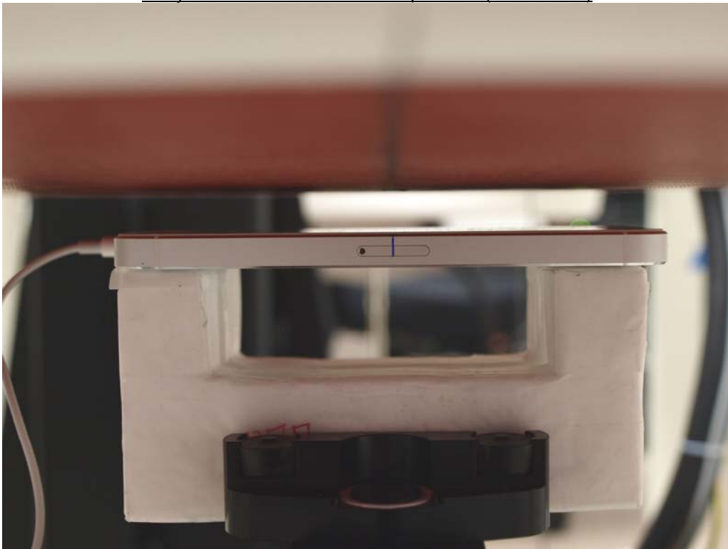
Body-worn - Front w/ 10 mm Separation (w/ Headset)
