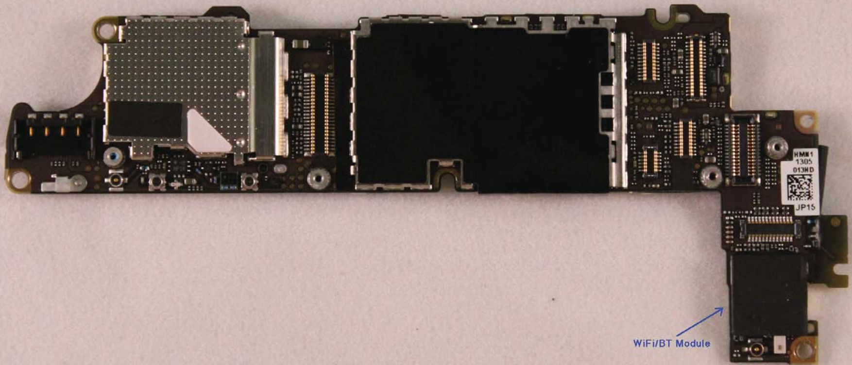
A1387 - Photo 13 Main Circuit Board front side
