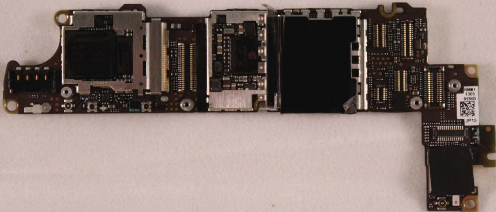
A1387 - Photo 14 Main Circuit Board front side Shields removed
