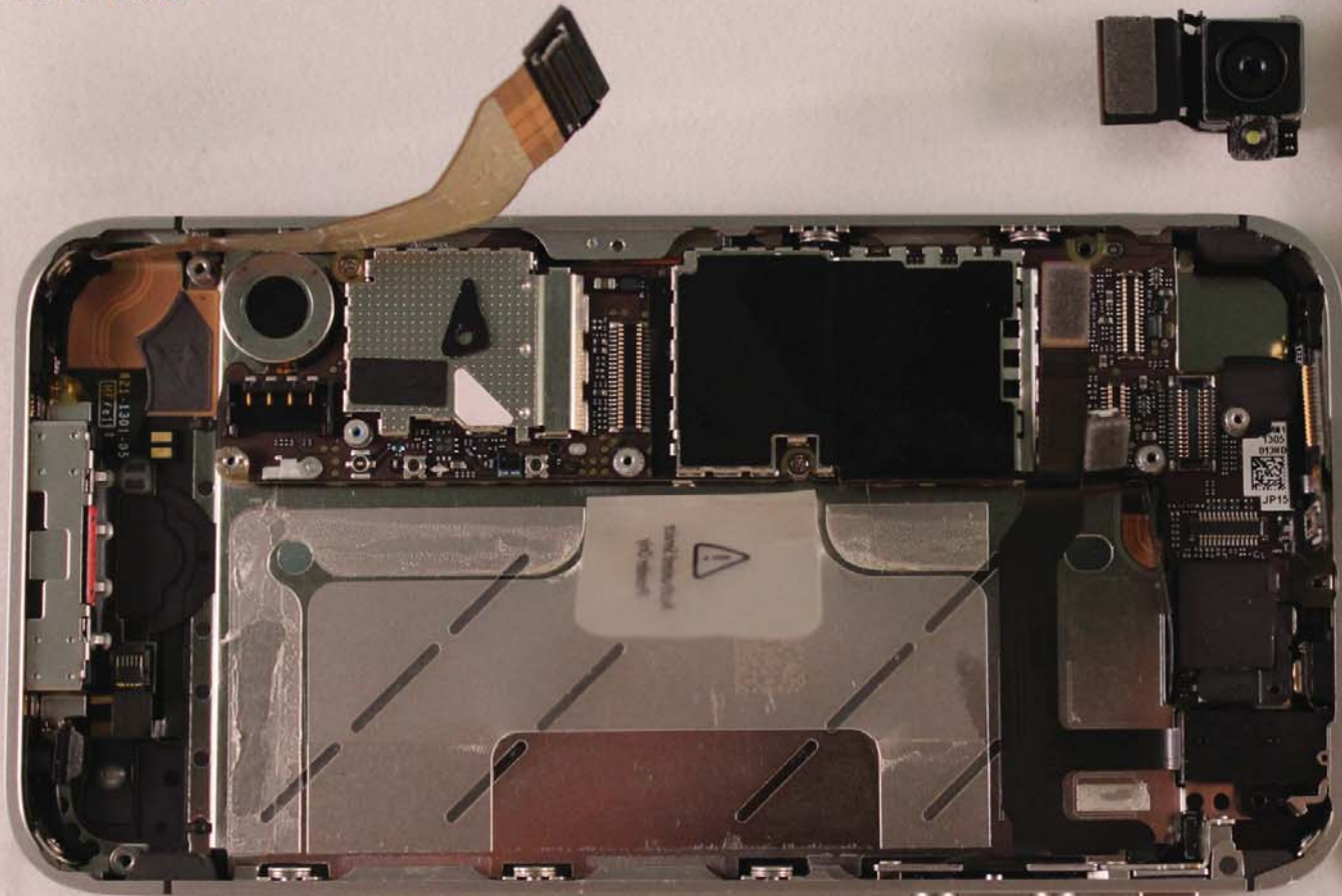
A1387 - Photo 10 Rear Camera removed
