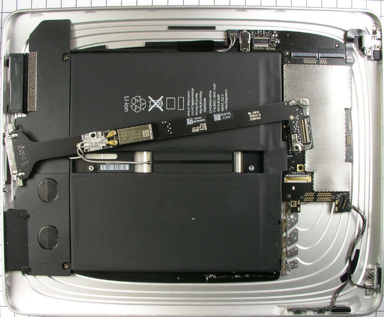
PHOTO 4 BOTTOM HOUSNG UNDERSIDE OF RIGID FLEX
