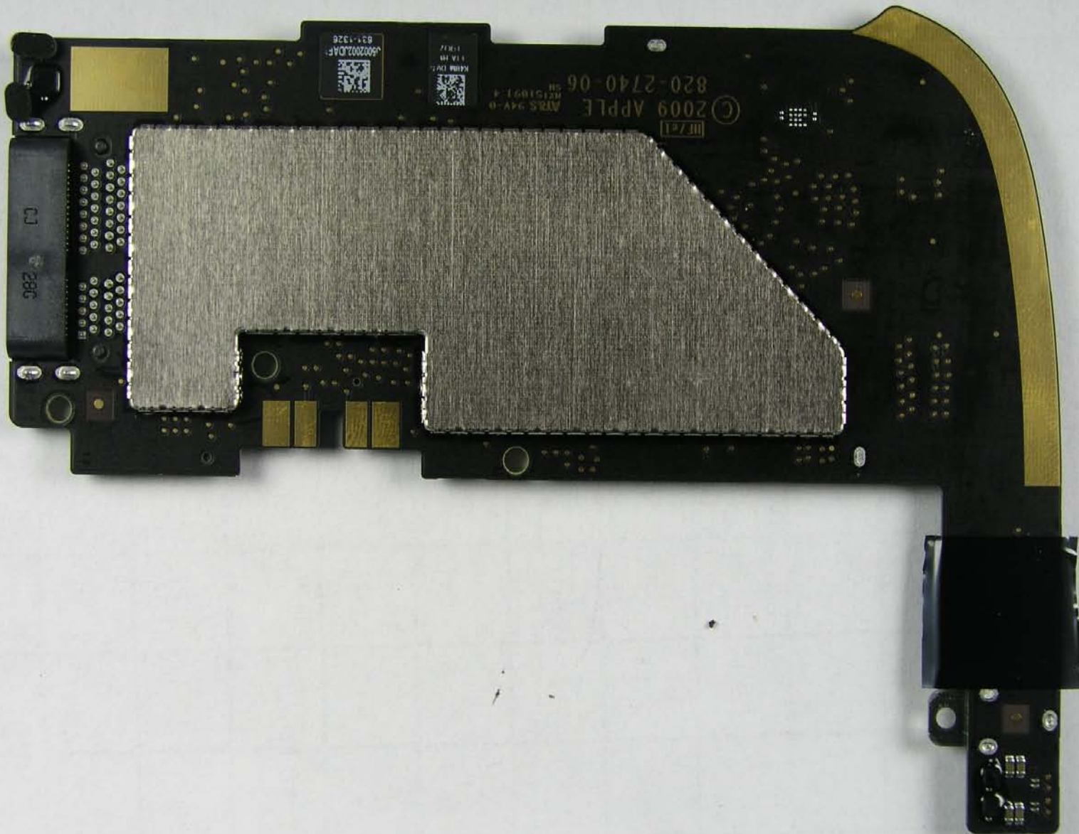
PHOTO 11 MAIN LOGIC BOARD BOTTOM SIDE
