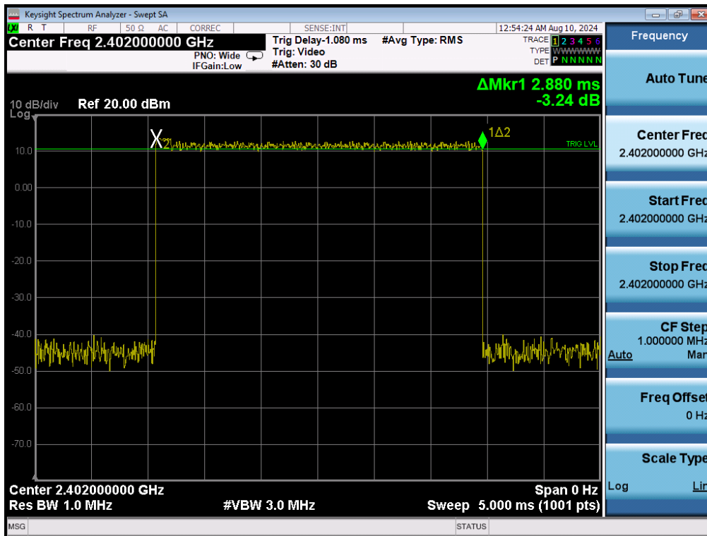
Plot 7-18. Time of Occupancy Plot (Bluetooth, 8DPSK, iPA)
