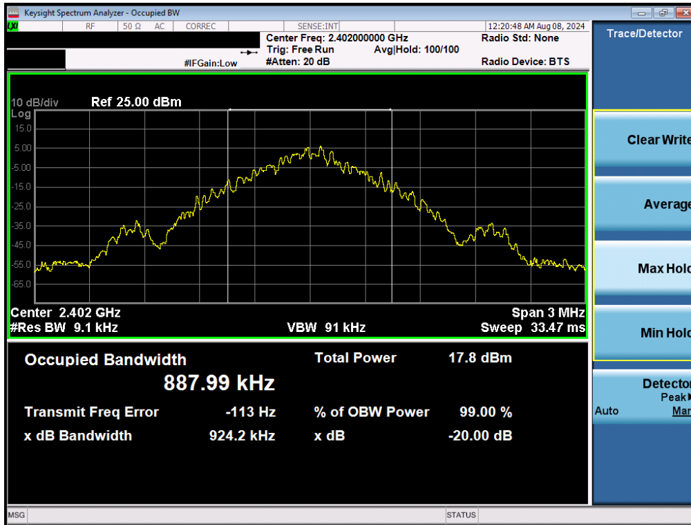
Plot 7-1. 20dB BW and 99% OBW Plot (Bluetooth, GFSK, iPA – Ch. 0)
