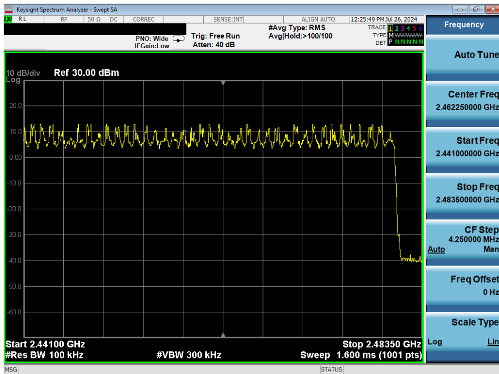
Plot 7-22. High End Spectrum Channel Hopping Plot (Bluetooth, 8DPSK, iPA)
