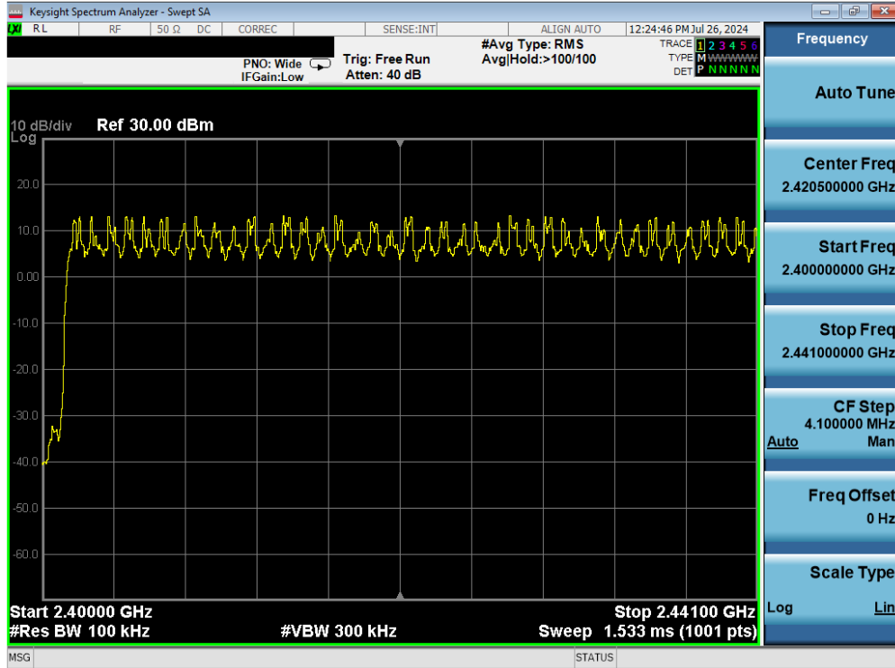
Plot 7-21. Low End Spectrum Channel Hopping Plot (Bluetooth, 8DPSK, iPA)
