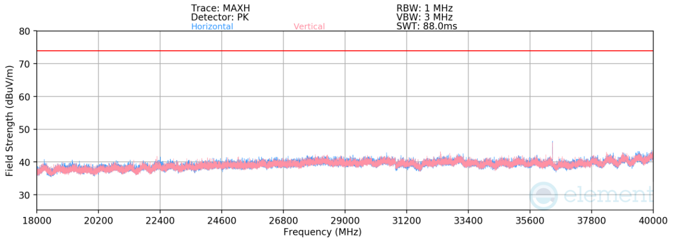
Plot 7-75. Radiated Spurious Emissions 18-40GHz (NB UNII BDR – 5201MHz)
