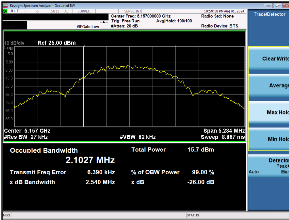
Plot 7-4. 26dB BW & 99% OBW (NB UNII LE2M – 5157MHz)
