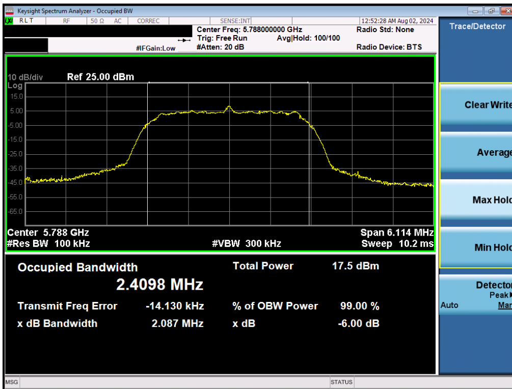
Plot 7-32. 6dB BW & 99% OBW (NB UNII HDRp4 – 5788MHz)
