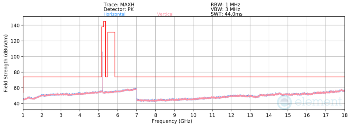
Plot 7-79. Radiated Spurious Emissions 1-18GHz (NB UNII LE2M - 5201MHz)
