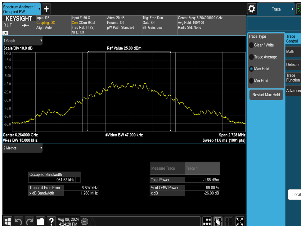
Plot 7-2. 26dB BW & 99% OBW (NB UNII BDR – 6264MHz)
