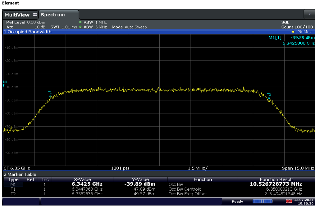
Plot 7-55. AWGN Signal
