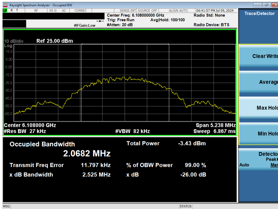
Plot 7-4. 26dB BW & 99% OBW (NB UNII LE, 2Mbps – 6108MHz)
