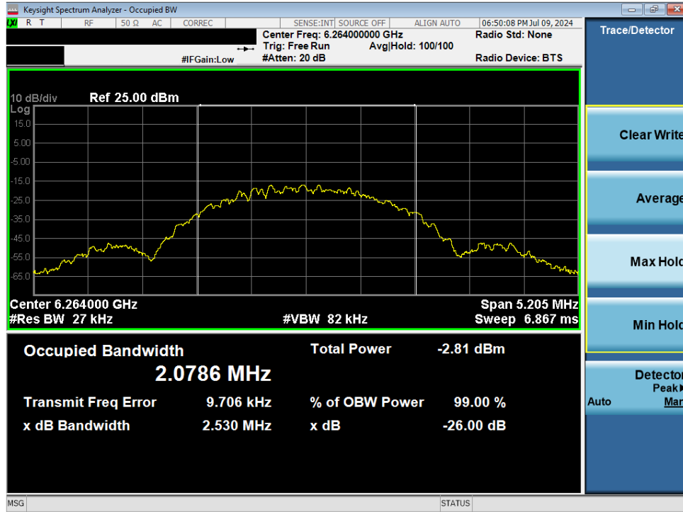
Plot 7-5. 26dB BW & 99% OBW (NB UNII LE, 2Mbps – 6264MHz)
