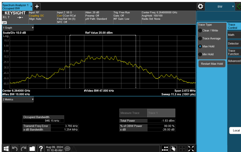
Plot 7-2. 26dB BW & 99% OBW (NB UNII BDR – 6264MHz)
