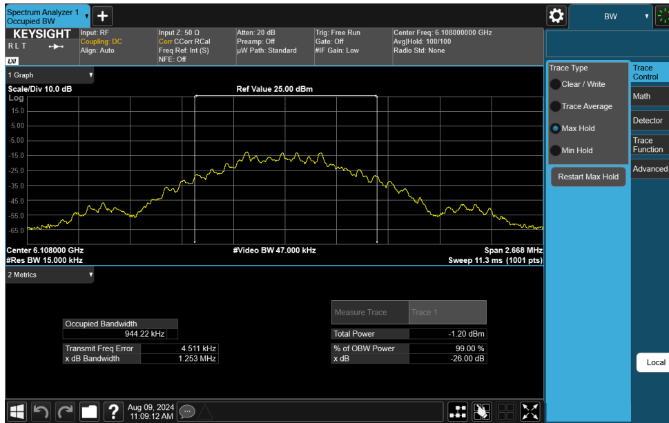
Plot 7-1. 26dB BW & 99% OBW (NB UNII BDR – 6108MHz)
