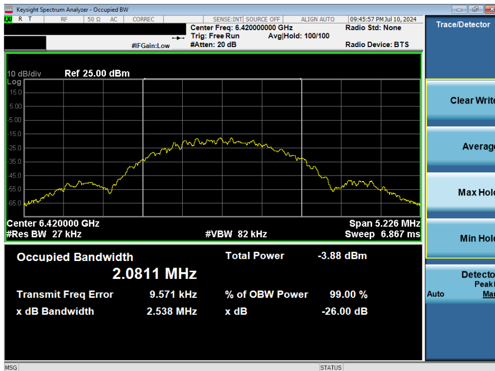
Plot 7-6. 26dB BW & 99% OBW (NB UNII LE, 2Mbps – 6420MHz)
