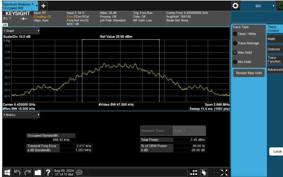
Plot 7-3. 26dB BW & 99% OBW (NB UNII BDR – 6420MHz)
