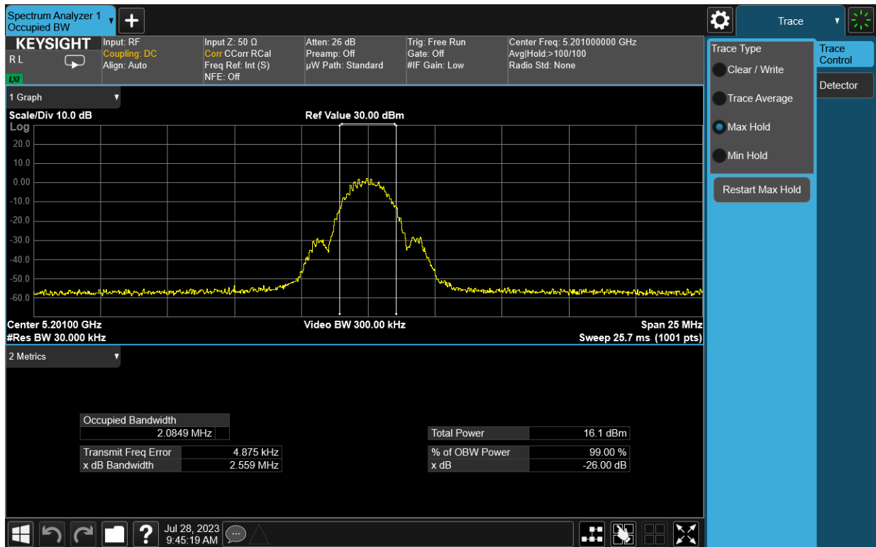
Plot 7-2. 26dB BW & 99% OBW (LE2M, 5201MHz)
