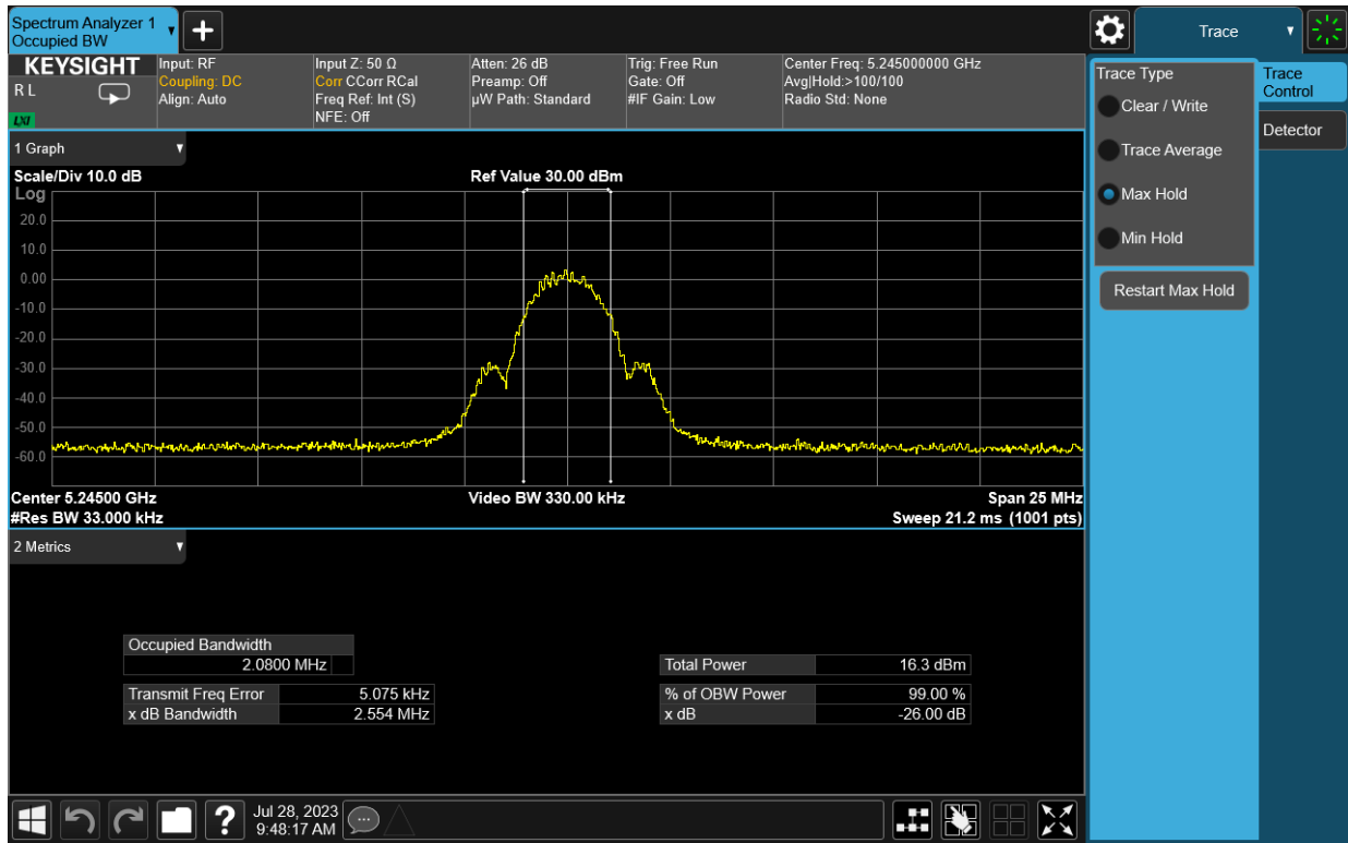
Plot 7-3. 26dB BW & 99% OBW (LE2M, 5245MHz)
