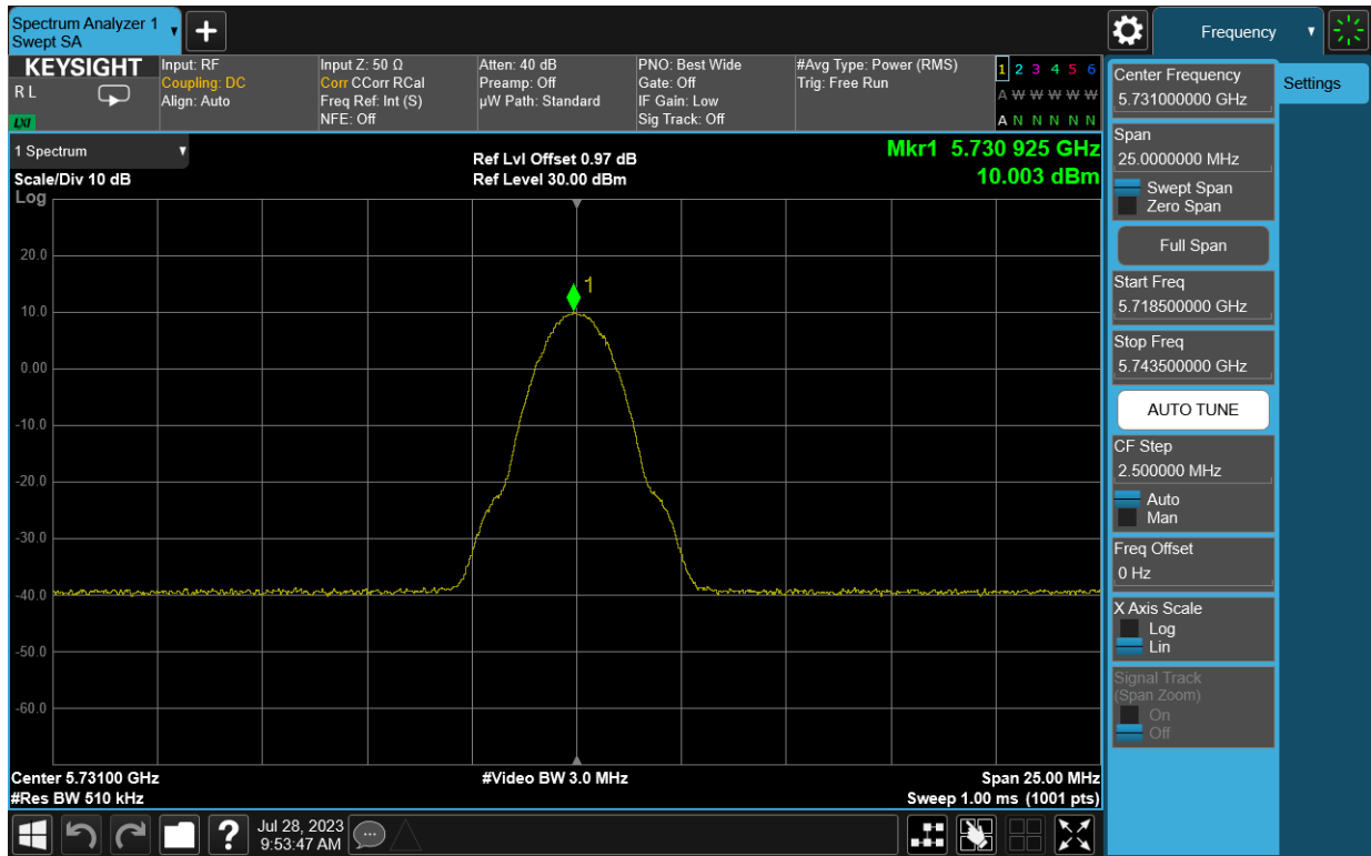
Plot 7-10. PSD (LE2M, 5731MHz)
