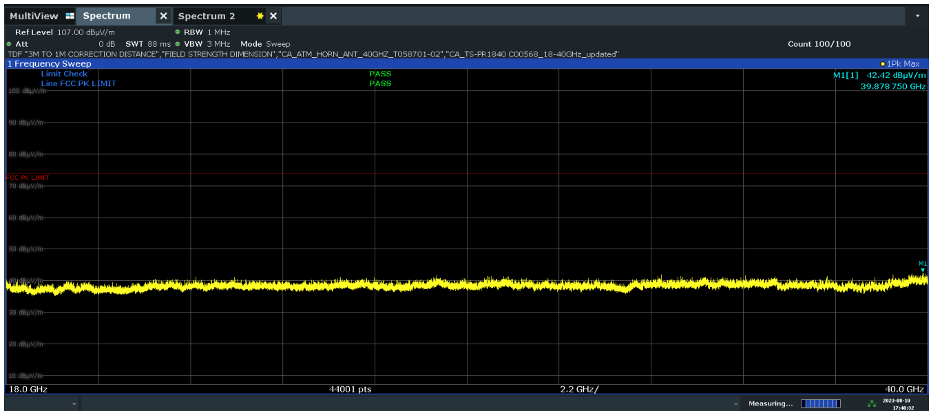
Plot 7-17. Radiated Spurious Emissions Above 18GHz (LE2M – 5157MHz Pol. V)
