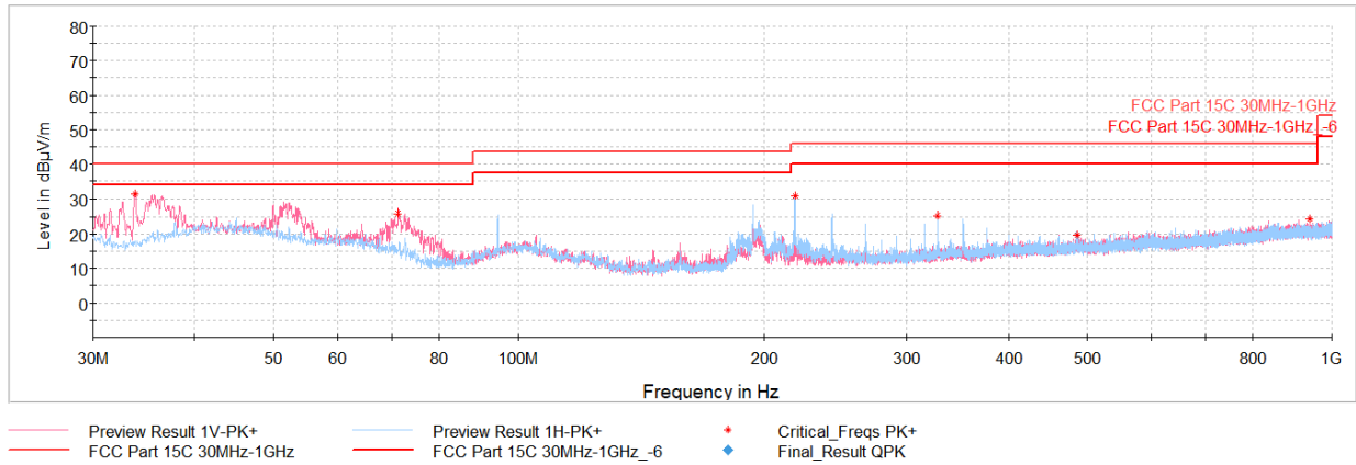
Plot 7-24. RSE 30MHz - 1GHz (LE2M – 5731MHz), with AC/DC Adapter and USB-C cable
