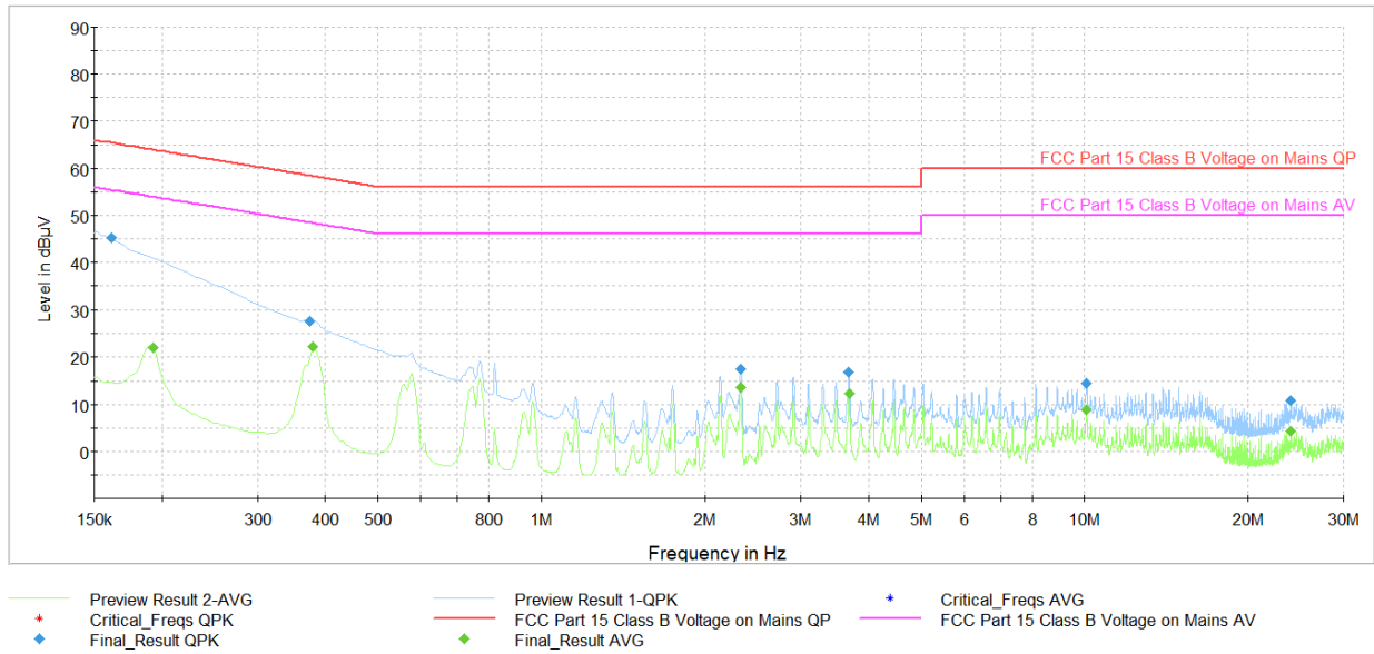
Plot 7-25. AC Line Conducted Plot (LE2M – 5731MHz) (L1) with host PC and USB-C Cable
