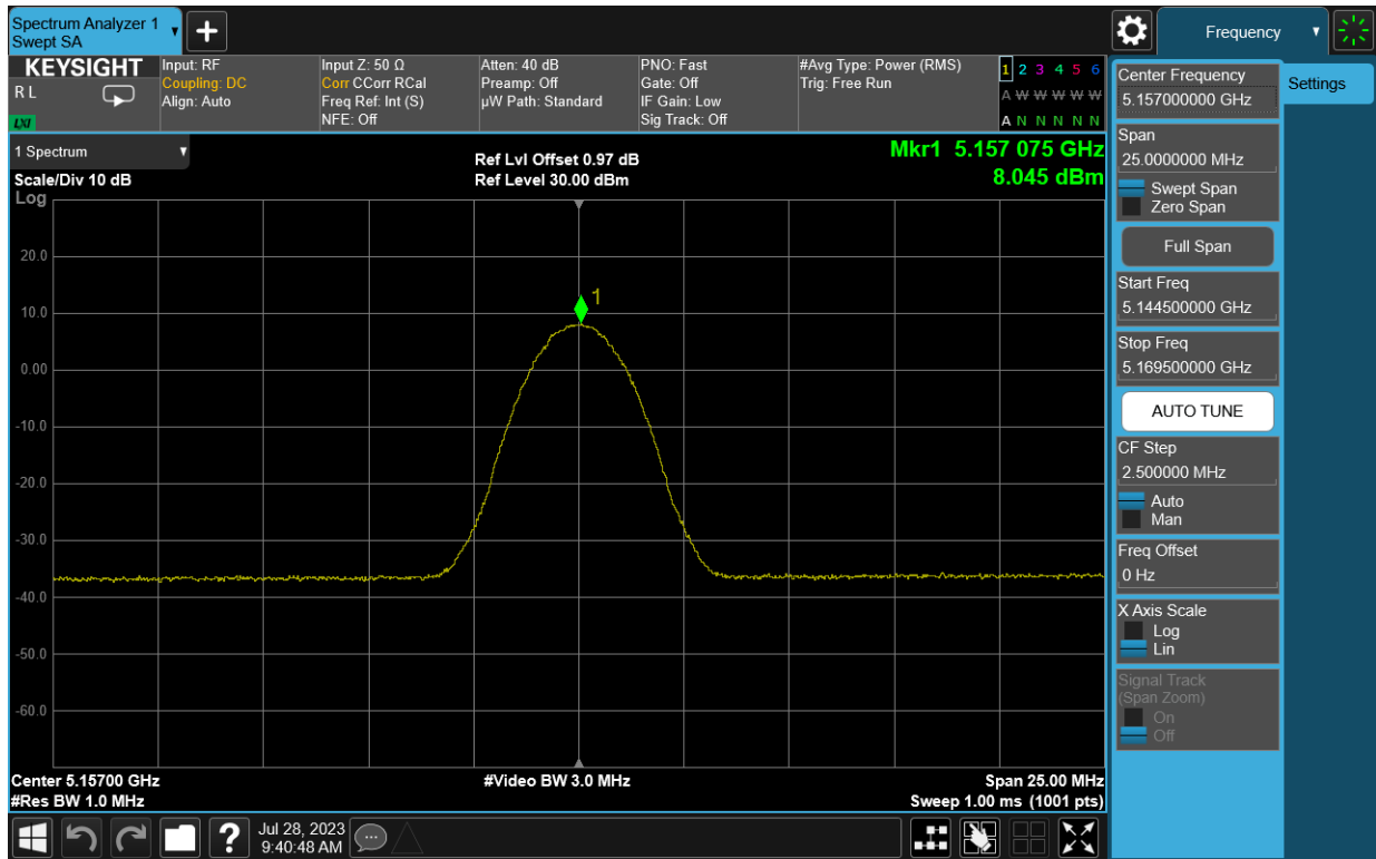
Plot 7-7. PSD (LE2M, 5157MHz)
