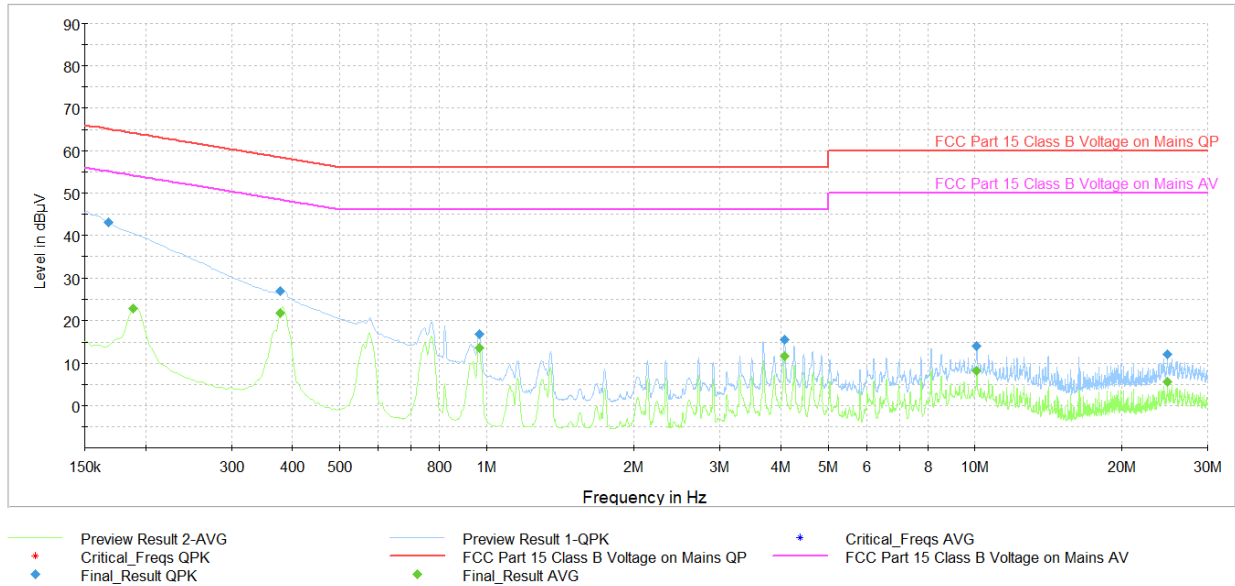
Plot 7-26. AC Line Conducted Plot (LE2M – 5731MHz) (N) with host PC and USB-C Cable
