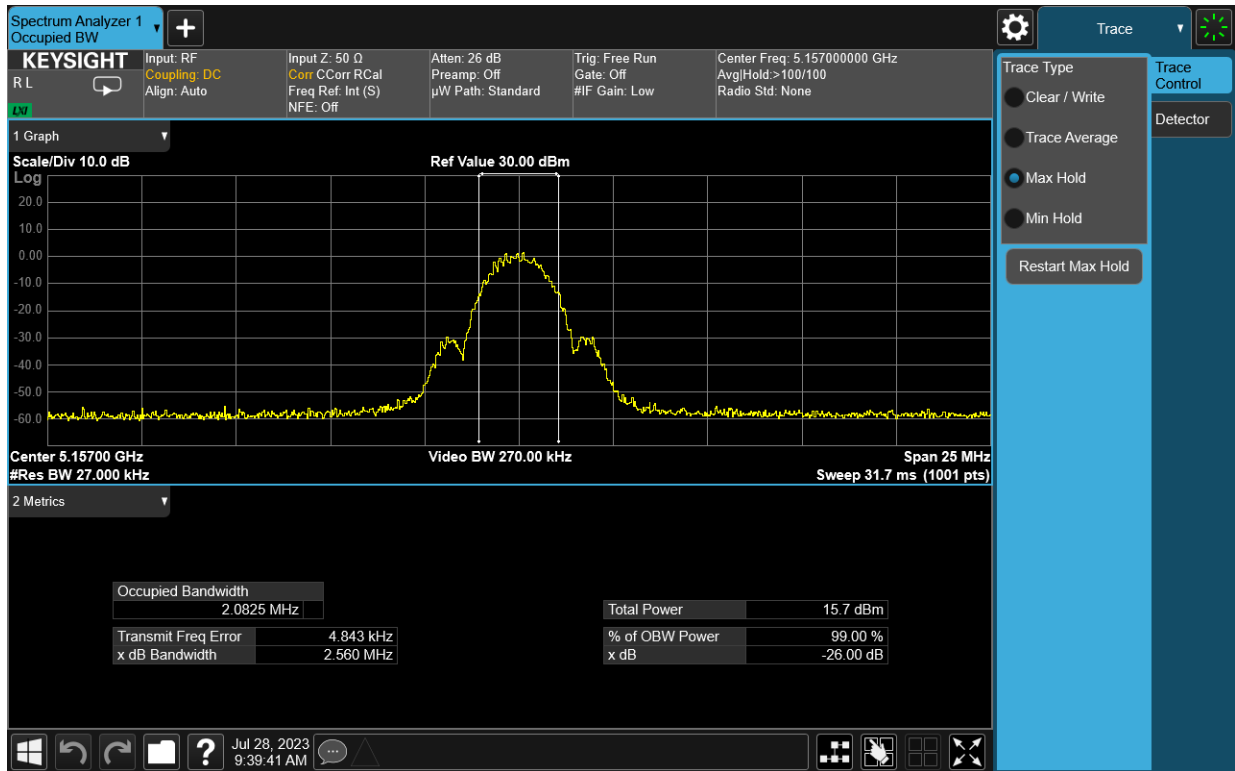
Plot 7-1. 26dB BW & 99% OBW (LE2M, 5157MHz)
