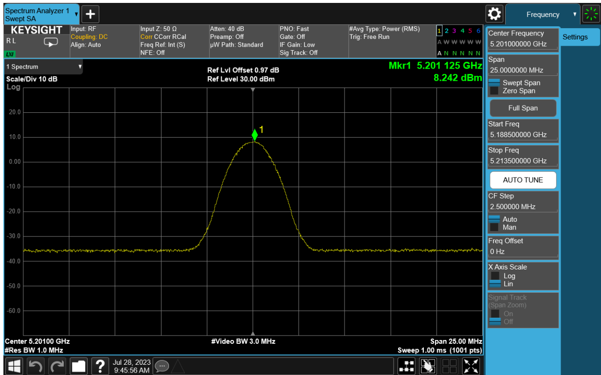
Plot 7-8. PSD (LE2M, 5201MHz)
