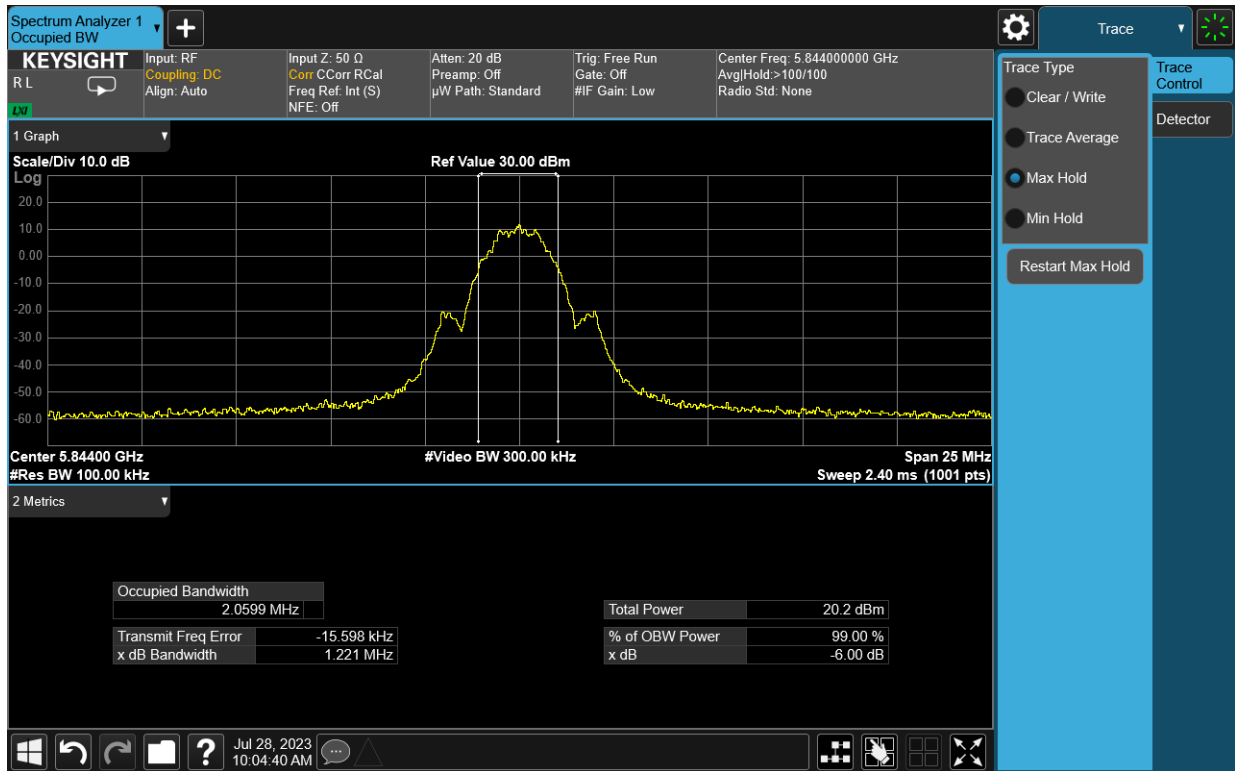
Plot 7-6. 6dB BW & 99% OBW (LE2M, 5844MHz)
