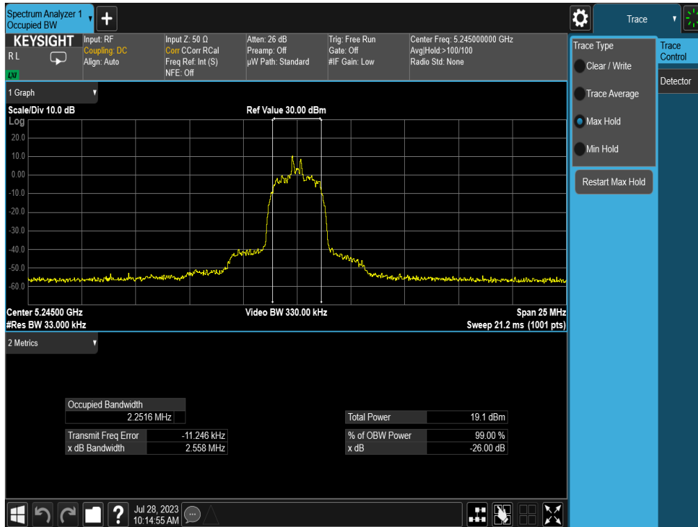
Plot 7-3. 26dB BW & 99% OBW (HDR4, 5245MHz)
