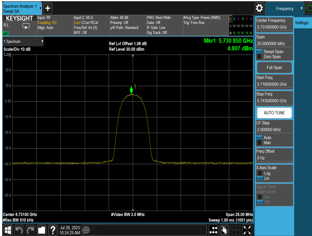
Plot 7-37. PSD (HDR4 – 5731MHz)
