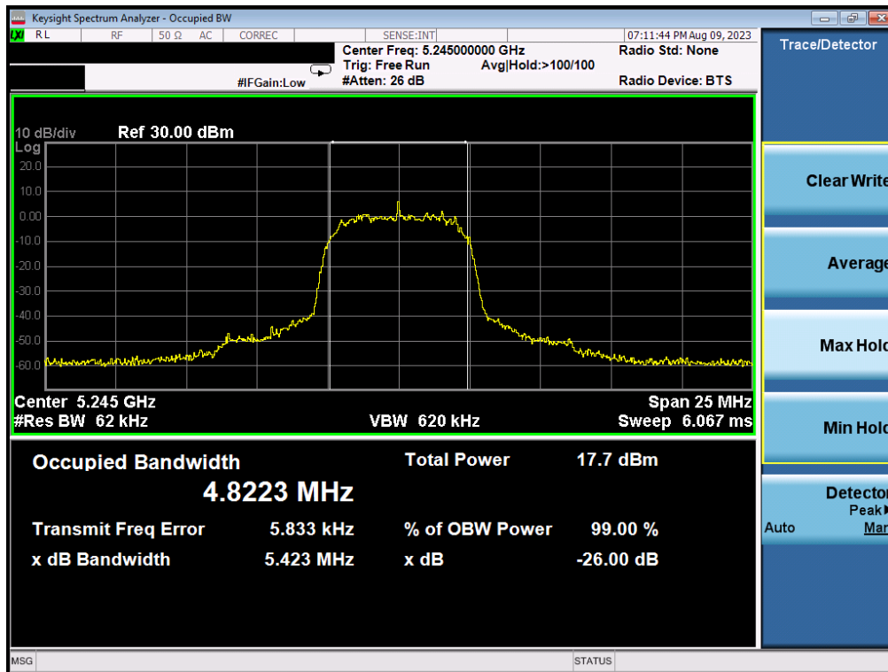
Plot 7-12. 26dB BW & 99% OBW (HDRp8, 5245MHz)
