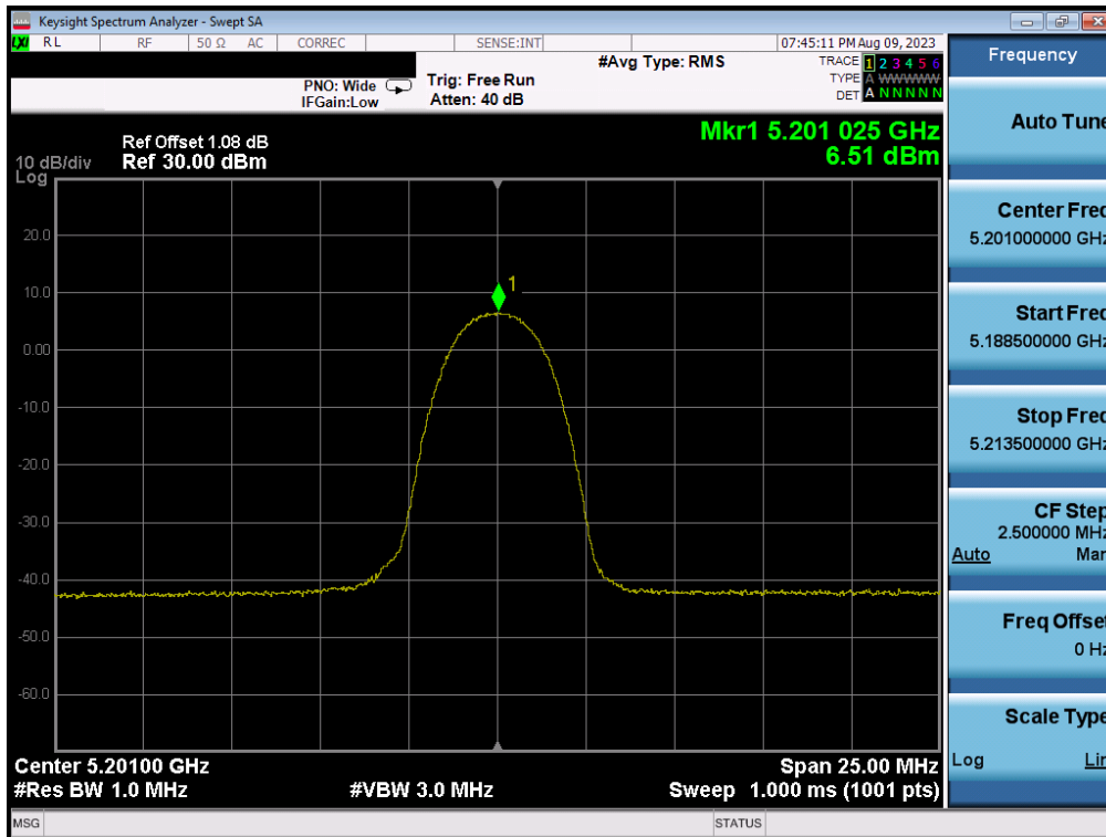
Plot 7-26. PSD (HDR4 – 5201MHz)
