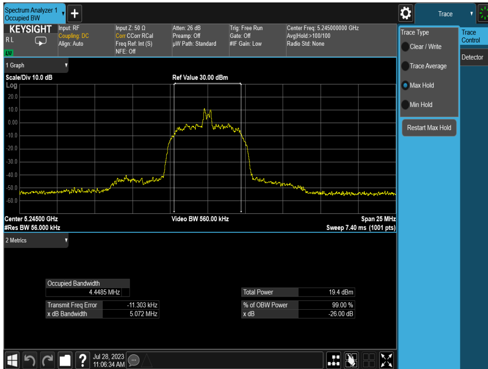
Plot 7-6. 26dB BW & 99% OBW (HDR8, 5245MHz)
