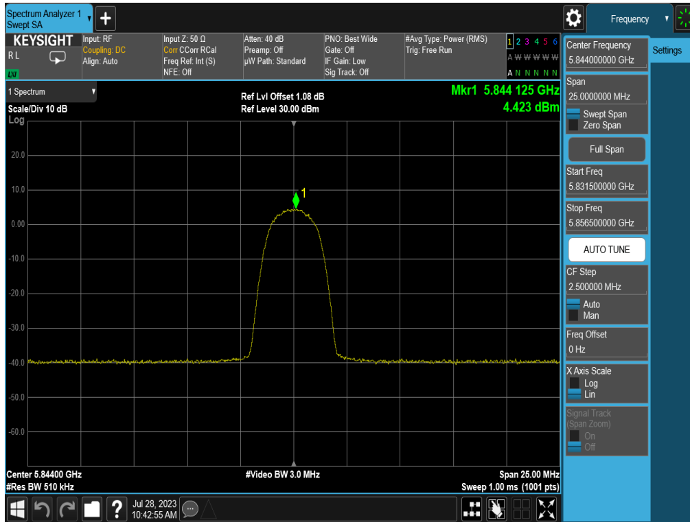
Plot 7-39. PSD (HDR4 – 5844MHz)
