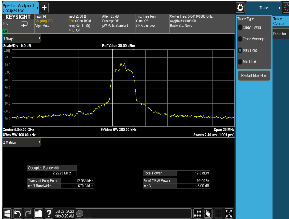
Plot 7-15. 6dB BW & 99% OBW (HDR4, 5844MHz)
