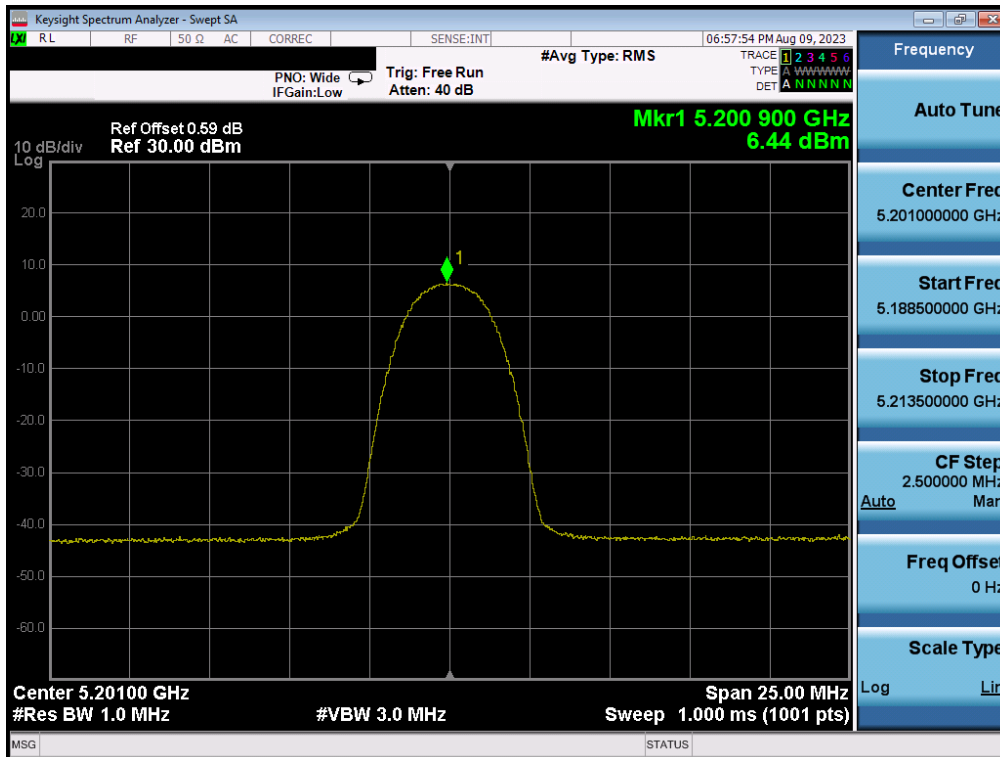
Plot 7-32. PSD (HDRp4 – 5201MHz)
