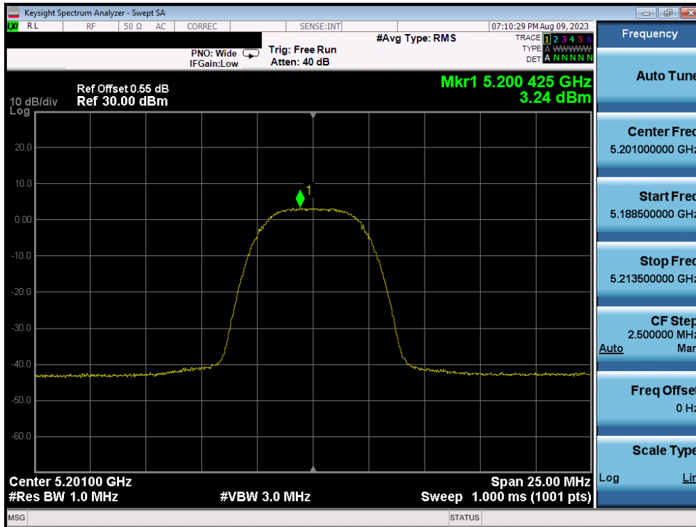
Plot 7-35. PSD (HDRp8 – 5201MHz)
