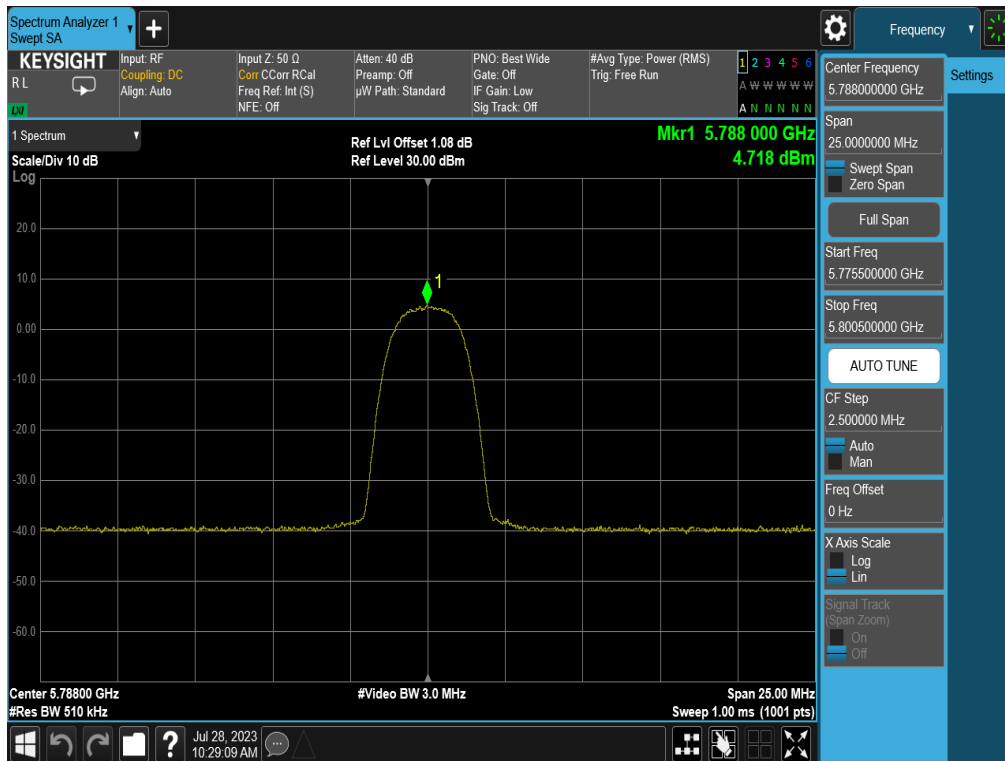
Plot 7-38. PSD (HDR4 – 5788MHz)
