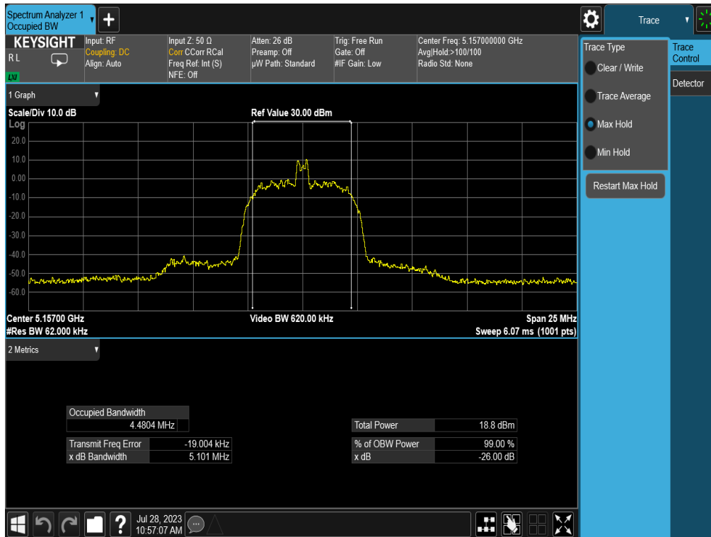
Plot 7-4. 26dB BW & 99% OBW (HDR8, 5157MHz)
