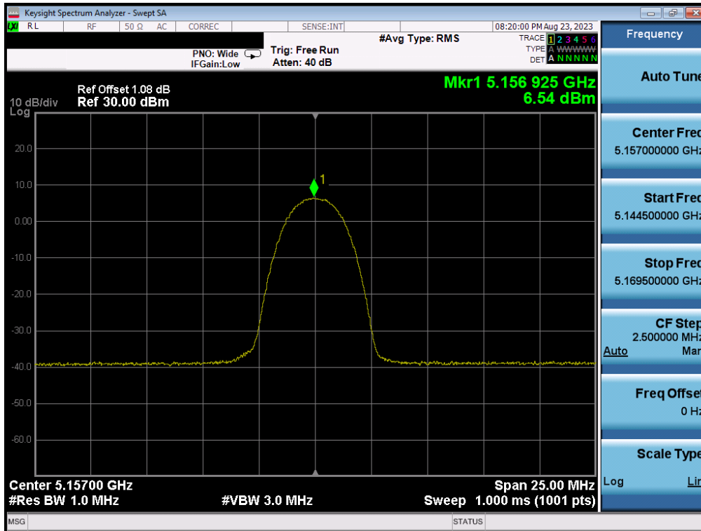
Plot 7-25. PSD (HDR4 – 5157MHz)
