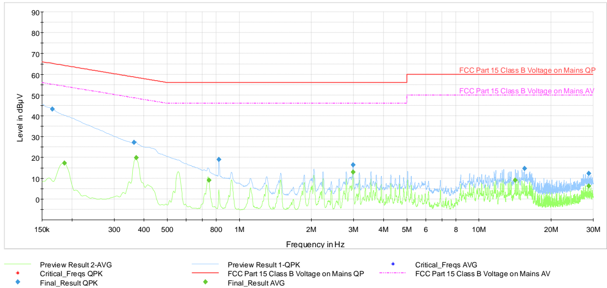
Plot 7-70. AC Line Conducted Plot (HDR4 – 5201MHz) (L1) with host PC and USB-C Cable
