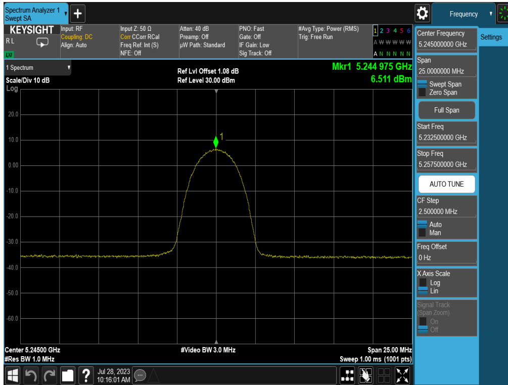
Plot 7-27. PSD (HDR4 – 5245MHz)
