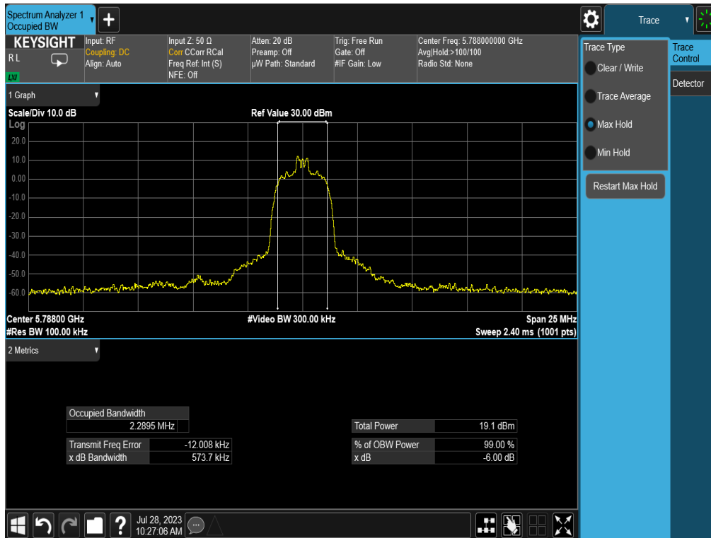
Plot 7-14. 6dB BW & 99% OBW (HDR4, 5788MHz)
