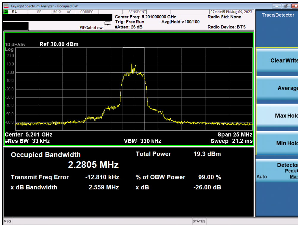
Plot 7-2. 26dB BW & 99% OBW (HDR4, 5201MHz)
