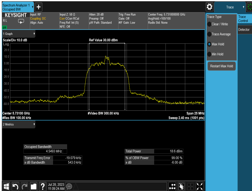
Plot 7-16. 6dB BW & 99% OBW (HDR8, 5731MHz)
