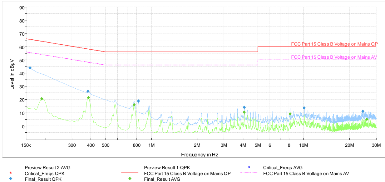
Plot 7-71. AC Line Conducted Plot (HDR4 – 5201MHz) (N) with host PC and USB-C Cable
