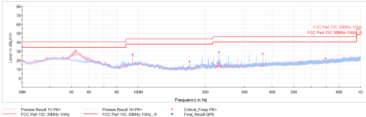
Plot 7-69. Radiated Spurious Emissions 30MHz - 1GHz (HDR4 – 5201MHz), with AC/DC Adapter and USB-C Cable
