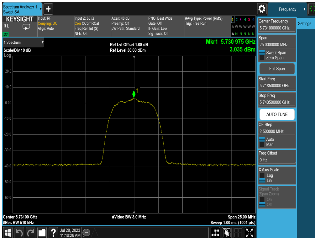
Plot 7-40. PSD (HDR8 – 5731MHz)
