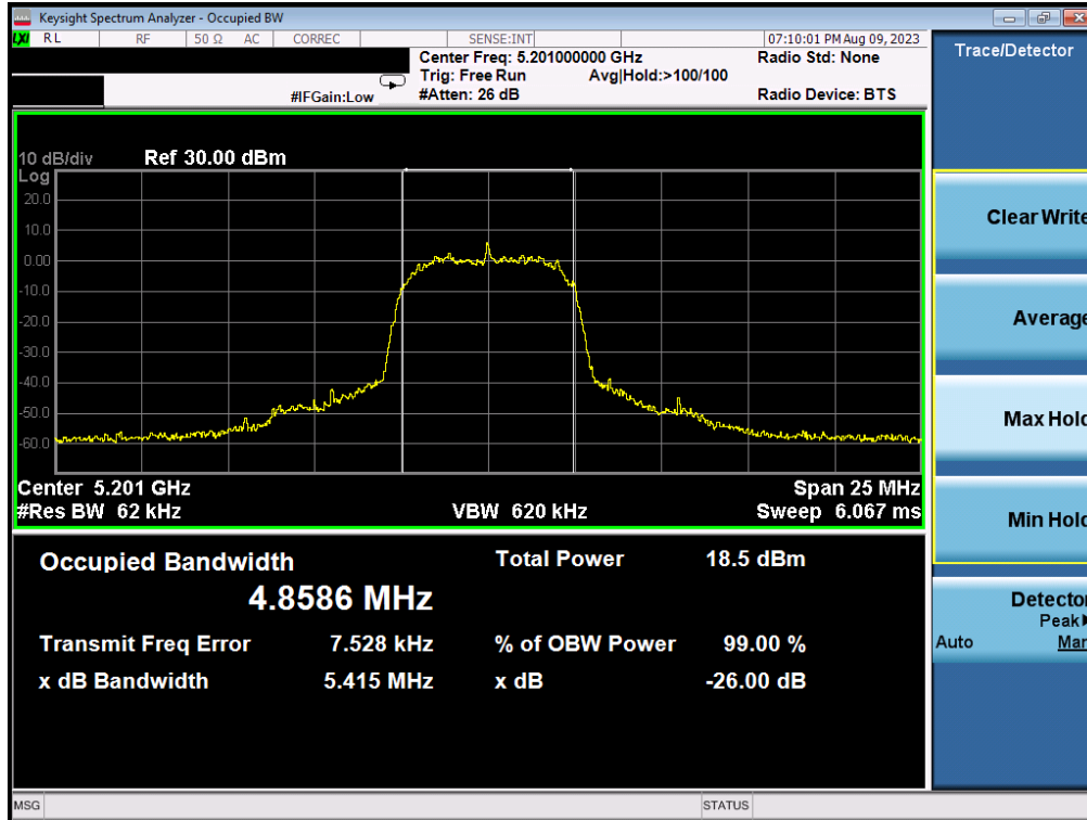
Plot 7-11 26dB BW & 99% OBW (HDRp8, 5201MHz)
