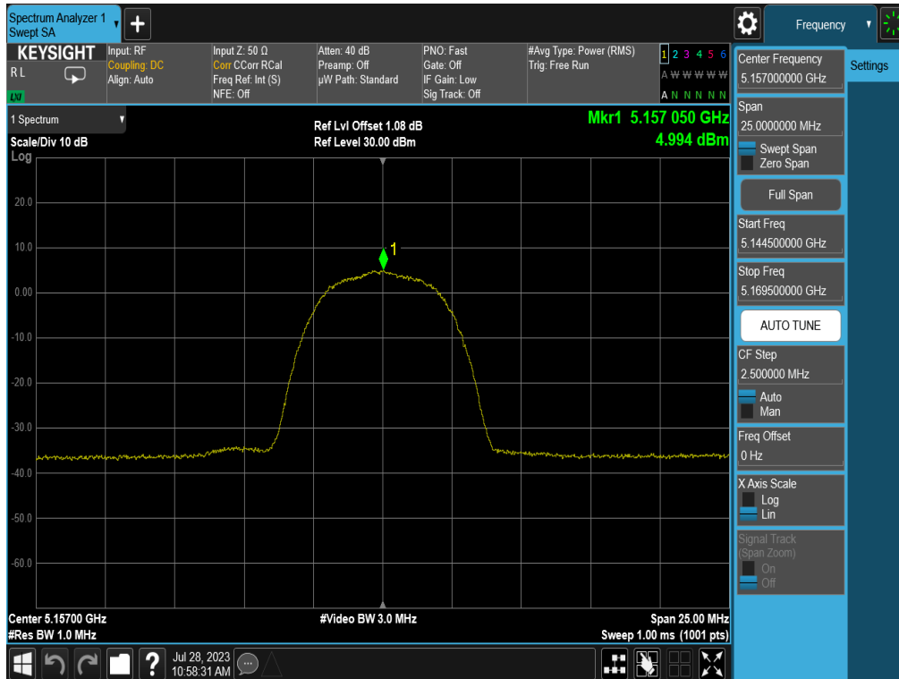
Plot 7-28. PSD (HDR8 – 5157MHz)
