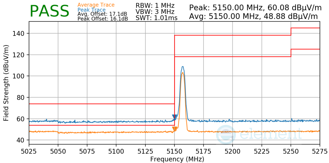
Plot 7-57. Radiated Lower Band Edge Measurement
