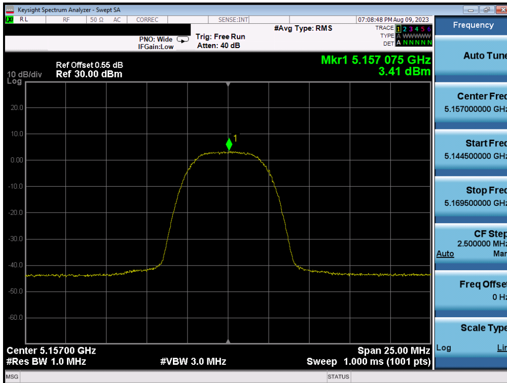
Plot 7-34. PSD (HDRp8 – 5157MHz)
