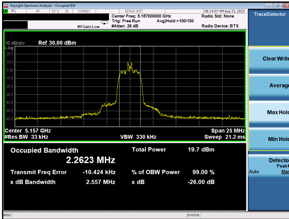
Plot 7-1. 26dB BW & 99% OBW (HDR4, 5157MHz)
