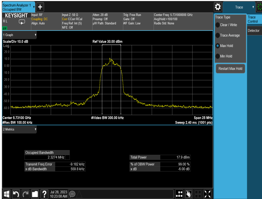
Plot 7-13. 6dB BW & 99% OBW (HDR4, 5731MHz)
