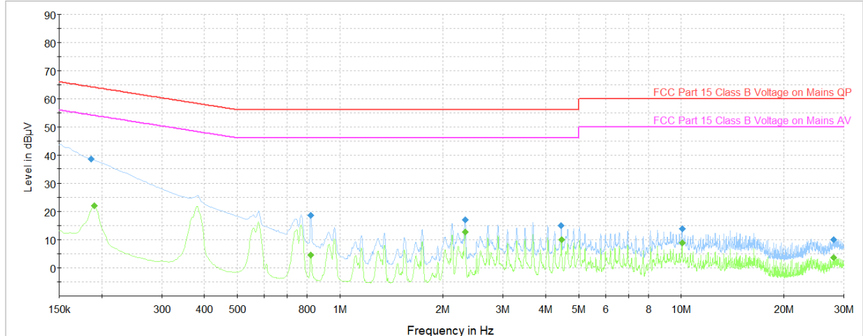
Plot 7-25. AC Line Conducted Plot (BDR – 5157MHz) (L1) with host PC and USB-C cable
