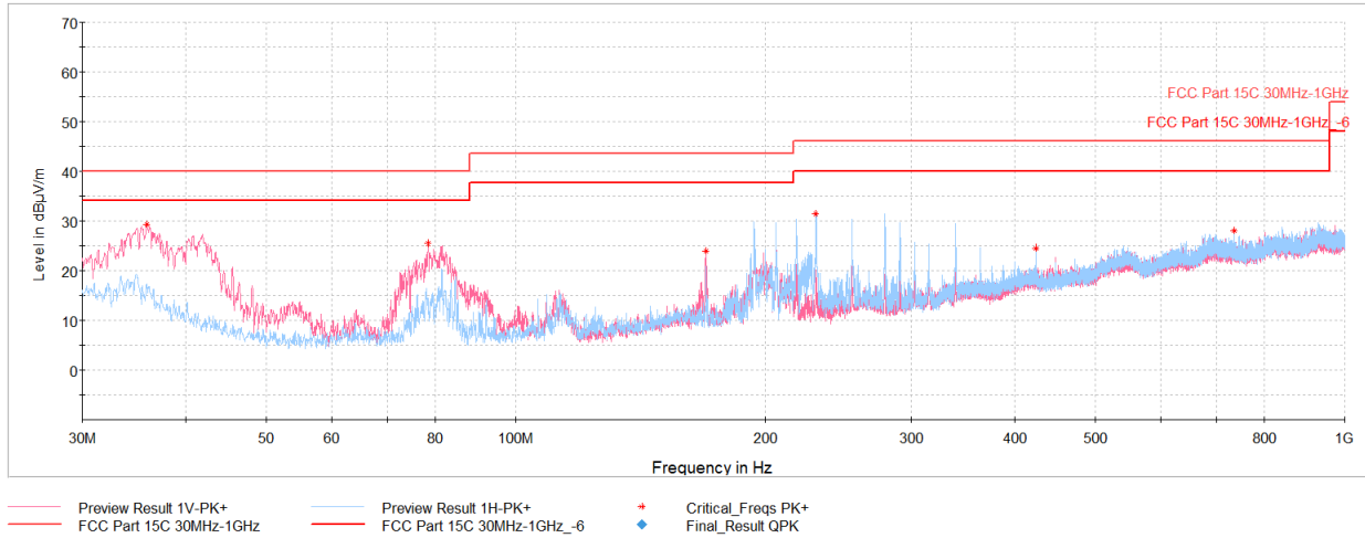
Plot 7-24. RSE 30MHz - 1GHz (BDR – 5157MHz), with AC/DC Adapter and USB-C Cable
