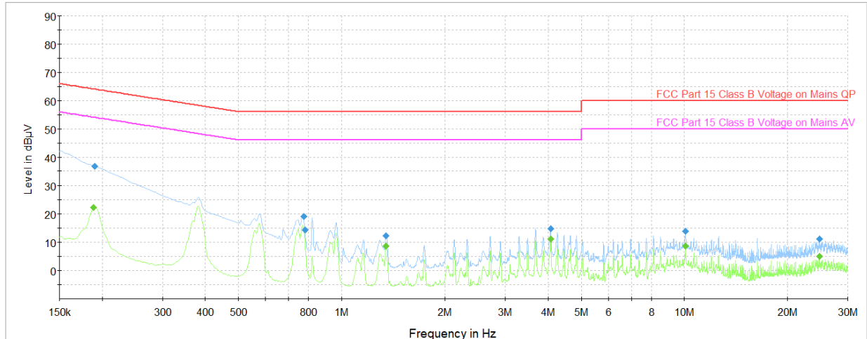
Plot 7-26. AC Line Conducted Plot (BDR – 5157MHz) (N) with host PC and USB-C cable
