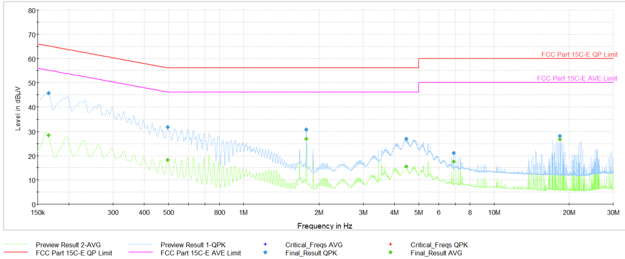
Plot 7-44. AC Line Conducted Plot (Ch. 9, Config 409, Payload 4093 N, with AC/DC Adapter + Magnetic Charger)
