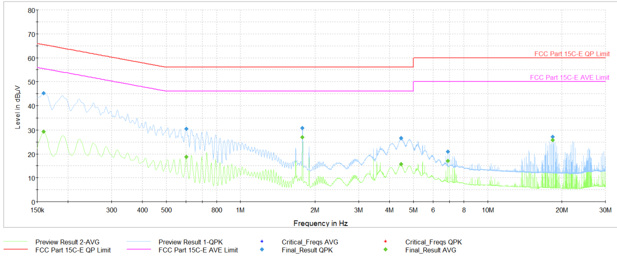
Plot 7-42. AC Line Conducted (Ch. 5, Config 409, Payload 4093 N, with AC/DC Adapter + Magnetic Charger)
