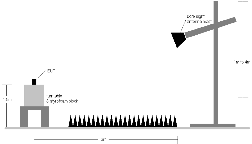
Figure 7-1. Test Setup
