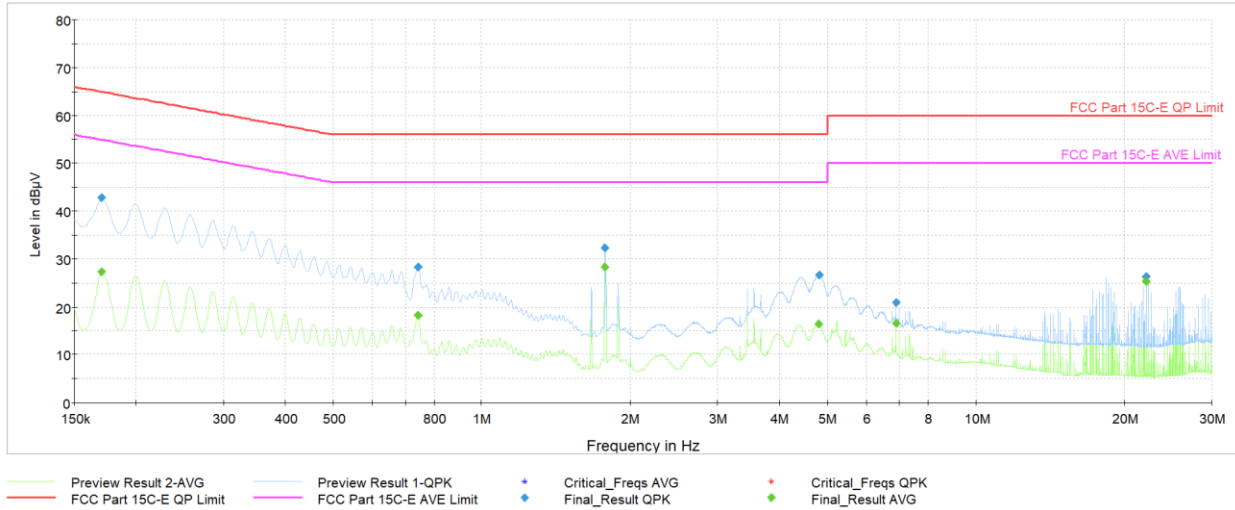
Plot 7-41. AC Line Conducted (Ch. 5, Config 409, Payload 4093 L1, with AC/DC Adapter + Magnetic Charger)
