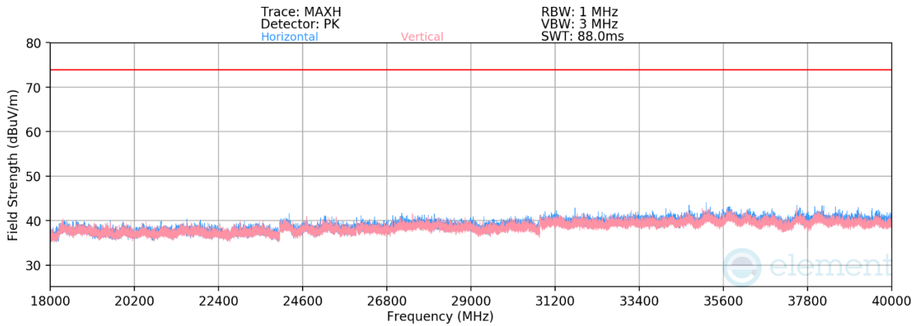
Plot 7-34. Radiated Emissions 18GHz-40GHz (802.11n – Ch. 64)
