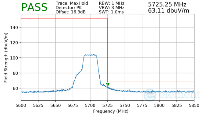
Plot 7-52. (Pk, Ch.140, 802.11n, MCS7)
