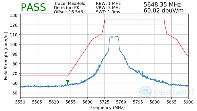
Plot 7-54. (Pk, Ch.149, 802.11n, MCS7)
