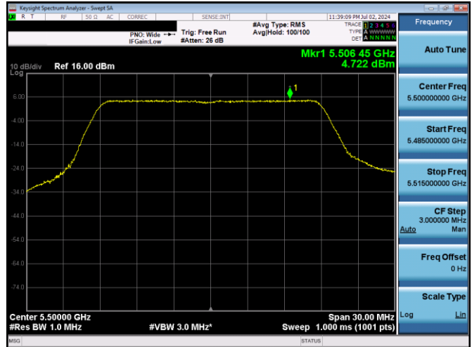
Plot 7-22. PSD (20MHz BW 802.11n - Ch. 100, MCS0)
