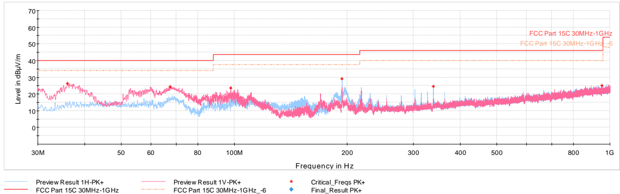
Plot 7-57. Radiated Spurious Emissions below 1GHz, 802.11n, Ch. 64 with AC/DC Adapter & magnetic charger
