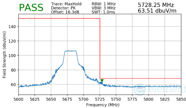
Plot 7-50. (Pk, Ch.136, 802.11n, MCS7)
