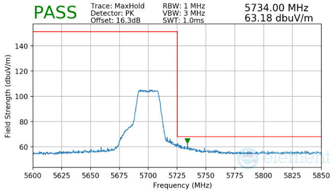
Plot 7-51. (Pk, Ch.140, 802.11n, MCS0)
