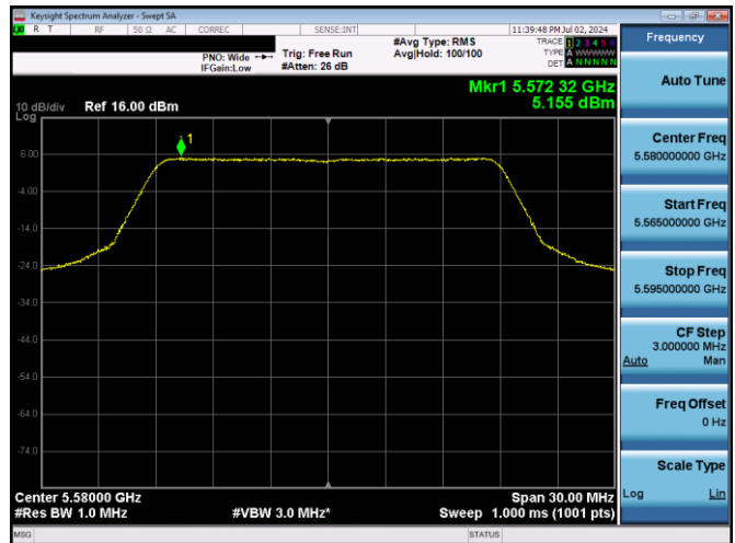
Plot 7-23. PSD (20MHz BW 802.11n - Ch. 116, MCS0)
