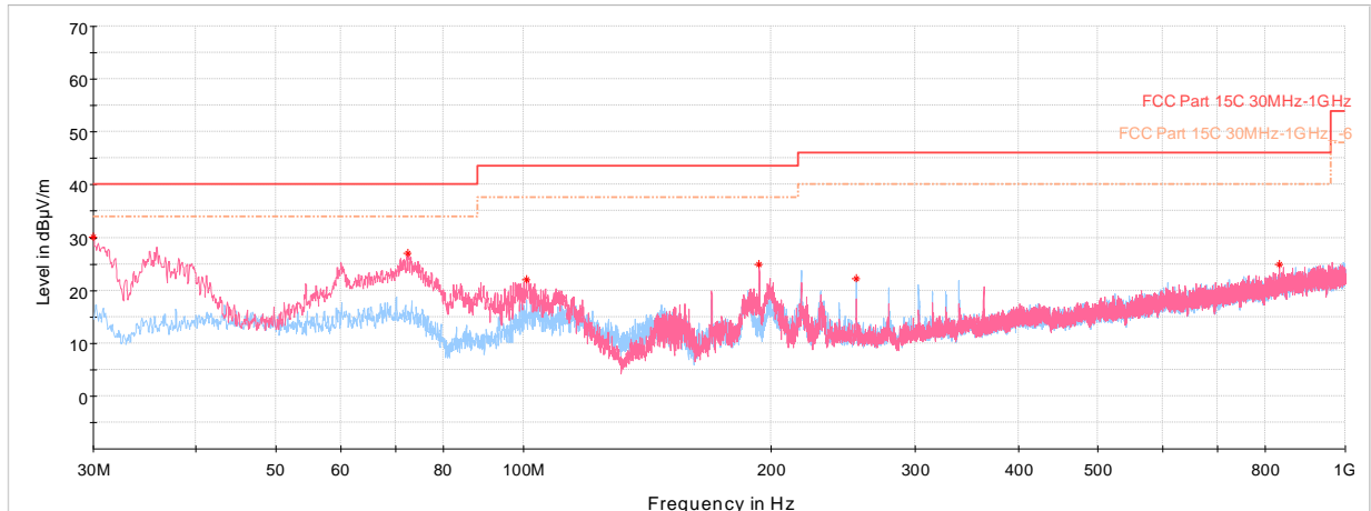
Plot 7-58. Radiated Spurious Emissions – Simultaneous Transmission 30MHz – 1GHz, with AC/DC Adapter & magnetic charger)
