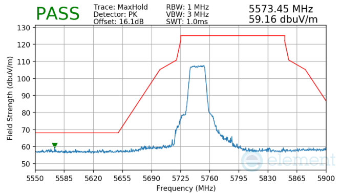
Plot 7-53. (Pk, Ch.149, 802.11n, MCS0)
