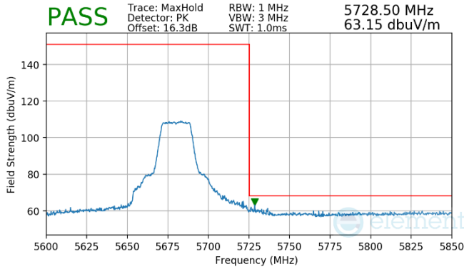
Plot 7-49. (Pk, Ch.136, 802.11n, MCS0)
