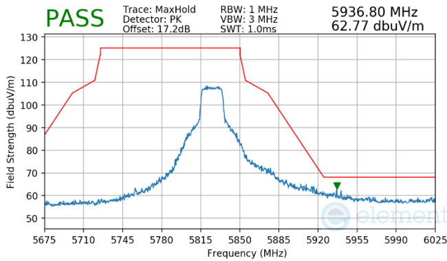
Plot 7-56. (Pk, Ch.165, 802.11n, MCS7)
