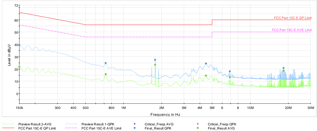
Plot 7-59. AC Line Conducted Plot with 802.11n Ch.64 (L1), with AC/DC adapter & magnetic charger
