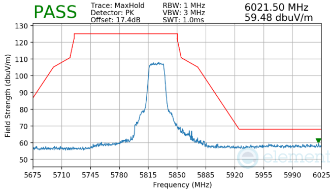
Plot 7-55. (Pk, Ch.165, 802.11n, MCS0)
