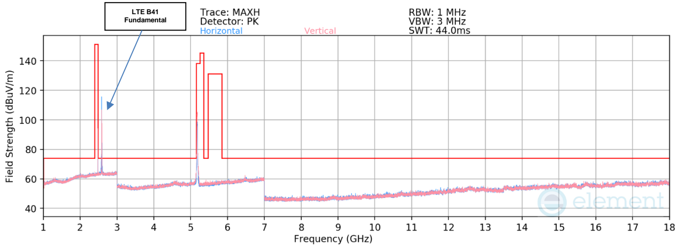
Plot 7-41. Radiated Spurious Emissions – Simultaneous Transmission Configuration 1GHz-18GHz
