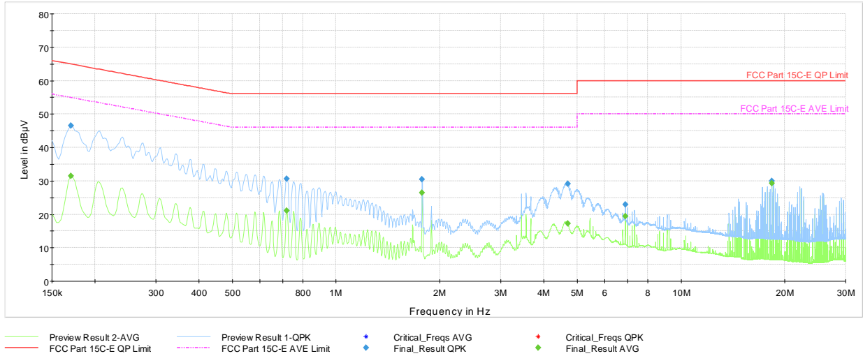
Plot 7-60. AC Line Conducted Plot with 802.11n Ch.64 (N), with AC/DC adapter & magnetic charger
