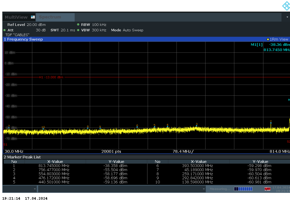
Plot 7-13. Conducted Spurious Plot (LTE Band 26 - 5MHz QPSK - RB Size 1, RB Offset 0 - Low Channel)
