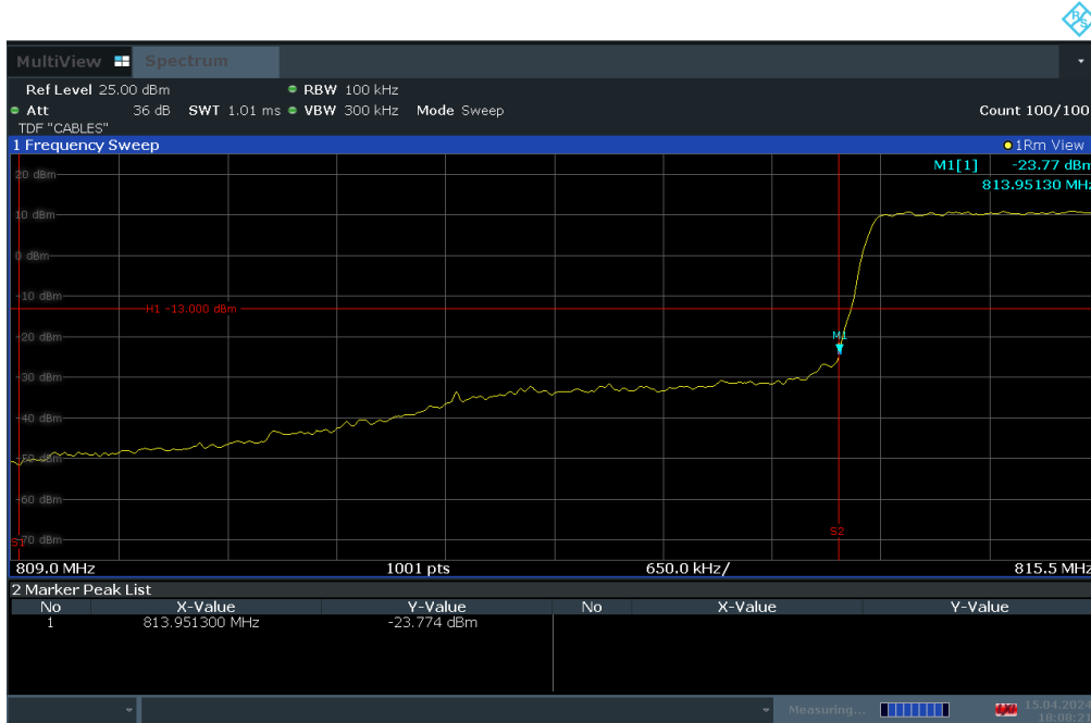
Plot 7-33. Channel Edge Plot (LTE Band 26 - 3MHz QPSK – Low Channel)
