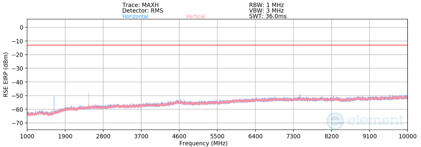
Plot 7-48. Antenna BCM Radiated Spurious Plot Above 1GHz (LTE Band 26)
