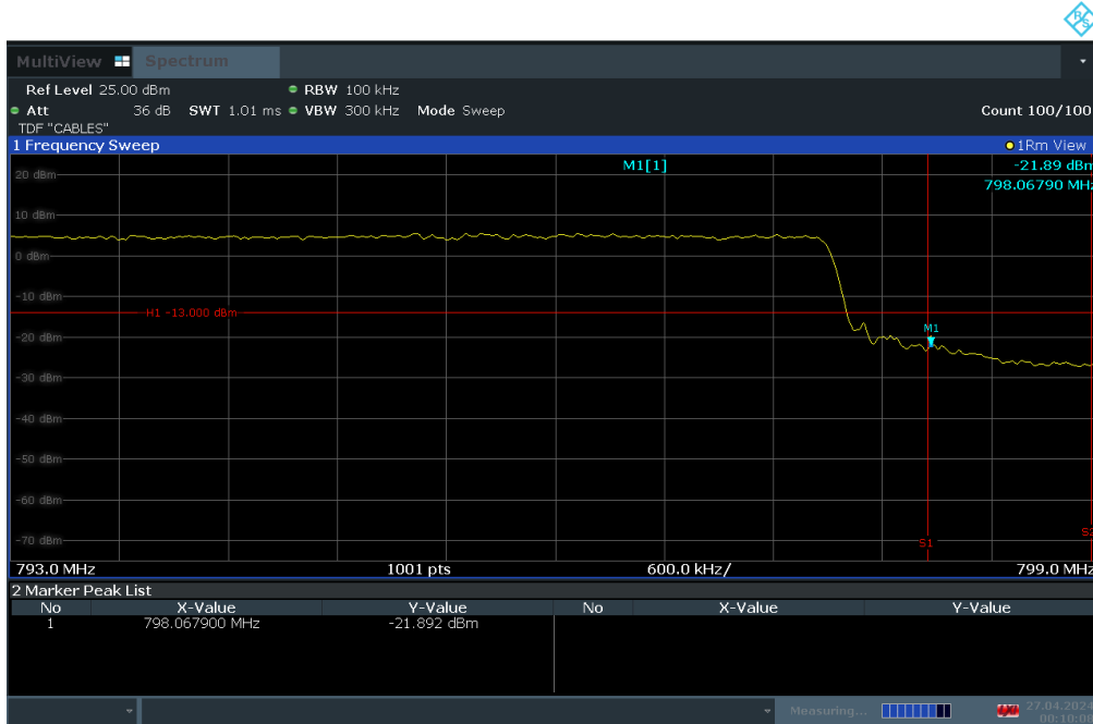
Plot 7-45. Upper Band Edge Plot (LTE Band 14 - 10MHz QPSK – RB Size 50)
