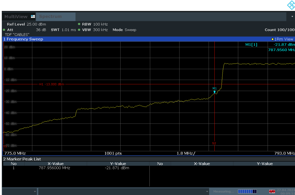
Plot 7-43. Lower Band Edge Plot (LTE Band 14 - 10MHz QPSK – RB Size 50)
