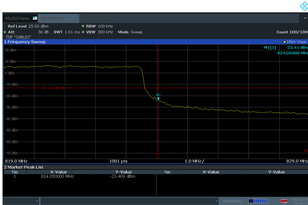
Plot 7-38. Channel Edge Plot (LTE Band 26 - 10MHz QPSK – High Channel)
