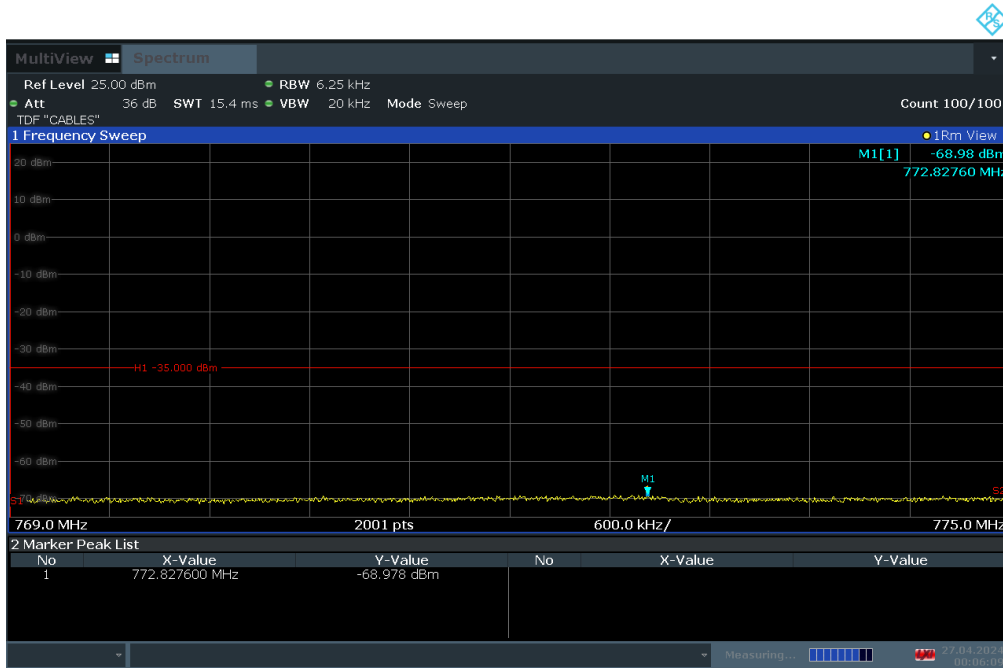
Plot 7-40. Lower Emission Mask Plot (LTE Band 14 - 5MHz QPSK – RB Size 25)
