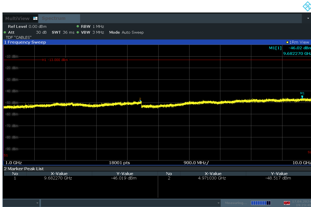
Plot 7-18. Conducted Spurious Plot (LTE Band 26 - 10MHz QPSK - RB Size 1, RB Offset 0 - Mid Channel)
