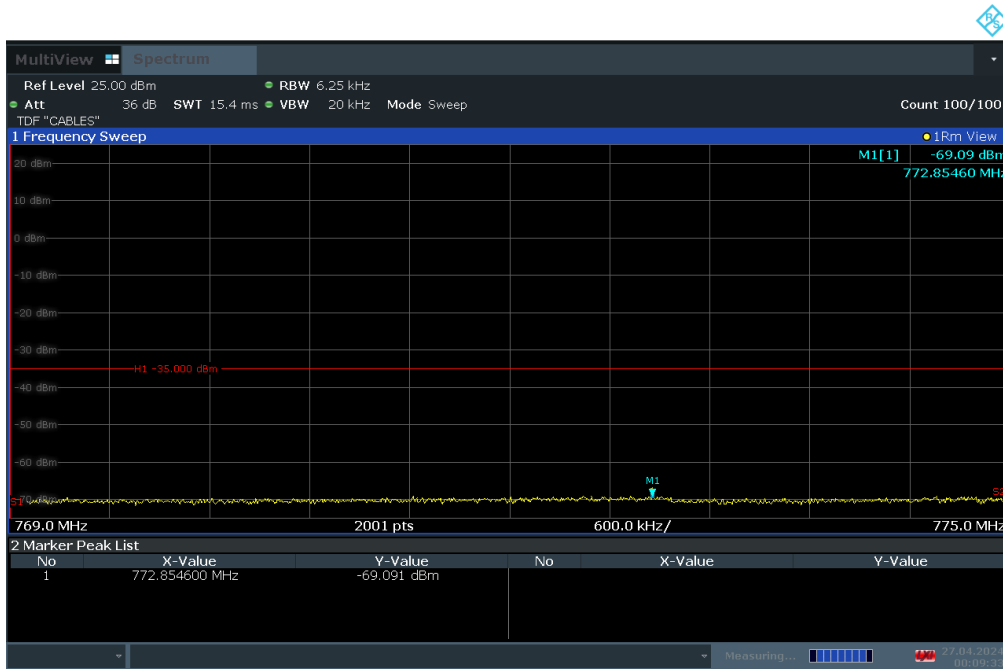
Plot 7-44. Lower Emission Mask Plot (LTE Band 14 - 10MHz QPSK – RB Size 50)
