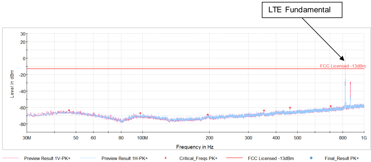
Plot 7-47. Antenna BCM Radiated Spurious Plot Below 1GHz (LTE Band 26)
