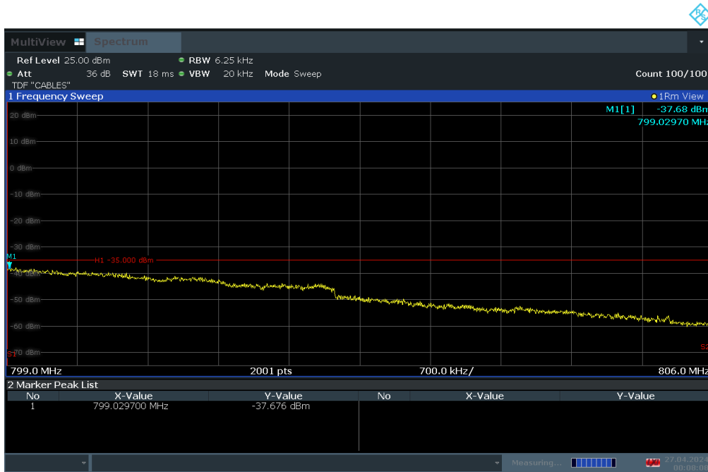
Plot 7-42. Upper Emission Mask Plot (LTE Band 14 - 5MHz QPSK – RB Size 25)
