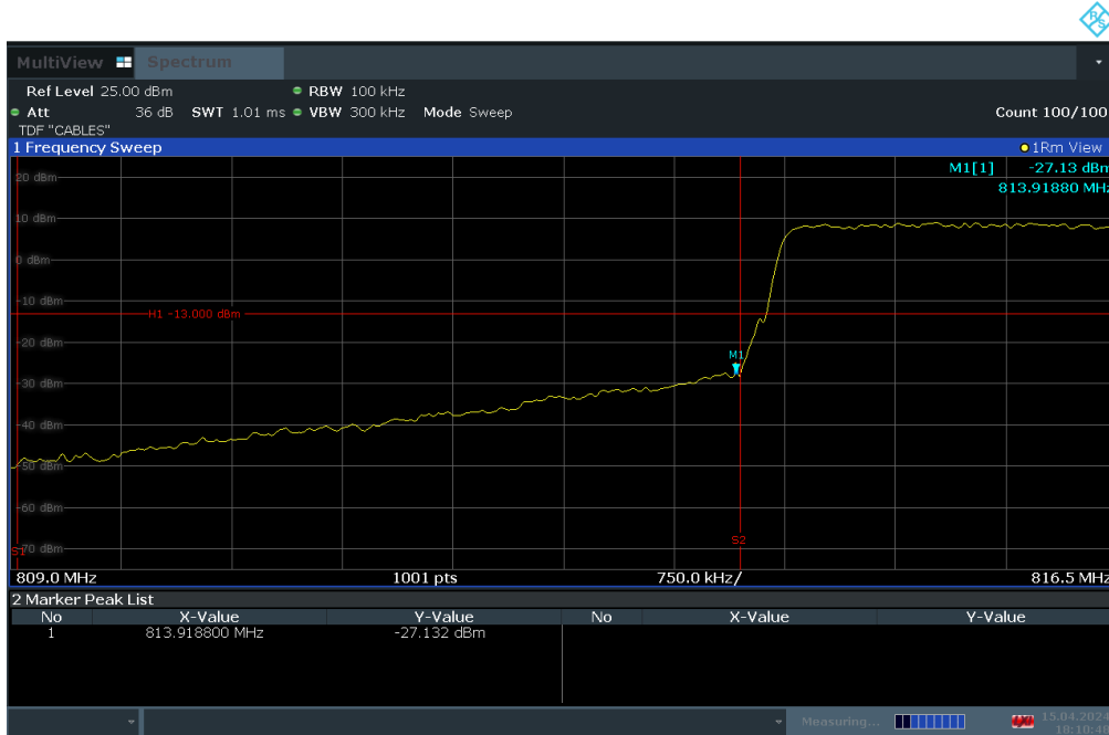
Plot 7-35. Channel Edge Plot (LTE Band 26 - 5MHz QPSK – Low Channel)
