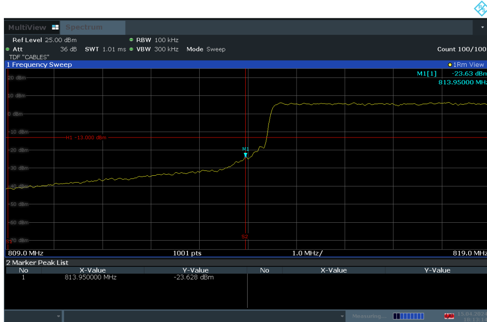
Plot 7-37. Channel Edge Plot (LTE Band 26 - 10MHz QPSK – Low Channel)
