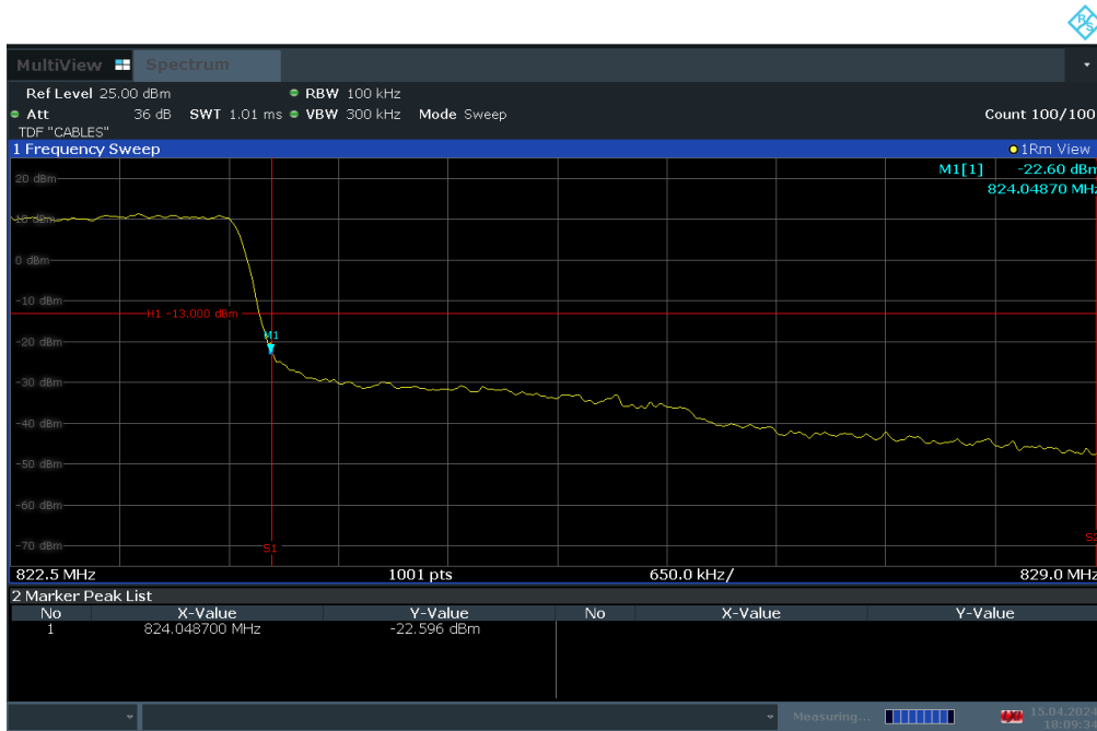
Plot 7-34. Channel Edge Plot (LTE Band 26 - 3MHz QPSK – High Channel)
