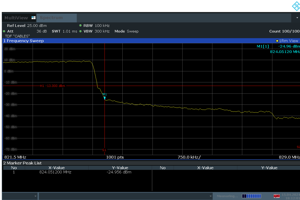
Plot 7-36. Channel Edge Plot (LTE Band 26 - 5MHz QPSK – High Channel)
