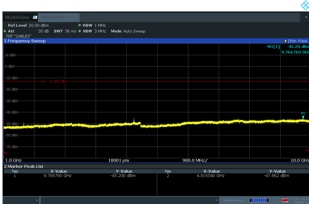
Plot 7-30. Conducted Spurious Plot (LTE Band 14 - 5MHz QPSK - RB Size 1, RB Offset 0 - High Channel)
