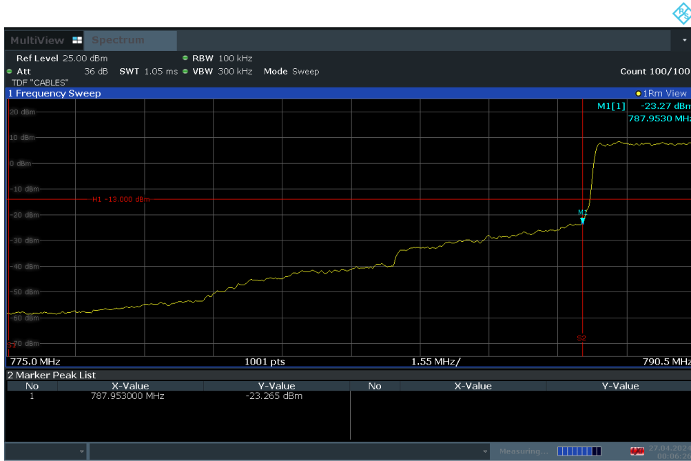
Plot 7-39. Lower Band Edge Plot (LTE Band 14 - 5MHz QPSK – RB Size 25)
