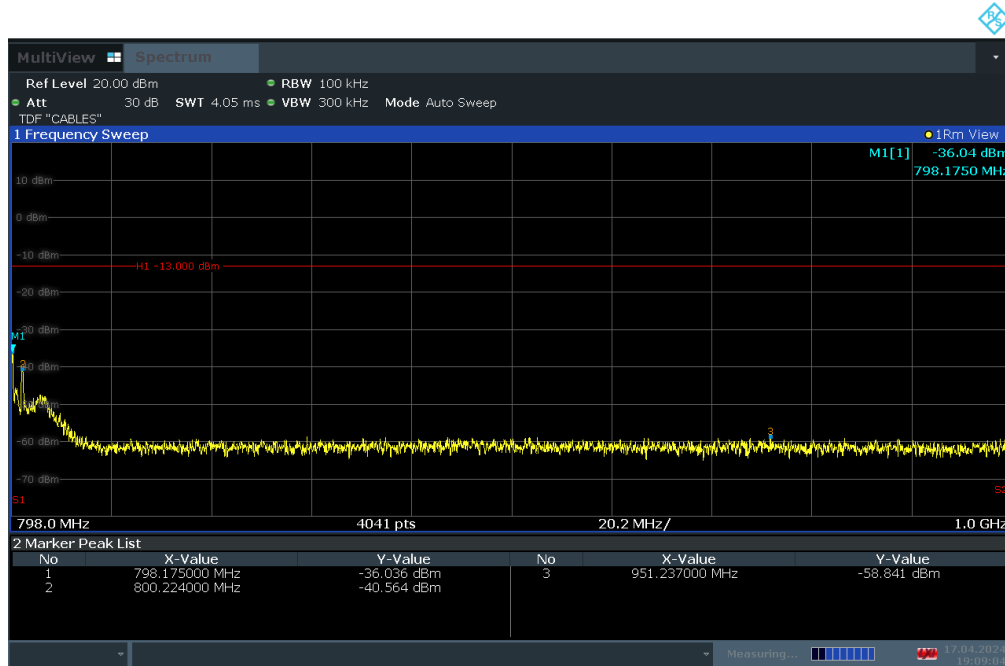
Plot 7-28. Conducted Spurious Plot (LTE Band 14 - 5MHz QPSK - RB Size 1, RB Offset 0 - High Channel)
