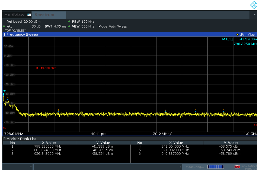
Plot 7-26. Conducted Spurious Plot (LTE Band 14 - 10MHz QPSK - RB Size 1, RB Offset 0 - Mid Channel)
