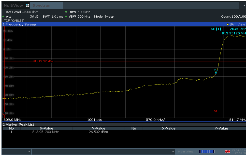
Plot 7-31. Channel Edge Plot (LTE Band 26 – 1.4MHz QPSK – Low Channel)
