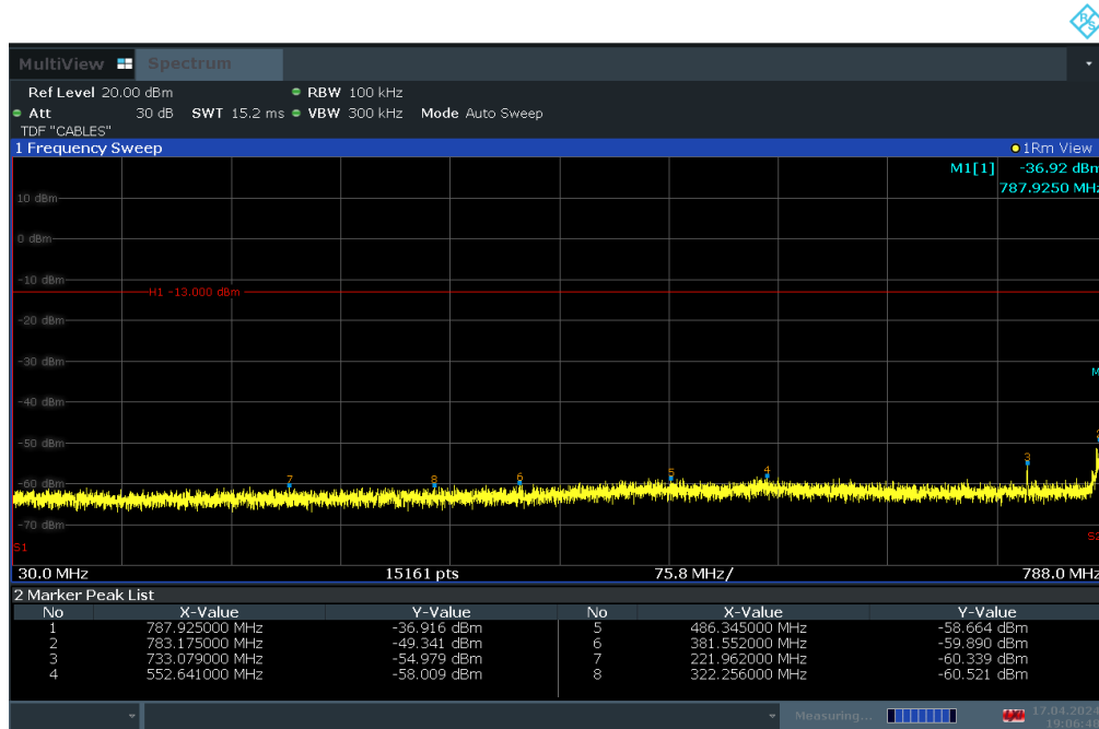
Plot 7-25. Conducted Spurious Plot (LTE Band 14 - 10MHz QPSK - RB Size 1, RB Offset 0 - Mid Channel)
