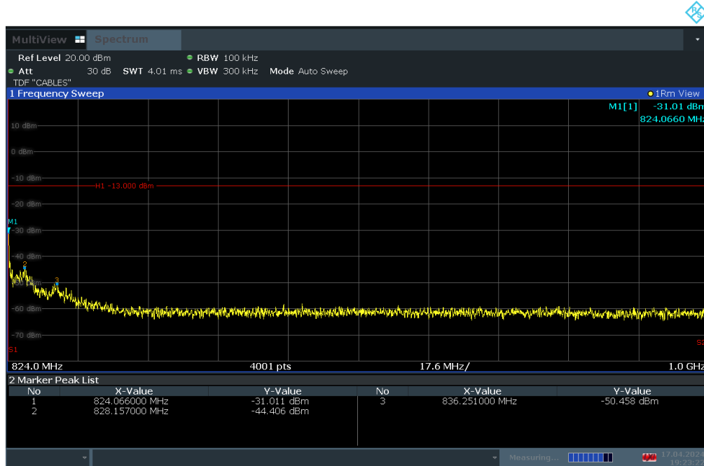
Plot 7-17. Conducted Spurious Plot (LTE Band 26 - 10MHz QPSK - RB Size 1, RB Offset 0 - Mid Channel)
