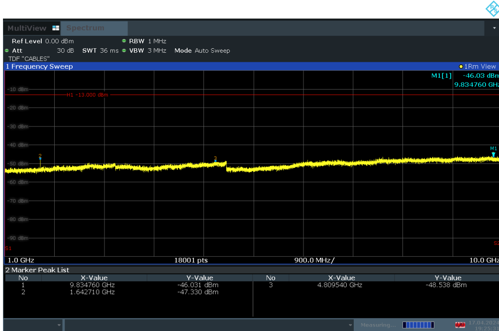
Plot 7-21. Conducted Spurious Plot (LTE Band 26 - 5MHz QPSK - RB Size 1, RB Offset 0 - High Channel)
