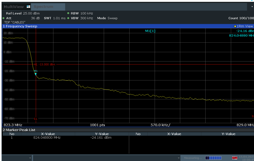
Plot 7-32. Channel Edge Plot (LTE Band 26 – 1.4MHz QPSK – High Channel)
