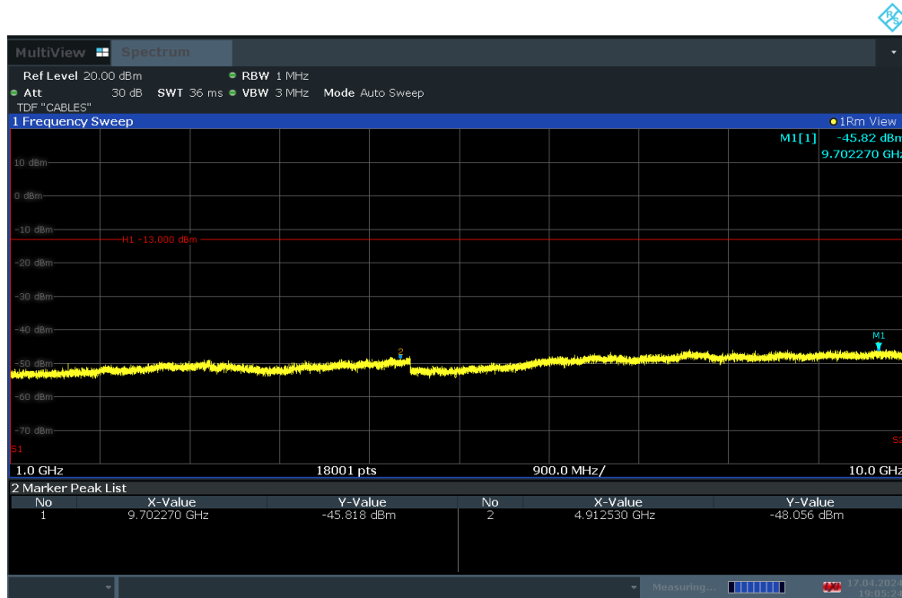
Plot 7-24. Conducted Spurious Plot (LTE Band 14 - 5MHz QPSK - RB Size 1, RB Offset 0 - Low Channel)
