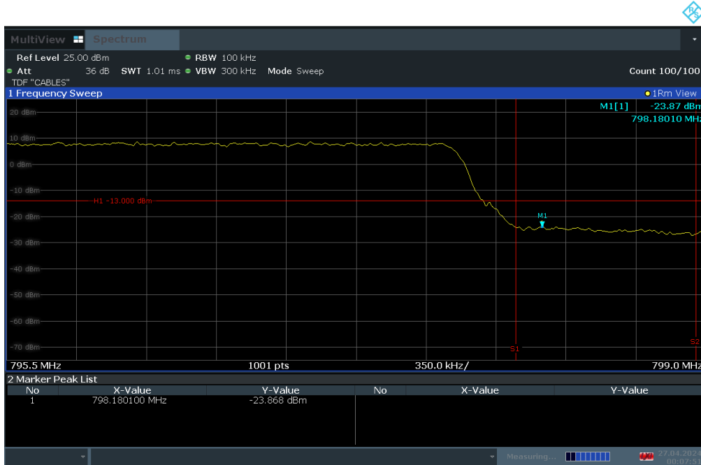
Plot 7-41. Upper Band Edge Plot (LTE Band 14 - 5MHz QPSK – RB Size 25)
