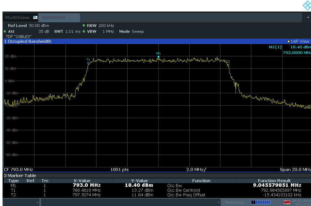
Plot 7-11. Occupied Bandwidth Plot (LTE Band 14 - 10MHz QPSK - Full RB)
