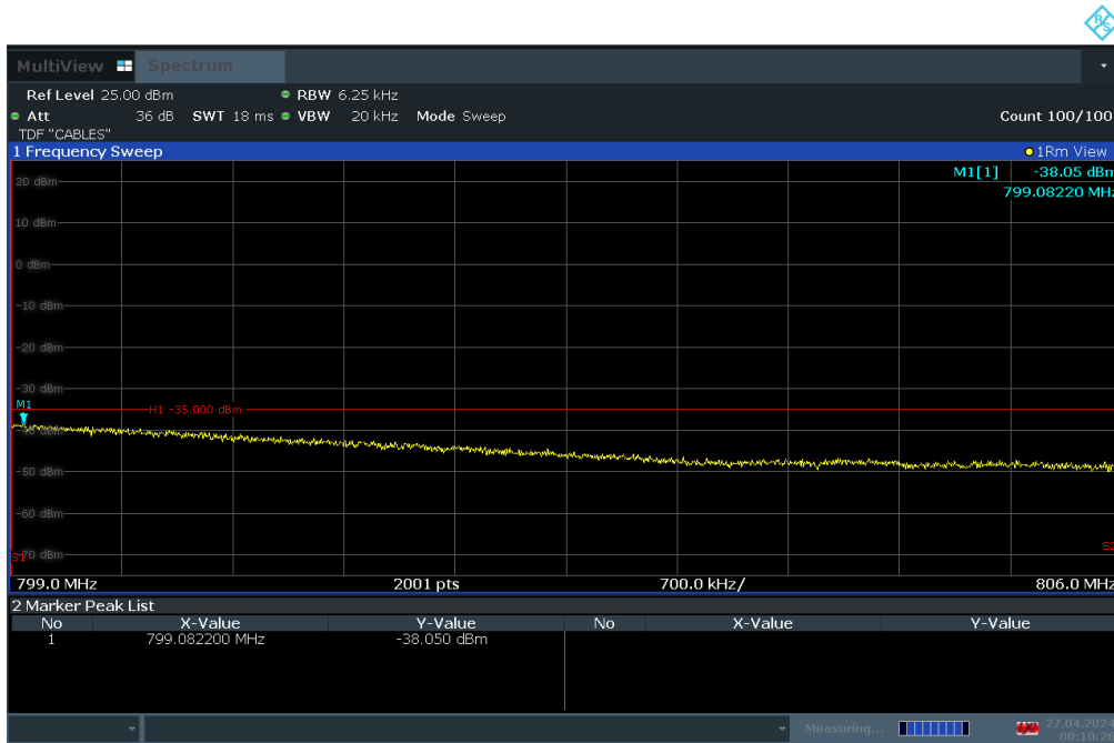
Plot 7-46. Upper Emission Mask Plot (LTE Band 14 - 10MHz QPSK – RB Size 50)
