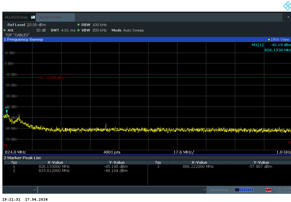
Plot 7-14. Conducted Spurious Plot (LTE Band 26 - 5MHz QPSK - RB Size 1, RB Offset 0 - Low Channel)
