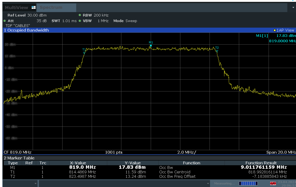
Plot 7-7. Occupied Bandwidth Plot (LTE Band 26 - 10MHz QPSK - Full RB)
