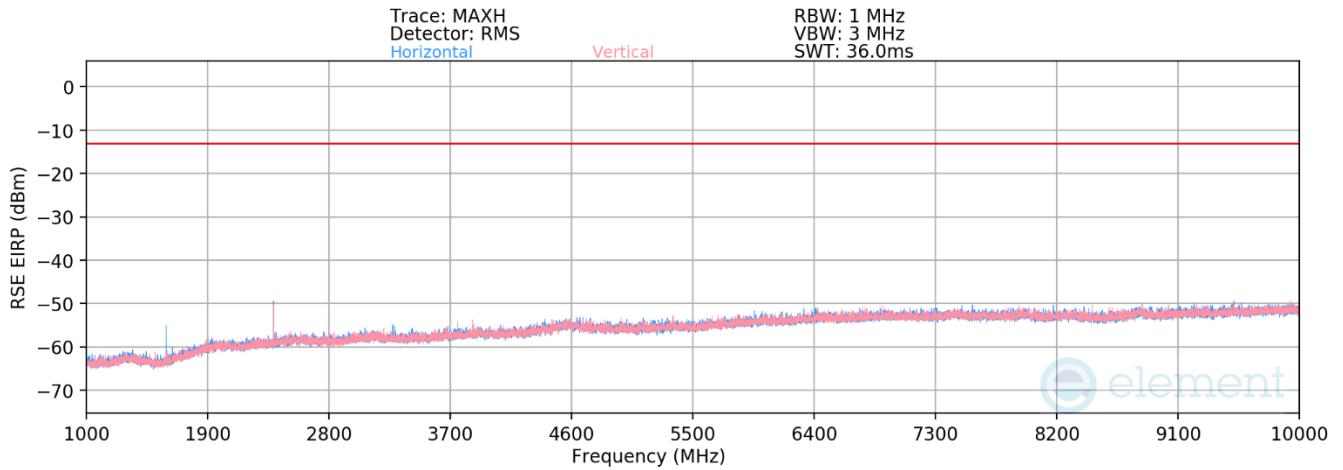
Plot 7-50. Antenna BCM Radiated Spurious Plot Above 1GHz (LTE Band 14)
