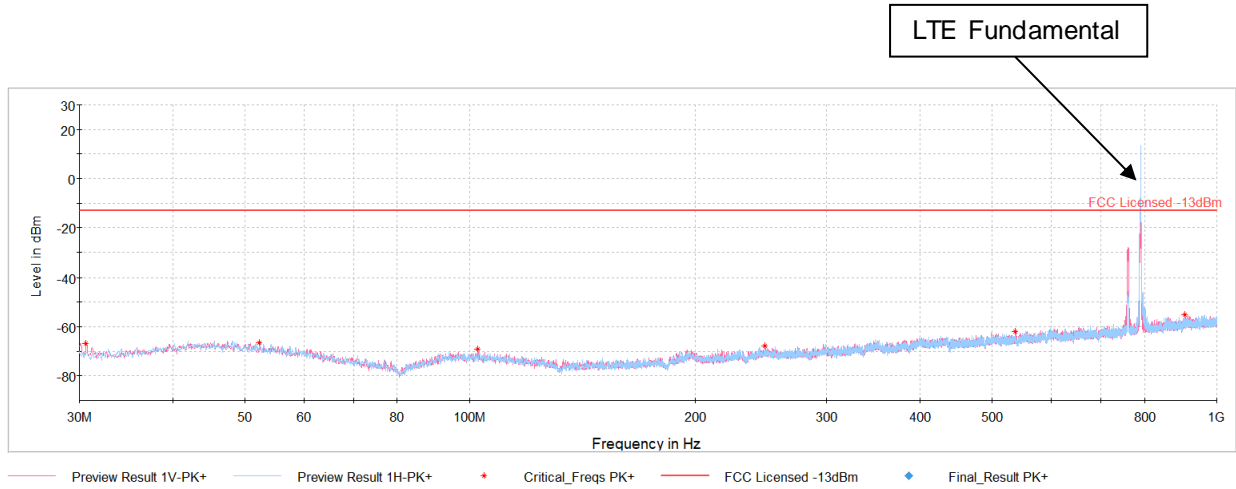
Plot 7-49. Antenna BCM Radiated Spurious Plot Below 1GHz (LTE Band 14)
