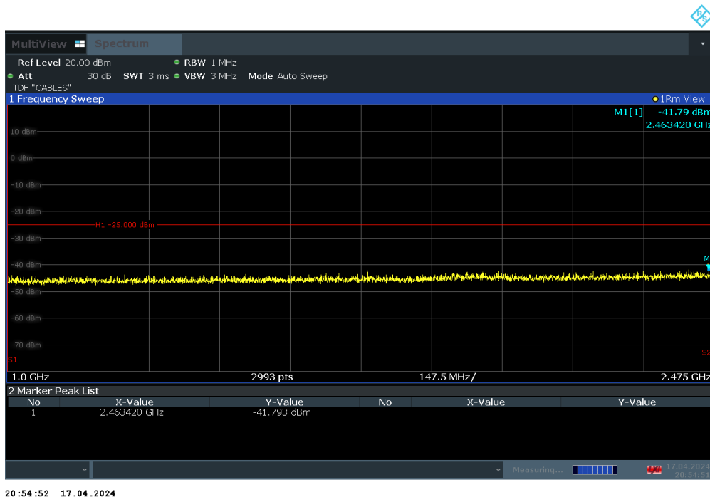
Plot 7-30. Conducted Spurious Plot (LTE Band 41 - 20MHz QPSK – RB Size 1, RB Offset 0 – Low Channel)
