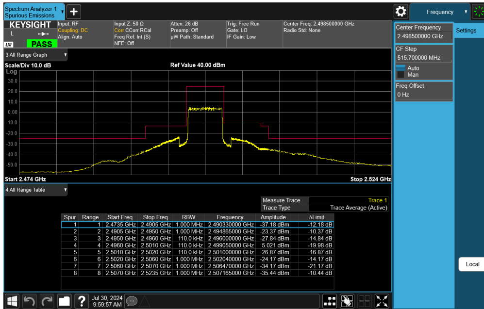
Plot 7-56. Lower ACP Plot (LTE Band 41 - 5MHz QPSK – Full RB)
