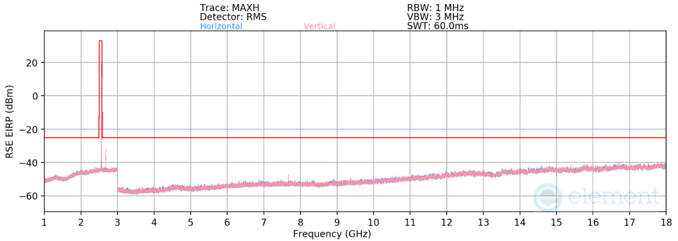
Plot 7-68. Antenna FCM Radiated Spurious Plot 1GHz – 18GHz (LTE Band 7)
