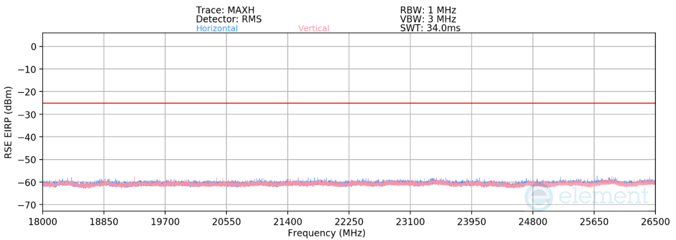
Plot 7-71. Antenna FCM Radiated Spurious Emission above 18GHz (LTE Band 41)
