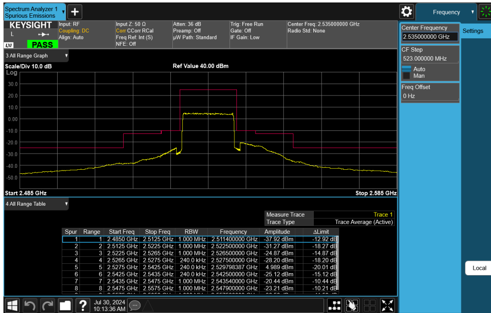
Plot 7-51. Middle ACP Plot (LTE Band 7 - 15MHz QPSK – Full RB)
