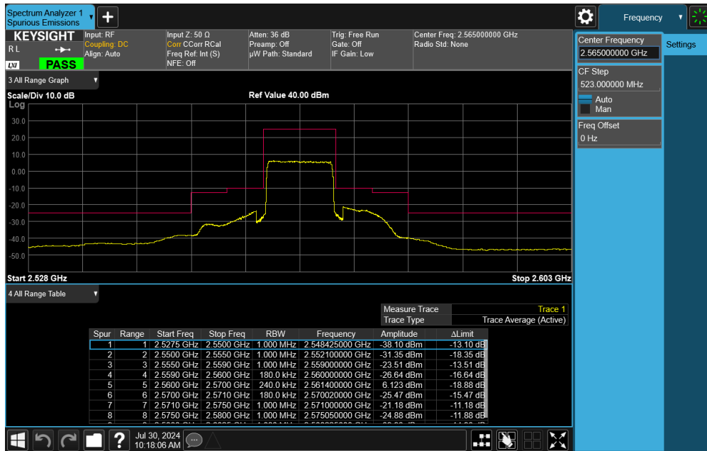
Plot 7-49. Upper ACP Plot (LTE Band 7 - 10MHz QPSK – Full RB)
