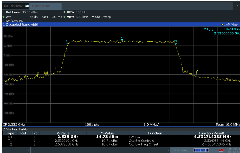
Plot 7-2. Occupied Bandwidth Plot (LTE Band 7 - 5MHz 16-QAM - Full RB)
