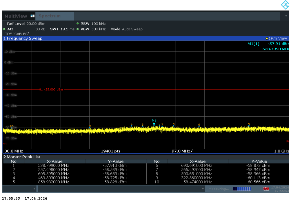
Plot 7-17. Conducted Spurious Plot (LTE Band 7 - 20MHz QPSK – RB Size 1, RB Offset 0 – Low Channel)
