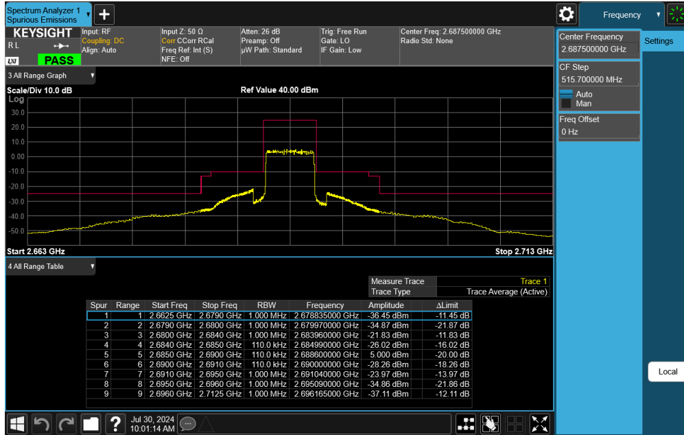
Plot 7-58. Upper ACP Plot (LTE Band 41 - 5MHz QPSK – Full RB)
