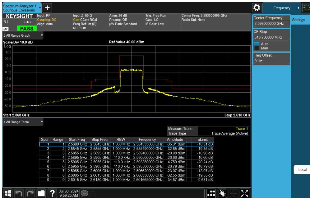
Plot 7-57. Middle ACP Plot (LTE Band 41 - 5MHz QPSK – Full RB)
