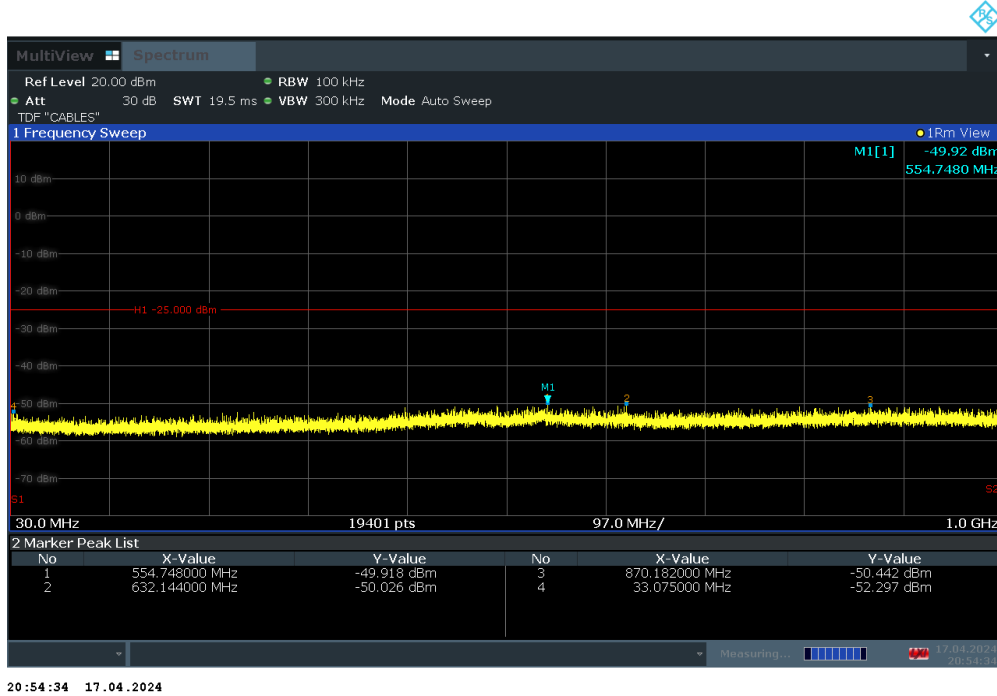
Plot 7-29. Conducted Spurious Plot (LTE Band 41 - 20MHz QPSK – RB Size 1, RB Offset 0 – Low Channel)
