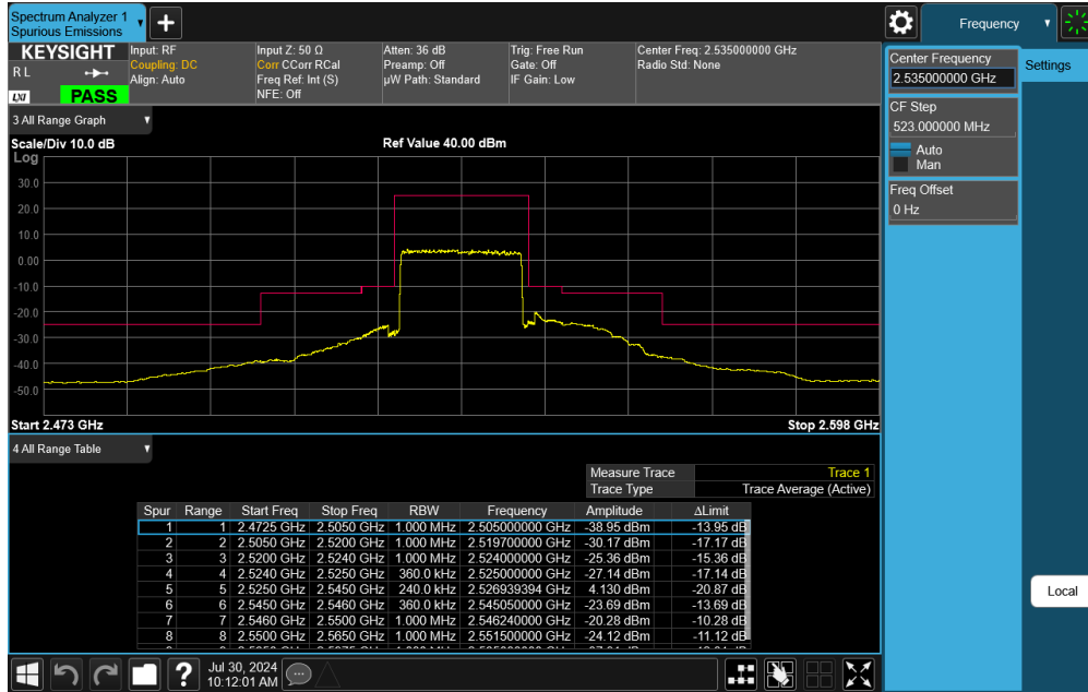
Plot 7-54. Middle ACP Plot (LTE Band 7 - 20MHz QPSK – Full RB)
