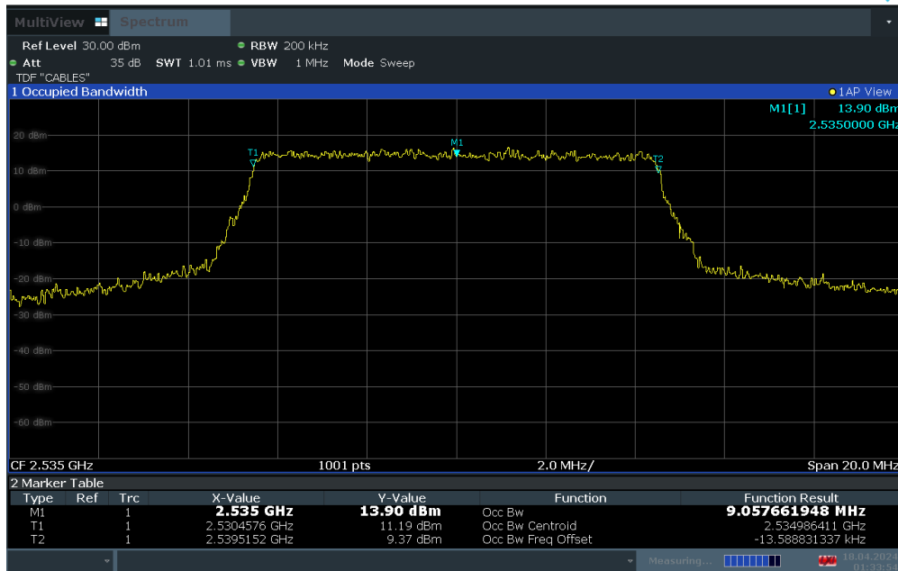
Plot 7-3. Occupied Bandwidth Plot (LTE Band 7 - 10MHz QPSK - Full RB)
