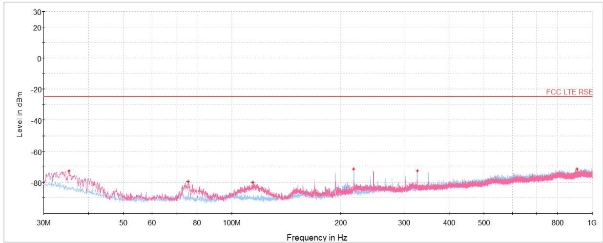
Plot 7-72. Antenna FCM Radiated Spurious Emissions -Simultaneous Transmission 30MHz – 1GHz
