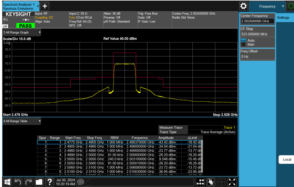
Plot 7-44. Lower ACP Plot (LTE Band 7 - 5MHz QPSK – Full RB)
