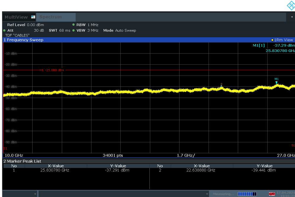
Plot 7-28. Conducted Spurious Plot (LTE Band 7 - 20MHz QPSK – RB Size 1, RB Offset 0 – High Channel)
