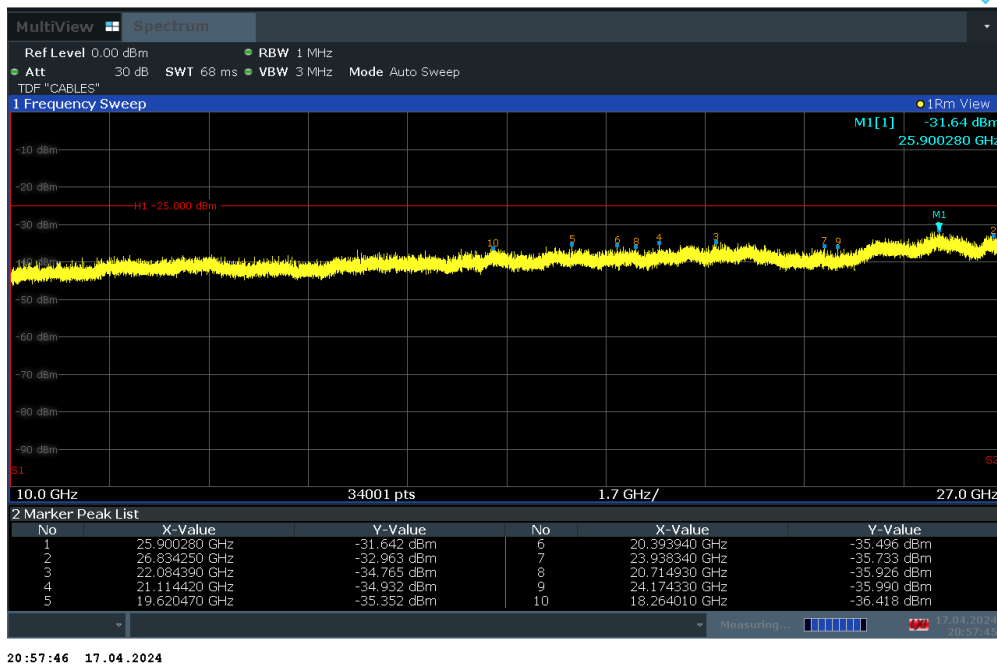
Plot 7-36. Conducted Spurious Plot (LTE Band 41 - 20MHz QPSK – RB Size 1, RB Offset 0 – Mid Channel)
