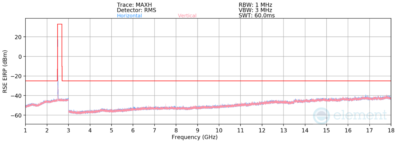
Plot 7-70. Antenna FCM Radiated Spurious Plot 1GHz – 18GHz (LTE Band 41)
