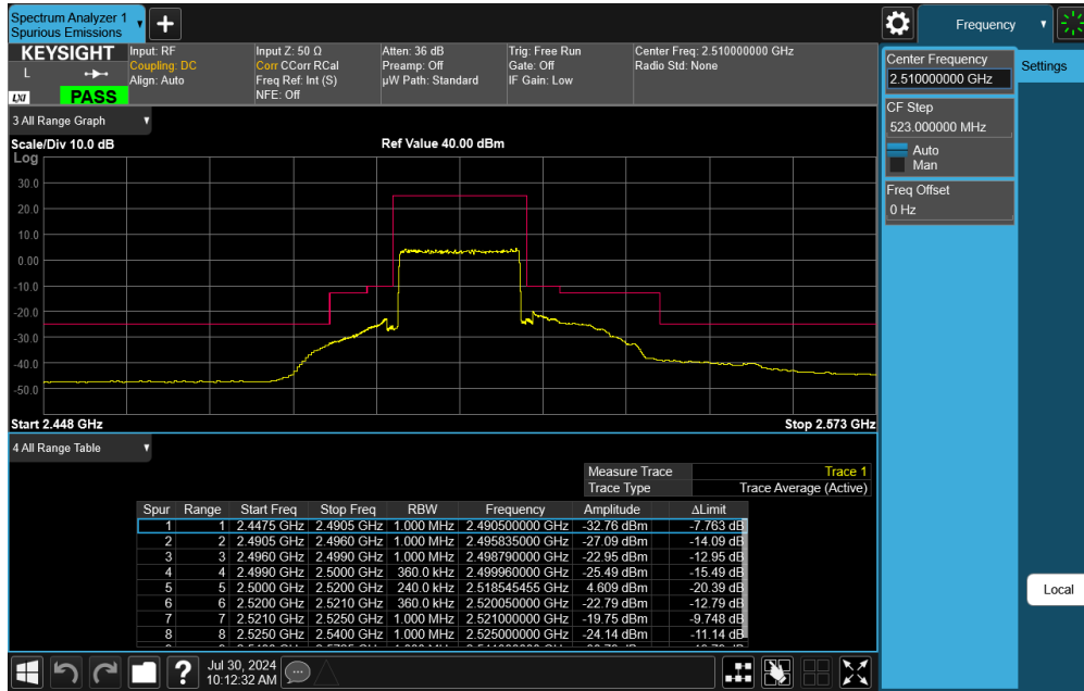
Plot 7-53. Lower ACP Plot (LTE Band 7 - 20MHz QPSK – Full RB)
