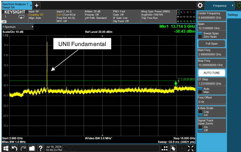
Plot 7-42. Simultaneous Tx Conducted Spurious Plot (LTE Band 41 + BT + UNII)
