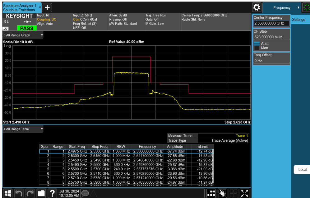
Plot 7-55. Upper ACP Plot (LTE Band 7 - 20MHz QPSK – Full RB)
