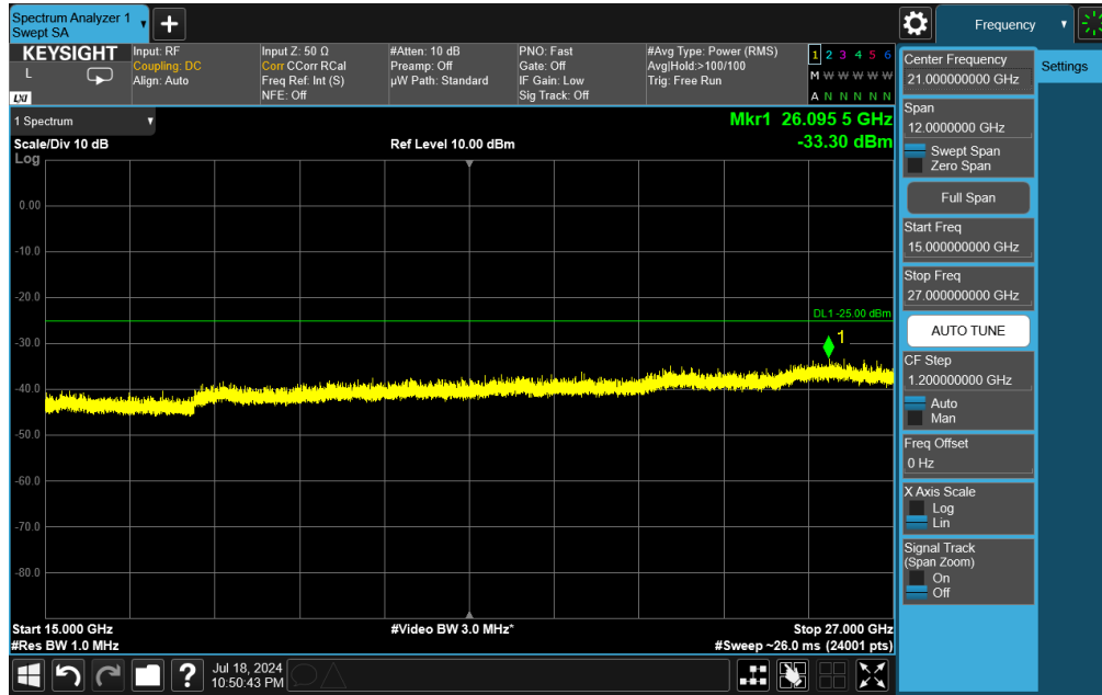
Plot 7-43. Simultaneous Tx Conducted Spurious Plot (LTE Band 41 + BT + UNII)
