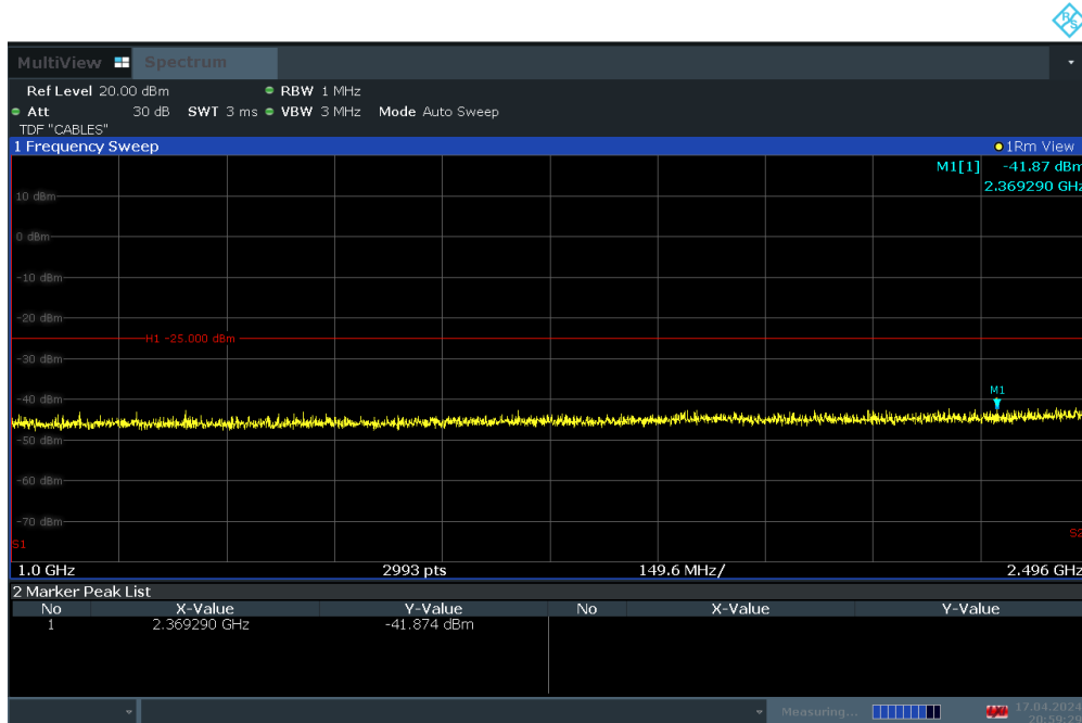
Plot 7-38. Conducted Spurious Plot (LTE Band 41 - 20MHz QPSK – RB Size 1, RB Offset 0 – High Channel)
