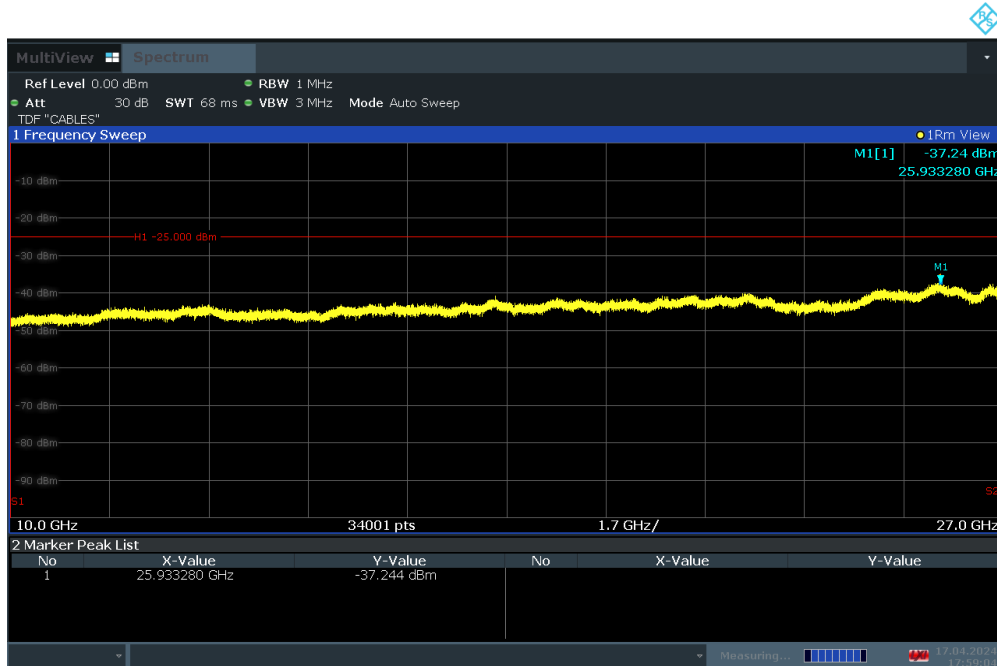
Plot 7-24. Conducted Spurious Plot (LTE Band 7 - 20MHz QPSK – RB Size 1, RB Offset 0 – Mid Channel)
