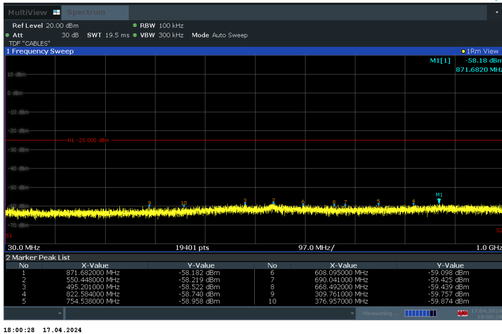
Plot 7-25. Conducted Spurious Plot (LTE Band 7 - 20MHz QPSK – RB Size 1, RB Offset 0 – High Channel)
