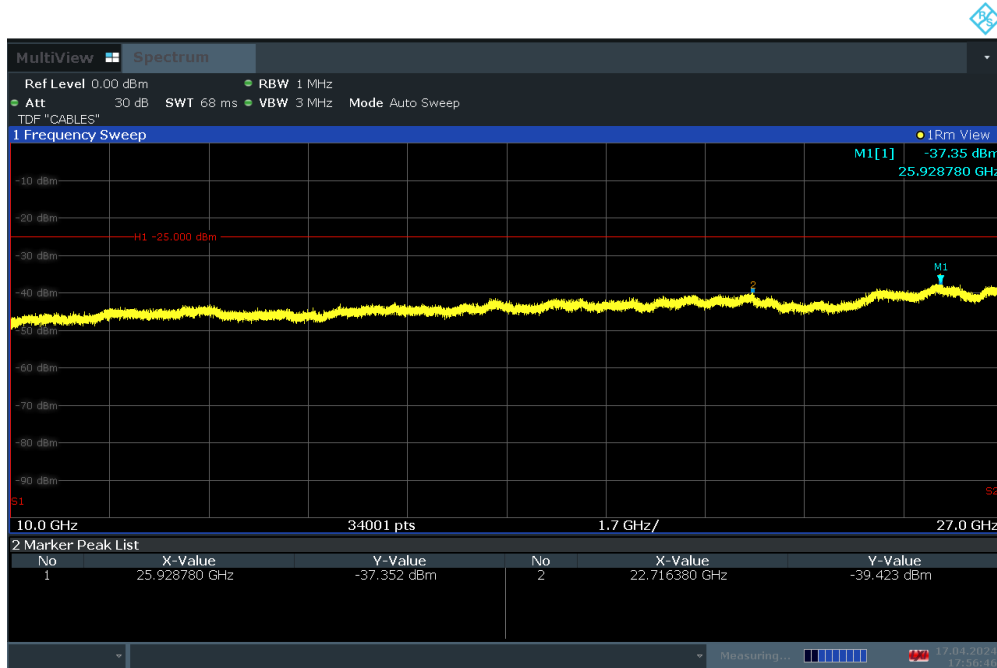
Plot 7-20. Conducted Spurious Plot (LTE Band 7 - 20MHz QPSK – RB Size 1, RB Offset 0 – Low Channel)
