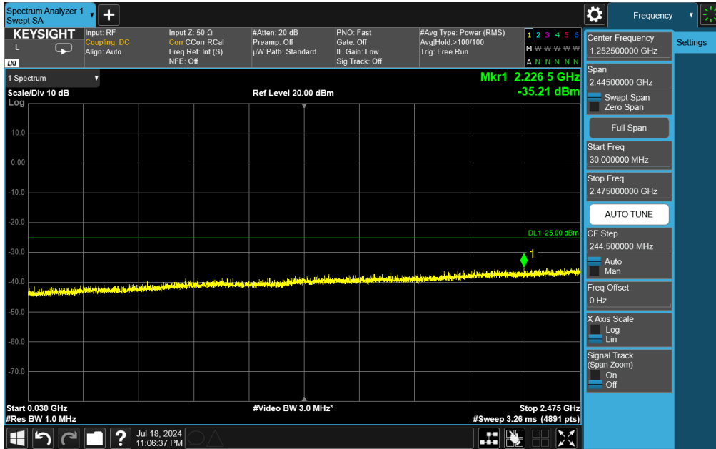
Plot 7-41. Simultaneous Tx Conducted Spurious Plot (LTE Band 41 + BT + UNII)
