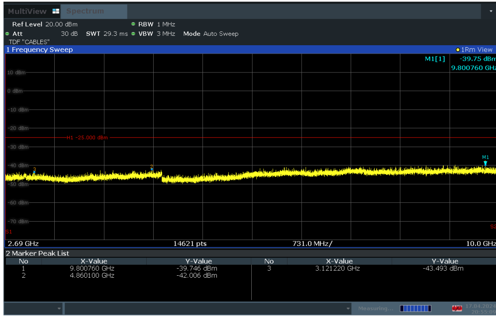
Plot 7-31. Conducted Spurious Plot (LTE Band 41 - 20MHz QPSK – RB Size 1, RB Offset 0 – Low Channel)
