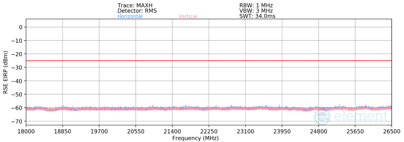
Plot 7-69. Antenna FCM Radiated Spurious Emission above 18GHz (LTE Band 7)
