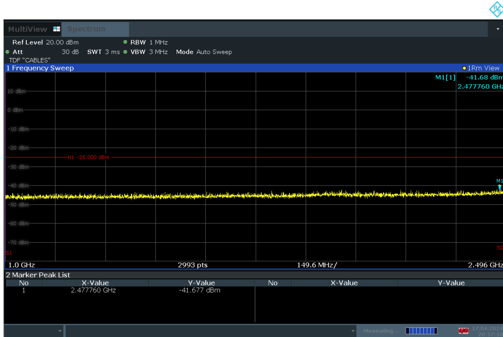
Plot 7-34. Conducted Spurious Plot (LTE Band 41 - 20MHz QPSK – RB Size 1, RB Offset 0 – Mid Channel)
