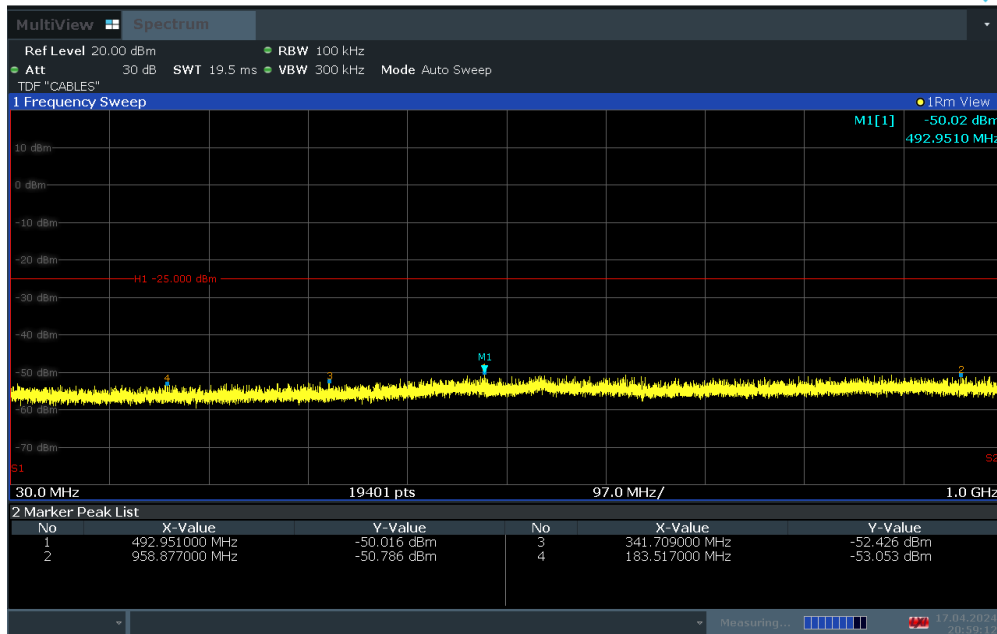
Plot 7-37. Conducted Spurious Plot (LTE Band 41 - 20MHz QPSK – RB Size 1, RB Offset 0 – High Channel)
