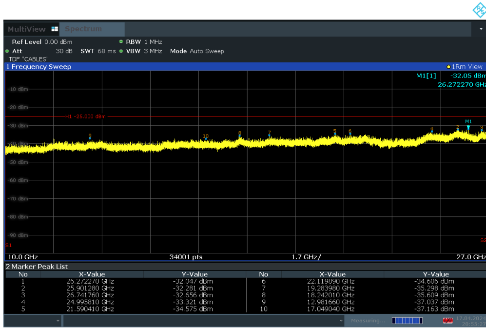
Plot 7-32. Conducted Spurious Plot (LTE Band 41 - 20MHz QPSK – RB Size 1, RB Offset 0 – Low Channel)
