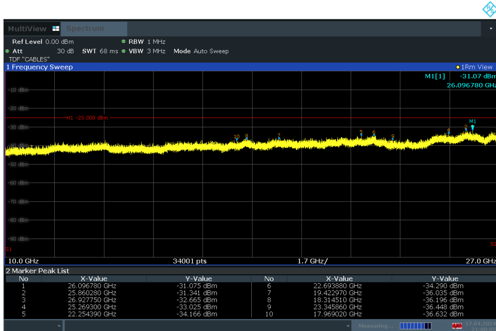
Plot 7-40. Conducted Spurious Plot (LTE Band 41 - 20MHz QPSK – RB Size 1, RB Offset 0 – High Channel)
