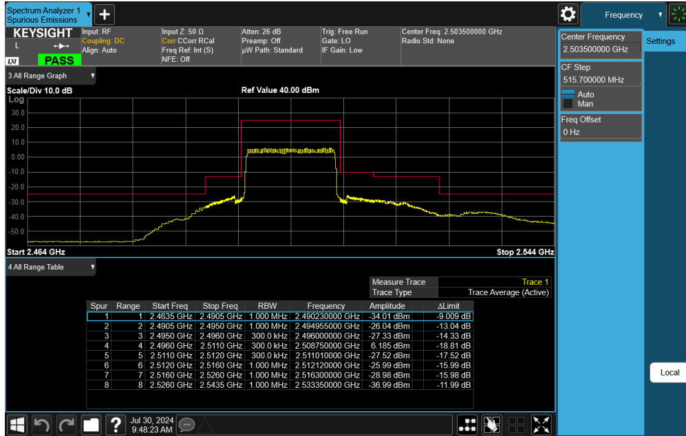
Plot 7-62. Lower ACP Plot (LTE Band 41 - 15MHz QPSK - Full RB)
