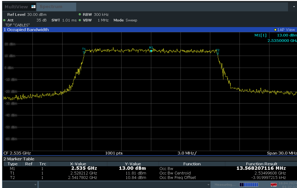
Plot 7-5. Occupied Bandwidth Plot (LTE Band 7 - 15MHz QPSK - Full RB)
