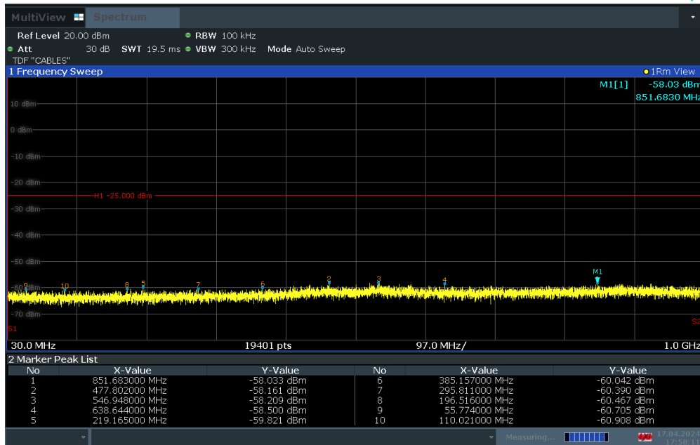
Plot 7-21. Conducted Spurious Plot (LTE Band 7 - 20MHz QPSK – RB Size 1, RB Offset 0 – Mid Channel)
