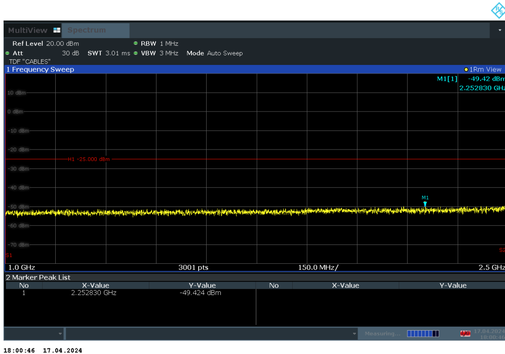
Plot 7-26. Conducted Spurious Plot (LTE Band 7 - 20MHz QPSK – RB Size 1, RB Offset 0 – High Channel)
