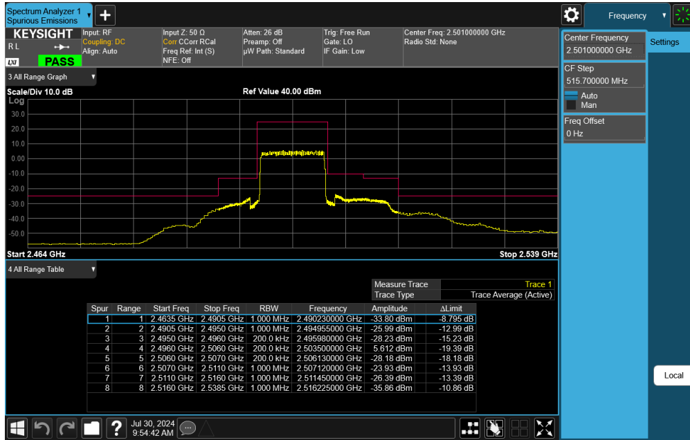
Plot 7-59. Lower ACP Plot (LTE Band 41 - 10MHz QPSK – Full RB)
