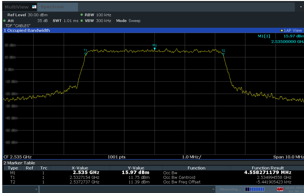
Plot 7-1. Occupied Bandwidth Plot (LTE Band 7 - 5MHz QPSK - Full RB)
