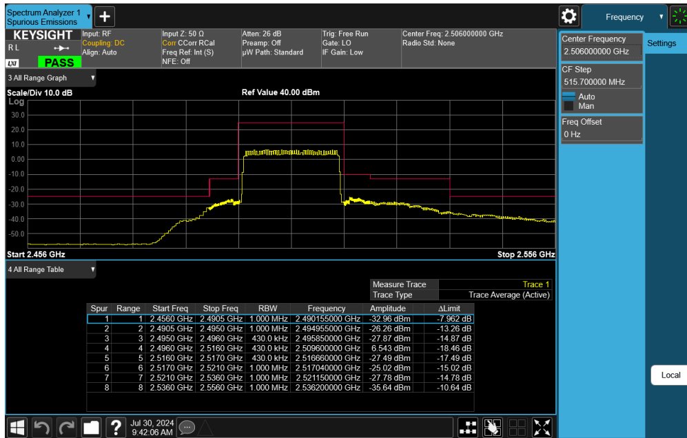
Plot 7-65. Lower ACP Plot (LTE Band 41 - 20MHz QPSK – Full RB)
