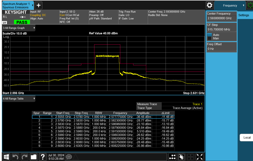
Plot 7-60. Middle ACP Plot (LTE Band 41 - 10MHz QPSK – Full RB)
