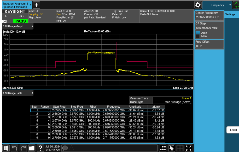
Plot 7-64. Upper ACP Plot (LTE Band 41 - 15MHz QPSK – Full RB)
