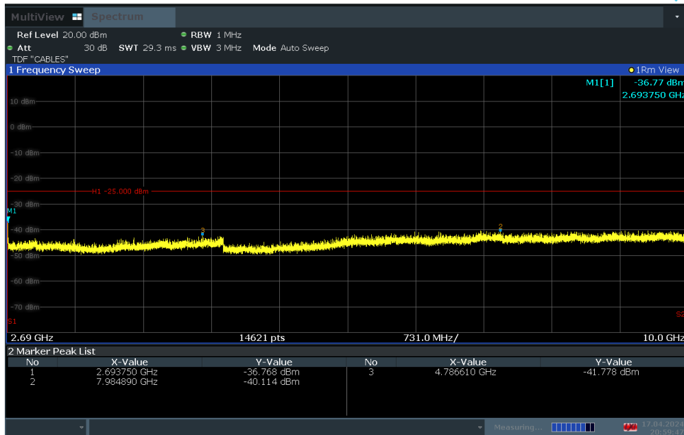
Plot 7-39. Conducted Spurious Plot (LTE Band 41 - 20MHz QPSK – RB Size 1, RB Offset 0 – High Channel)
