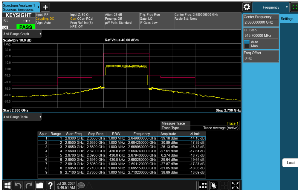
Plot 7-67. Upper ACP Plot (LTE Band 41 - 20MHz QPSK – Full RB)
