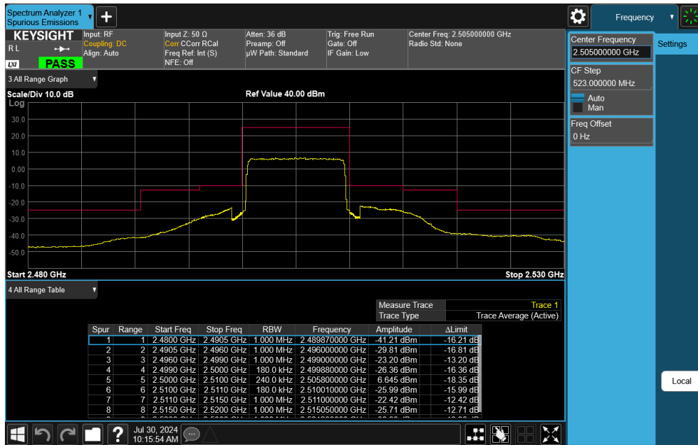
Plot 7-47. Lower ACP Plot (LTE Band 7 - 10MHz QPSK – Full RB)
