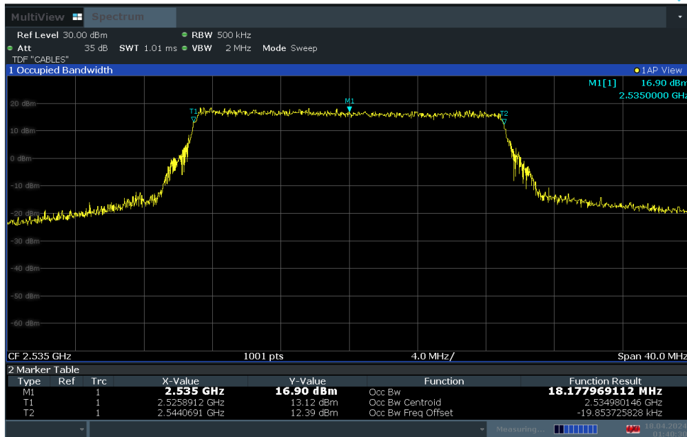
Plot 7-7. Occupied Bandwidth Plot (LTE Band 7 - 20MHz QPSK - Full RB)
