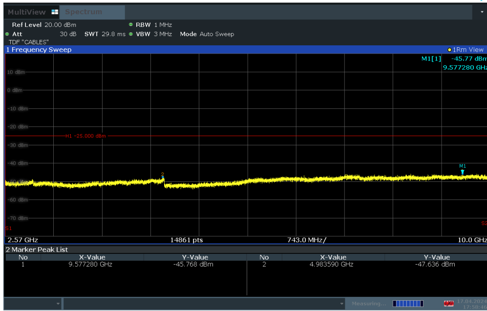
Plot 7-23. Conducted Spurious Plot (LTE Band 7 - 20MHz QPSK – RB Size 1, RB Offset 0 – Mid Channel)
