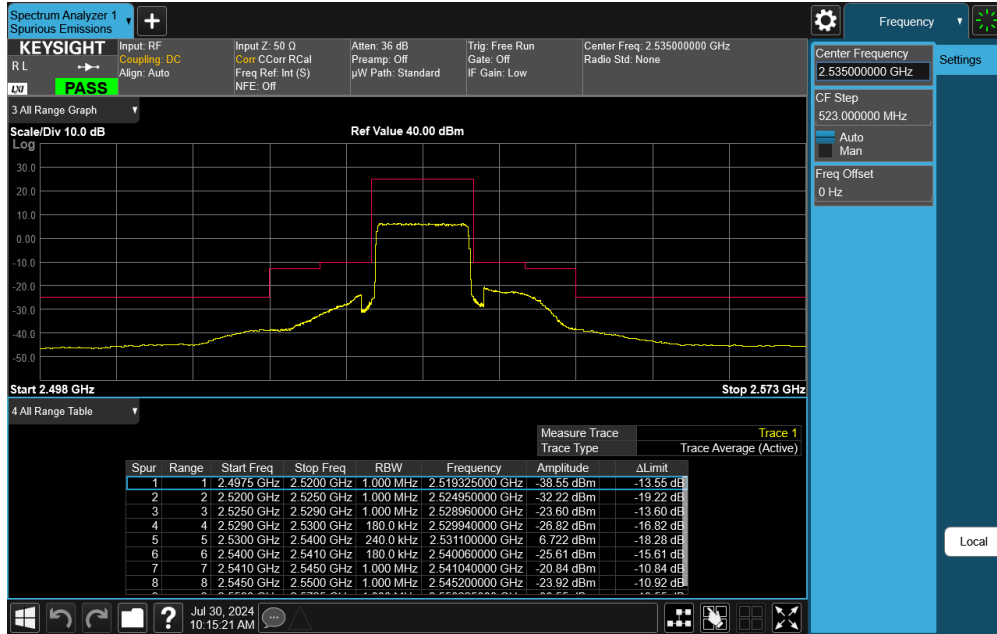
Plot 7-48. Middle ACP Plot (LTE Band 7 - 10MHz QPSK – Full RB)
