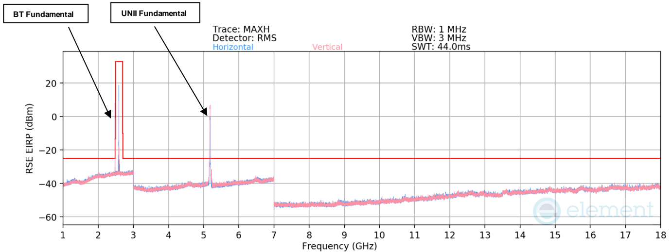
Plot 7-73. Antenna FCM Radiated Spurious Emissions -Simultaneous Transmission 1GHz – 18GHz
