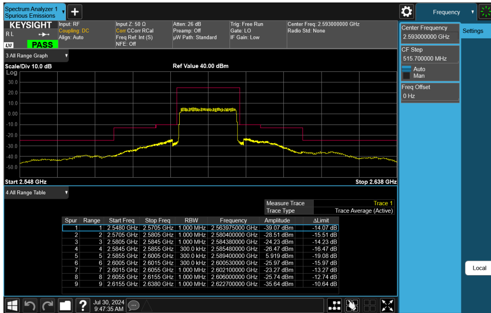
Plot 7-63. Middle ACP Plot (LTE Band 41 - 15MHz QPSK - Full RB)
