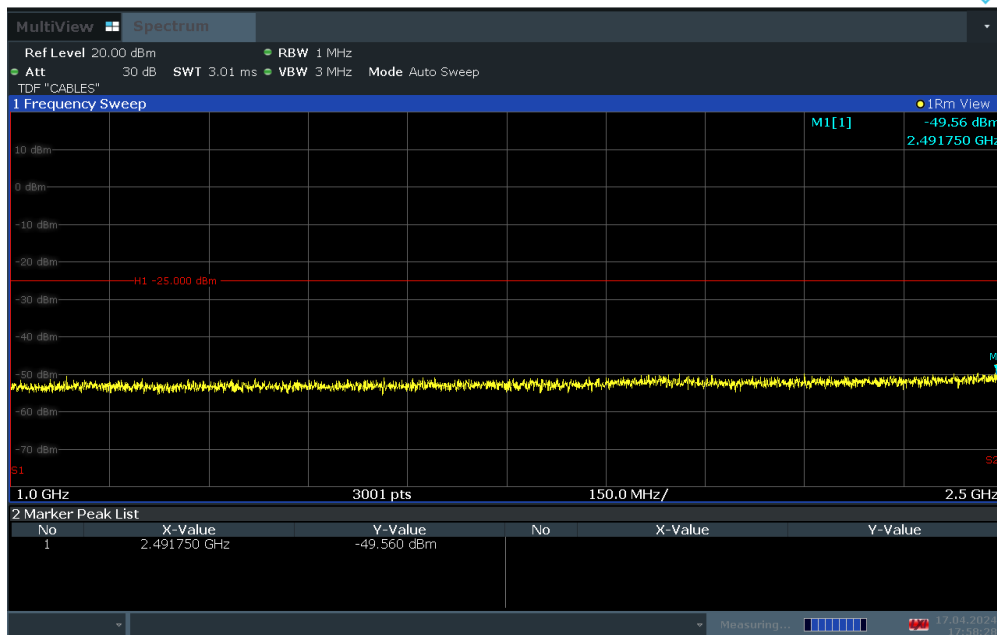
Plot 7-22. Conducted Spurious Plot (LTE Band 7 - 20MHz QPSK – RB Size 1, RB Offset 0 – Mid Channel)
