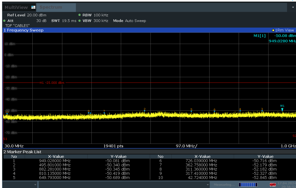
Plot 7-33. Conducted Spurious Plot (LTE Band 41 - 20MHz QPSK – RB Size 1, RB Offset 0 – Mid Channel)
