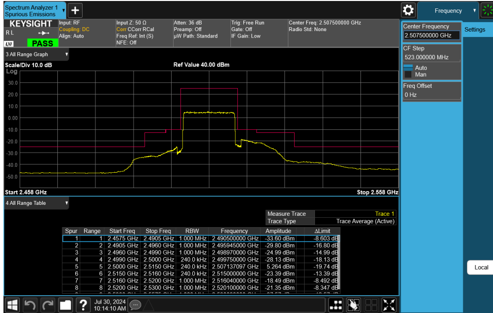
Plot 7-50. Lower ACP Plot (LTE Band 7 - 15MHz QPSK – Full RB)
