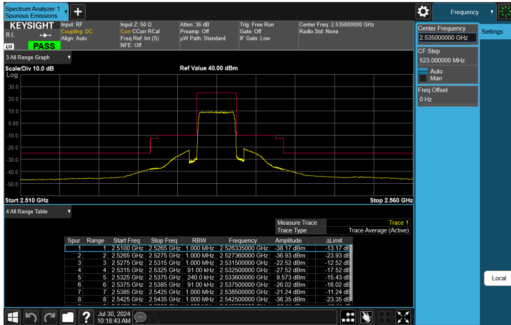
Plot 7-45. Middle ACP Plot (LTE Band 7 - 5MHz QPSK – Full RB)
