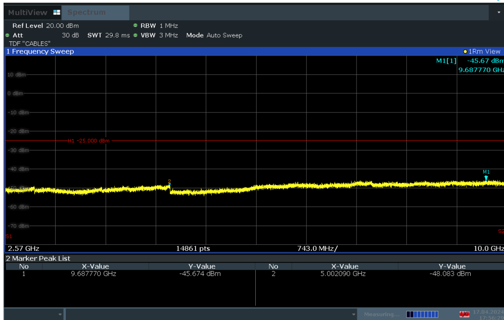
Plot 7-19. Conducted Spurious Plot (LTE Band 7 - 20MHz QPSK – RB Size 1, RB Offset 0 – Low Channel)
