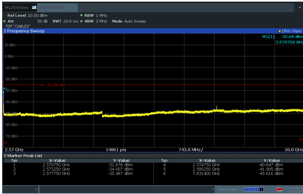
Plot 7-27. Conducted Spurious Plot (LTE Band 7 - 20MHz QPSK – RB Size 1, RB Offset 0 – High Channel)
