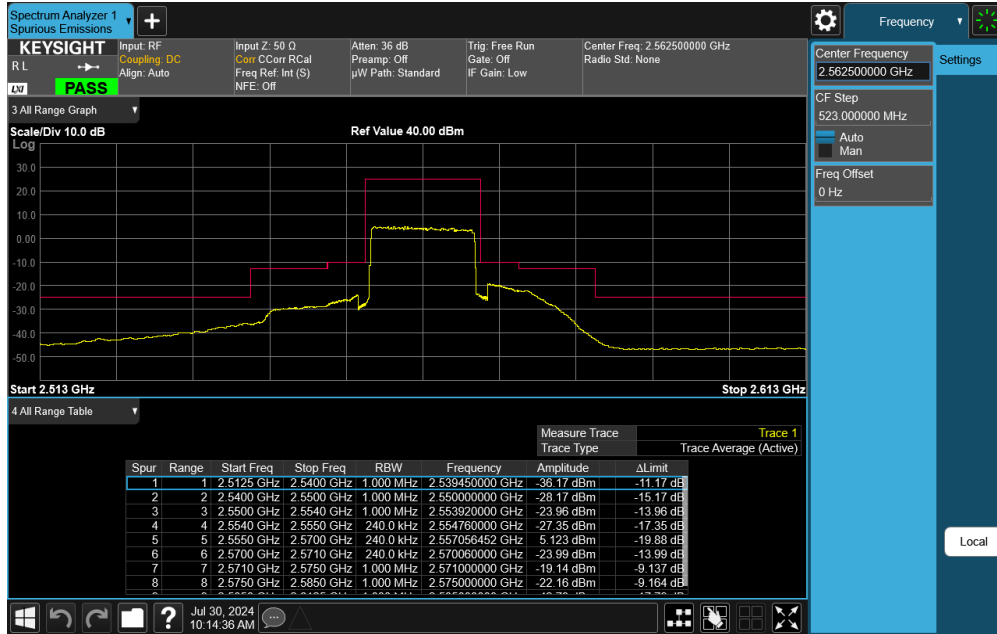
Plot 7-52. Upper ACP Plot (LTE Band 7 - 15MHz QPSK – Full RB)
