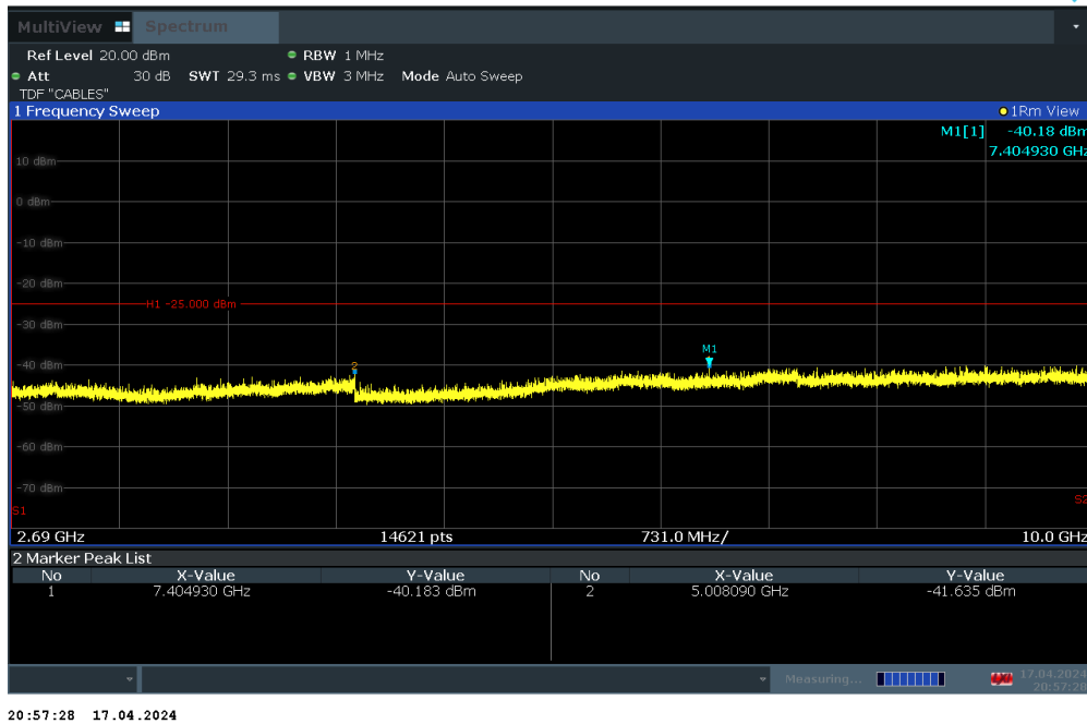
Plot 7-35. Conducted Spurious Plot (LTE Band 41 - 20MHz QPSK – RB Size 1, RB Offset 0 – Mid Channel)
