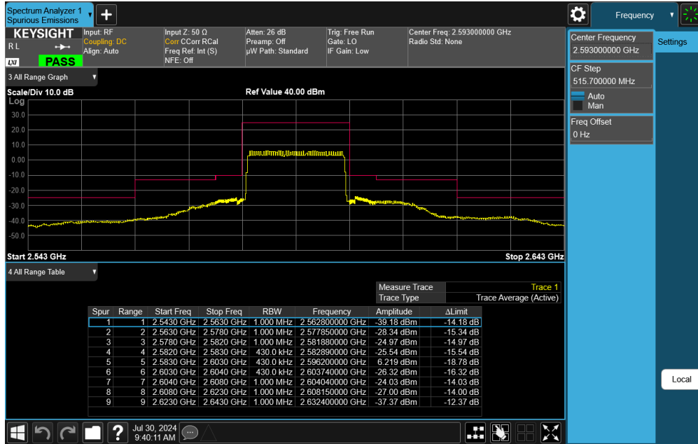
Plot 7-66. Middle ACP Plot (LTE Band 41 - 20MHz QPSK – Full RB)
