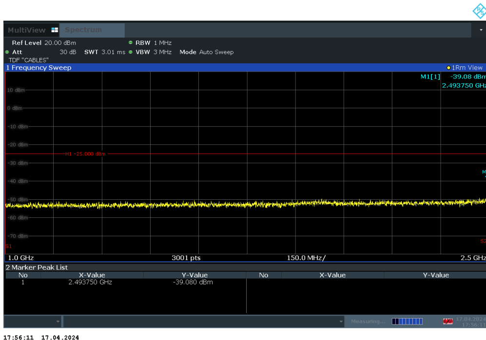
Plot 7-18. Conducted Spurious Plot (LTE Band 7 - 20MHz QPSK – RB Size 1, RB Offset 0 – Low Channel)
