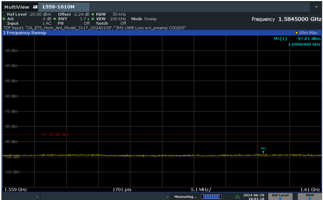
Plot 7-21. Radiated Spurious Emission 1559-1610MHz (Ch. 5, Config 409, Payload 4093 Ant. Pol. H)
