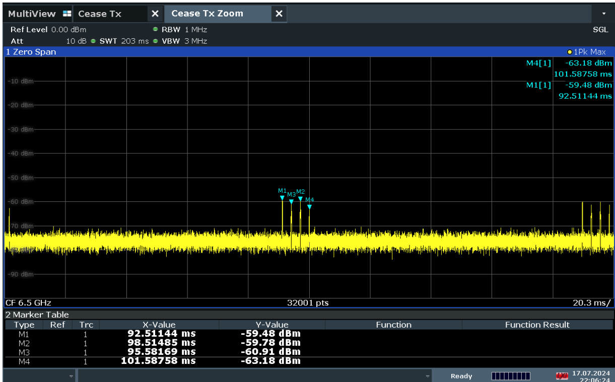
Plot 7-10. Zoom in Cessation Time – Mode1 (Ch. 5, 6.5 GHz)
