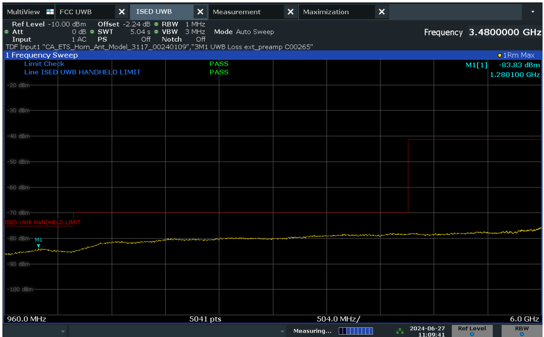
Plot 7-18. ISED Radiated Spurious Emission 960-6000MHz (Ch. 5, Config 409, Payload 4093 Ant. Pol. V)
