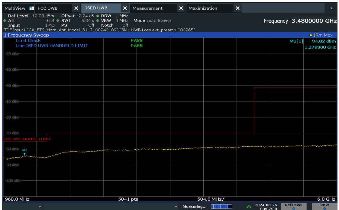
Plot 7-28. ISED Radiated Spurious Emission 960-6000MHz (Ch.9, Config 409, Payload 4093 Ant. Pol. V)
