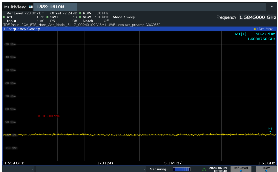
Plot 7-22. Radiated Spurious Emission 1559-1610MHz (Ch. 5, Config 409, Payload 4093 Ant. Pol. V)
