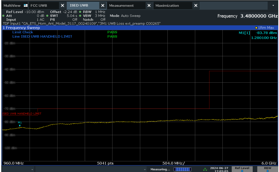
Plot 7-17. ISED Radiated Spurious Emission 960-6000MHz (Ch. 5, Config 409, Payload 4093 Ant. Pol. H)
