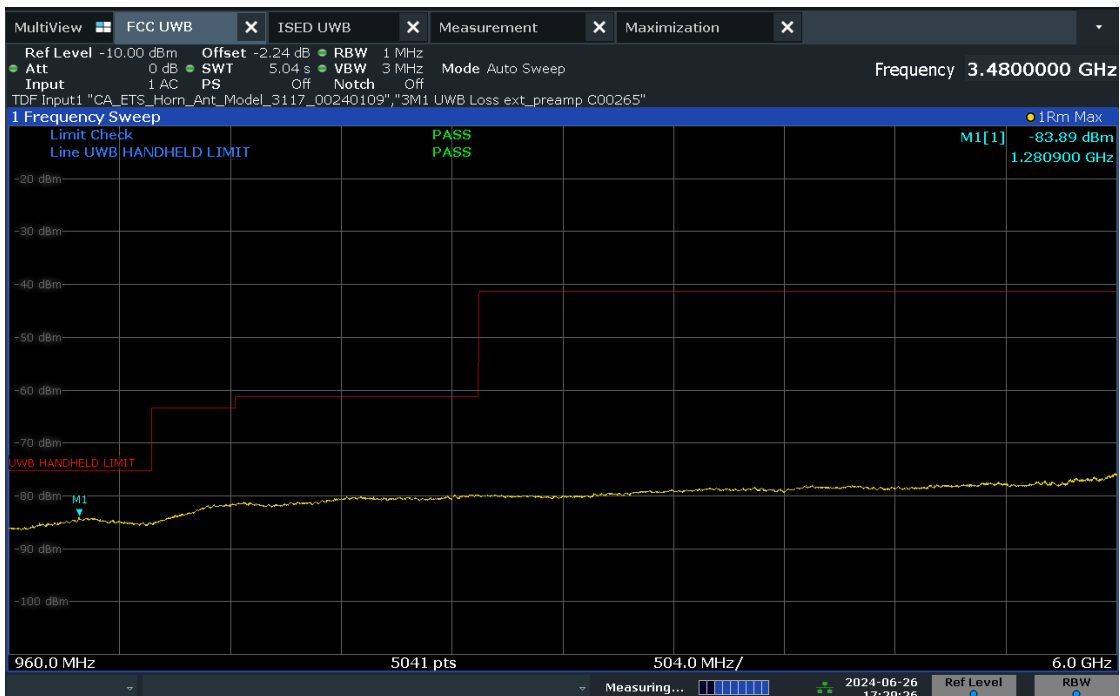
Plot 7-16. FCC Radiated Spurious Emissions 960-6000MHz (Ch. 5, Config 409, Payload 4093 Ant. Pol. V)
