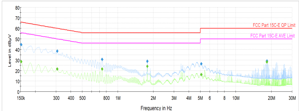
Plot 7-41. AC Line Conducted (Ch. 5, Config 409, Payload 4093 L1, with AC/DC Adapter + Magnetic Charger)
