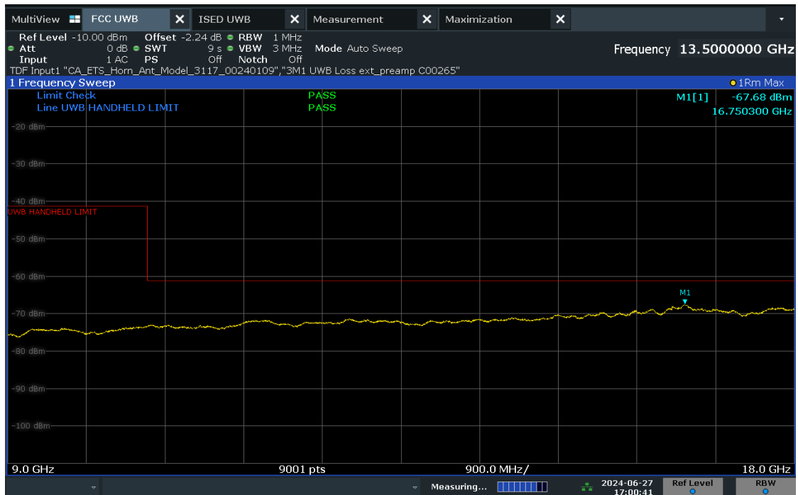
Plot 7-24. Radiated Spurious Emission 9-18GHz (Ch. 5, Config 409, Payload 4093 Ant. Pol. H)
