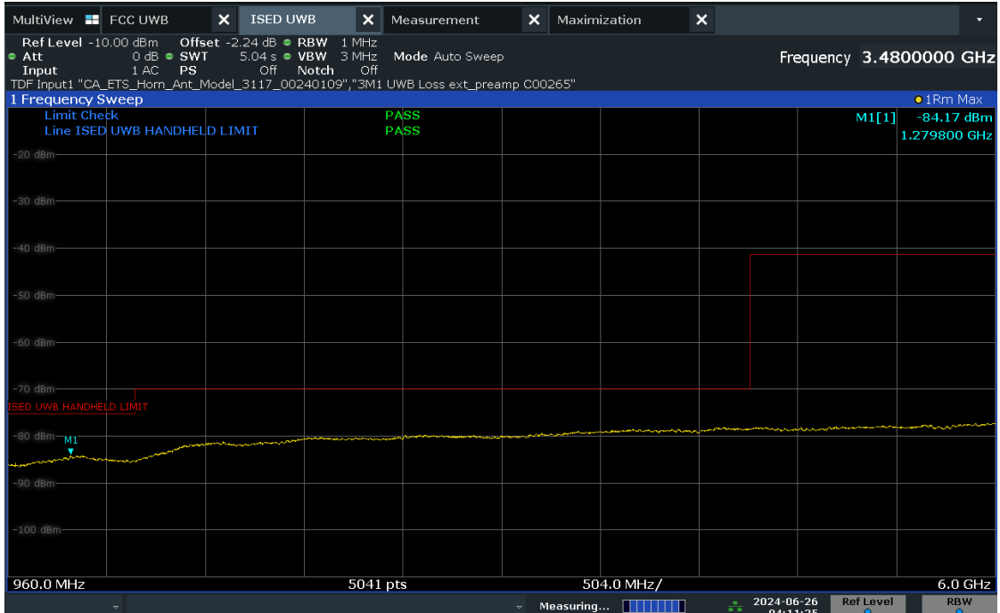
Plot 7-27. ISED Radiated Spurious Emission 960-6000MHz (Ch. 9, Config 409, Payload 4093 Ant. Pol. H)
