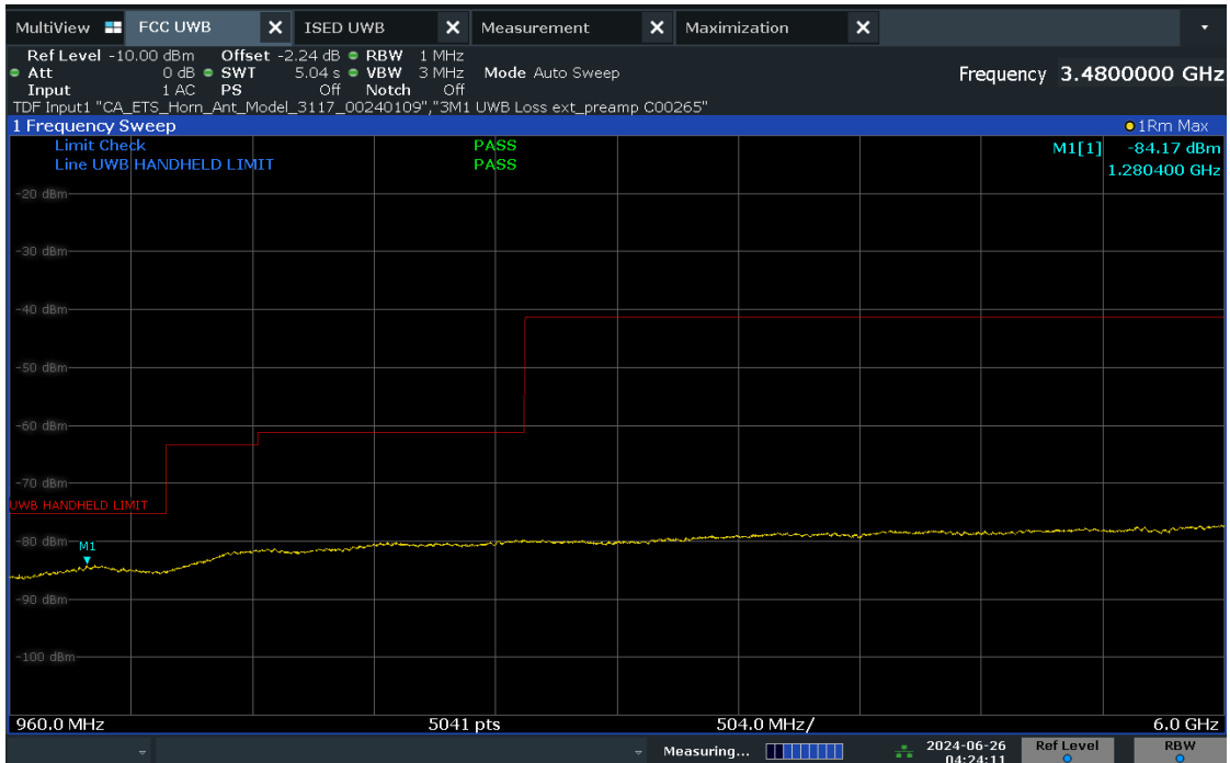
Plot 7-25. FCC Radiated Spurious Emission 960-6000MHz (Ch. 9, Config 409, Payload 4093 Ant. Pol. H)
