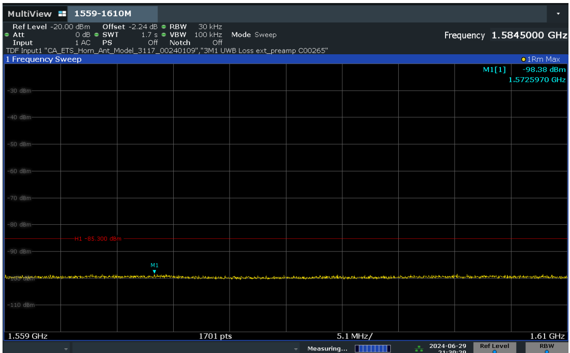
Plot 7-32. Radiated Spurious Emission 1559-1610MHz (Ch. 9, Config 409, Payload 4093 Ant. Pol. V)
