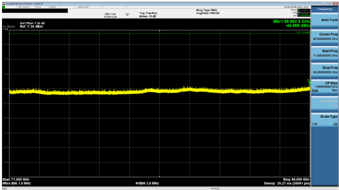
Plot 6-6. Radiated Spurious Emissions 71GHz – 90GHz (Mode 1)
