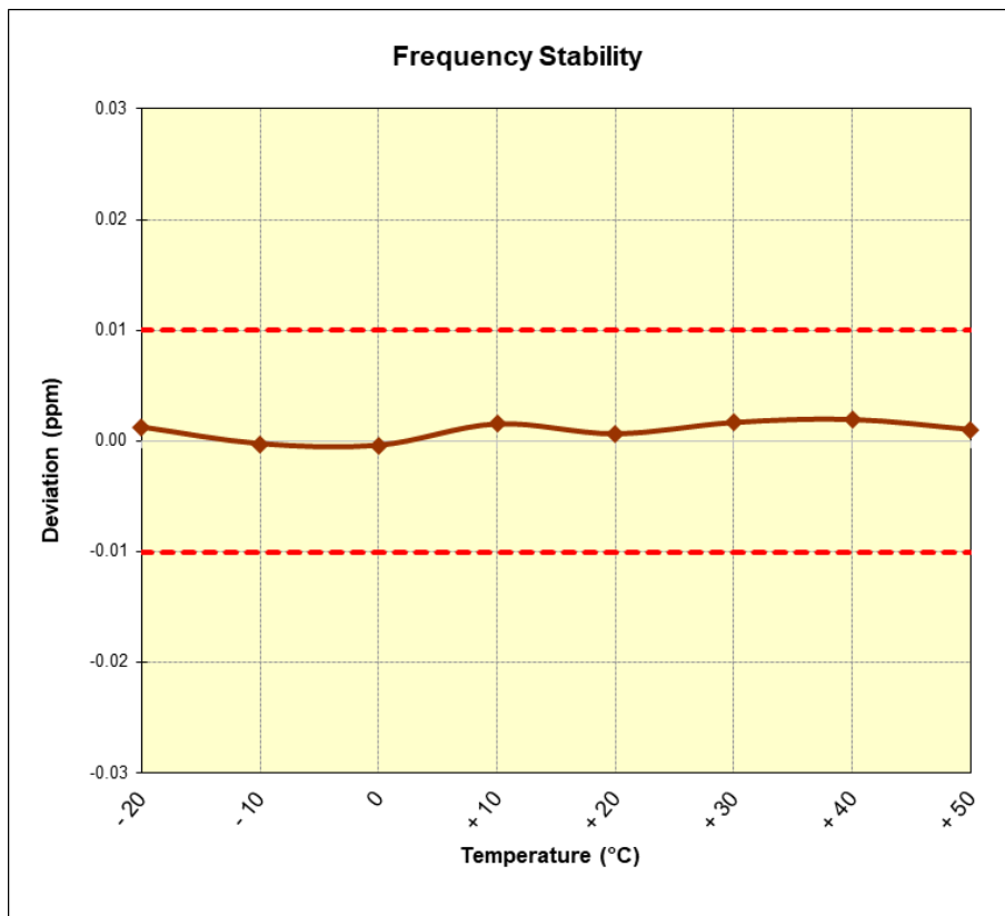
Figure 7-4. Frequency Stability Plot (Reader 10% ASK 1 out of 256)
