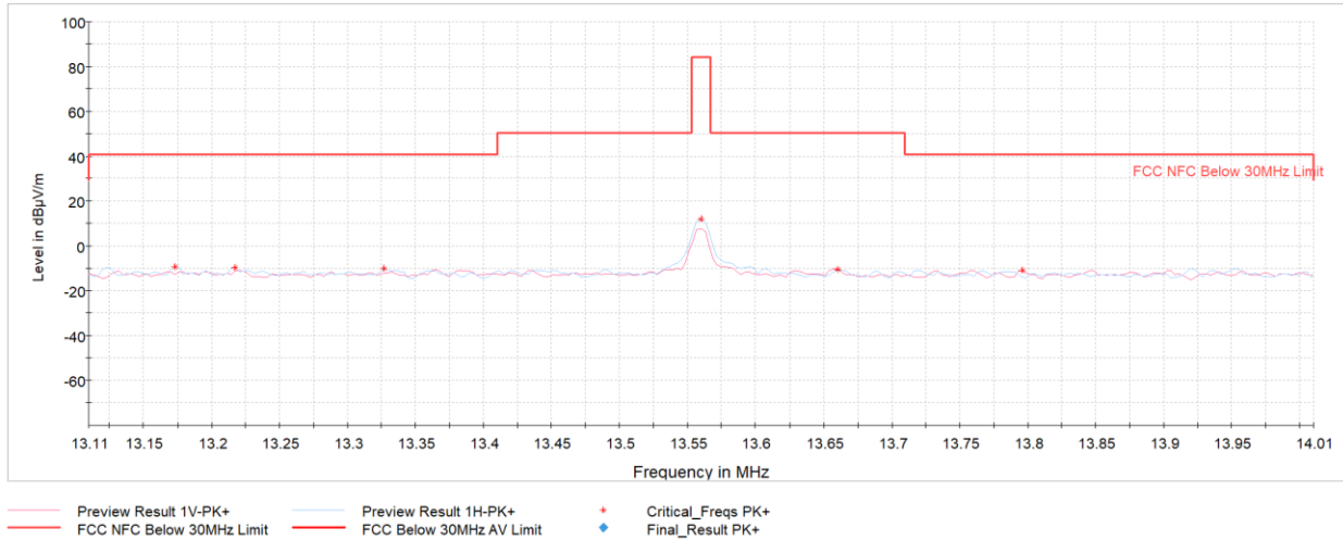
Plot 7-7. In Band Radiated Spurious Emissions (Reader A 848kbps, AC/DC Adapter and Magnetic Charger)
