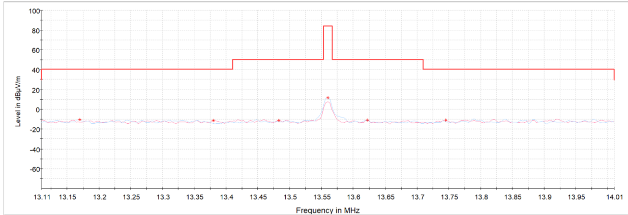
Plot 7-6. In Band Radiated Spurious Emissions (CE B 848kbps, with AC/DC Adapter and Magnetic Charger)
