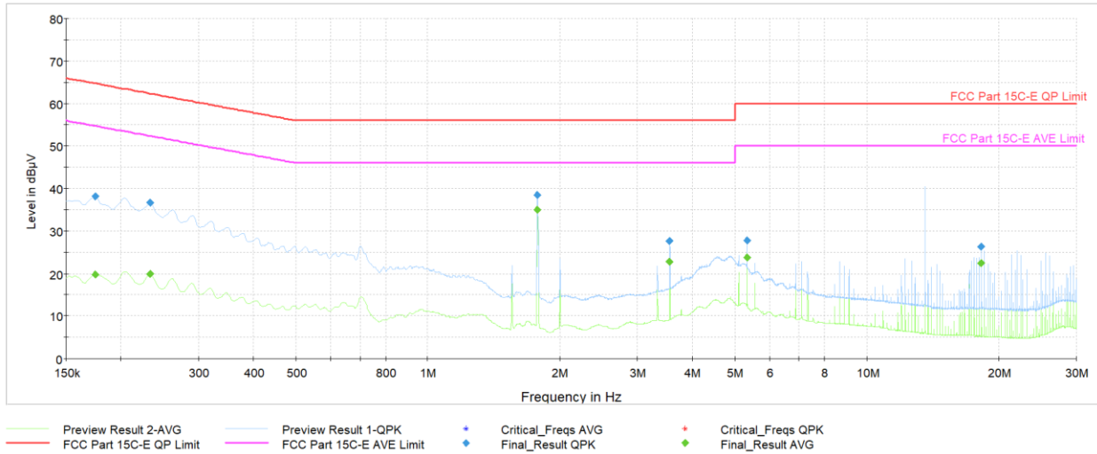
Plot 7-12. AC Line-Conducted Plot (L1, CE B 848kbps, with AC/DC Adapter and Magnetic Charger)
