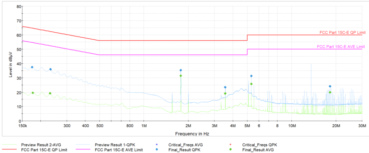
Plot 7-13. AC Line-Conducted Plot (N, CE B 848kbps, with AC/DC Adapter and Magnetic Charger)
