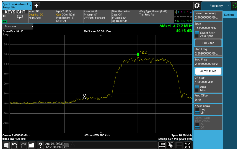
Plot 7-21. Band Edge Plot (Bluetooth (HDR8), ePA – Ch. 1)
