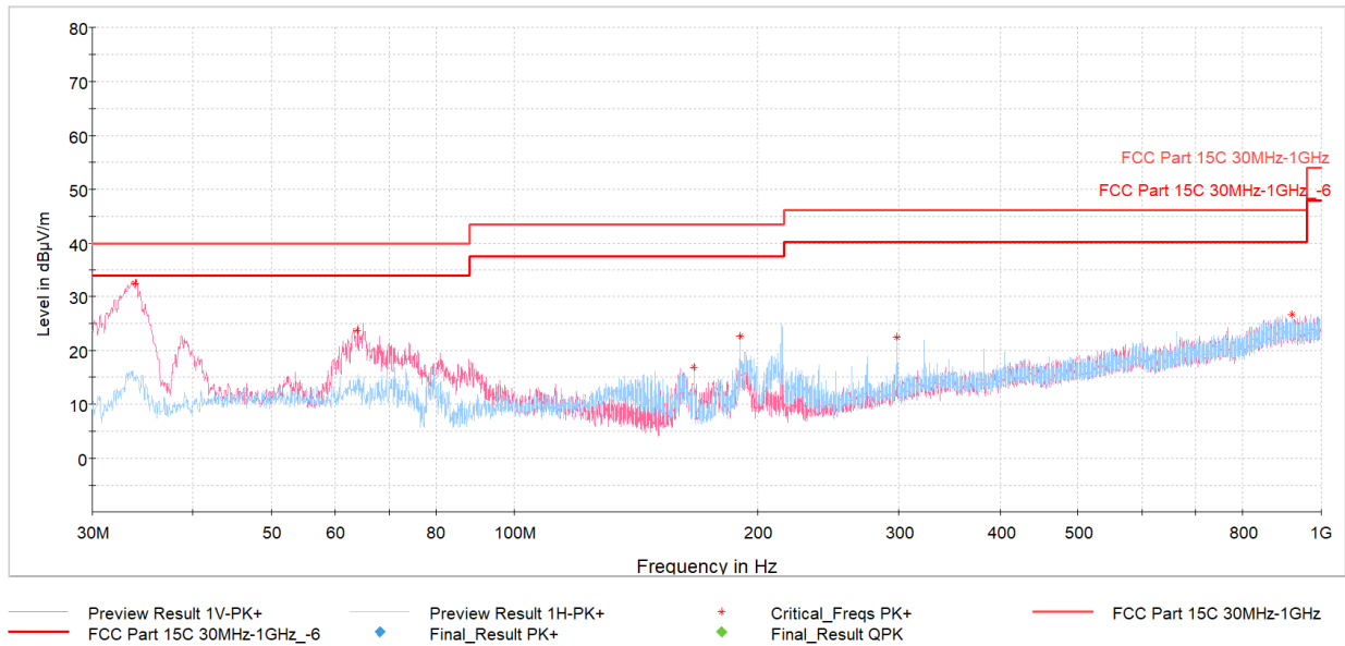
Plot 7-38. Radiated Spurious Emissions Below 1GHz (HDR4 ePA – Ch.38 with AC/DC Adapter + Magnetic Charger)
