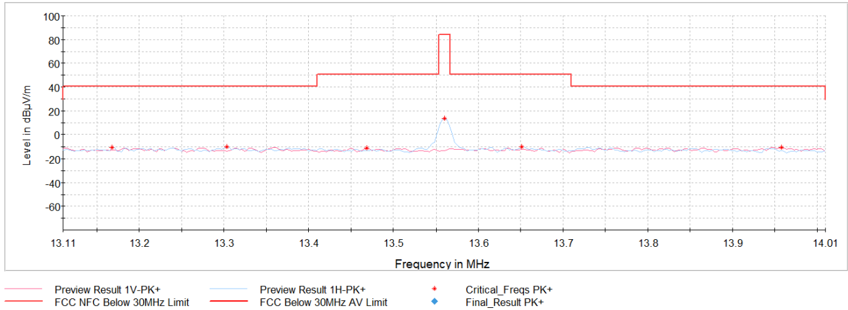
Plot 7-6. In Band Radiated Spurious Emissions (CE B 106kbps, with AC/DC Adapter and Magnetic Charger)
