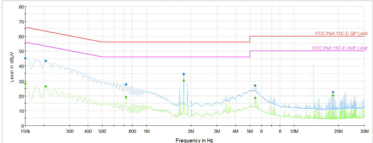
Plot 7-15. AC Line-Conducted Plot (N, Reader A 848kbps, with AC/DC Adapter and Magnetic Charger)
