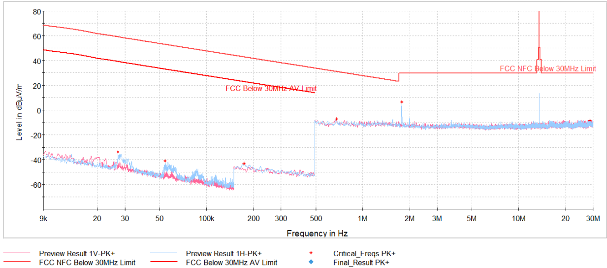
Plot 7-8. Radiated Spurious Emissions 9kHz – 30MHz (CE B 106 kbps, with AC/DC Adapter and Magnetic Charger)
