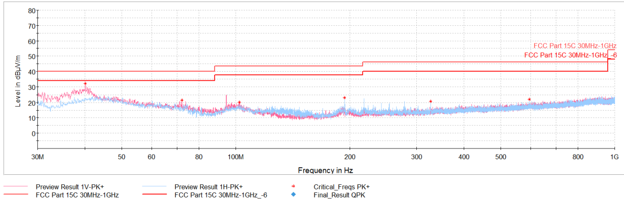
Plot 7-10. Radiated Spurious Emissions 30MHz – 1GHz (CE B 106kbps, with AC/DC Adapter and Magnetic Charger)
