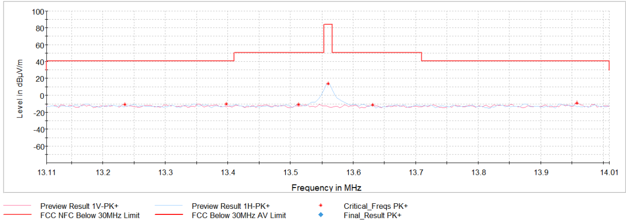
Plot 7-7. In Band Radiated Spurious Emissions (Reader A 848kbps, AC/DC Adapter and Magnetic Charger)
