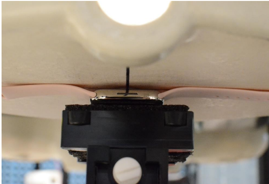
SAR Test Setup Photo 10: Stainless Steel with Sport Wristband, Extremity, Back Side at 0.0 cm
