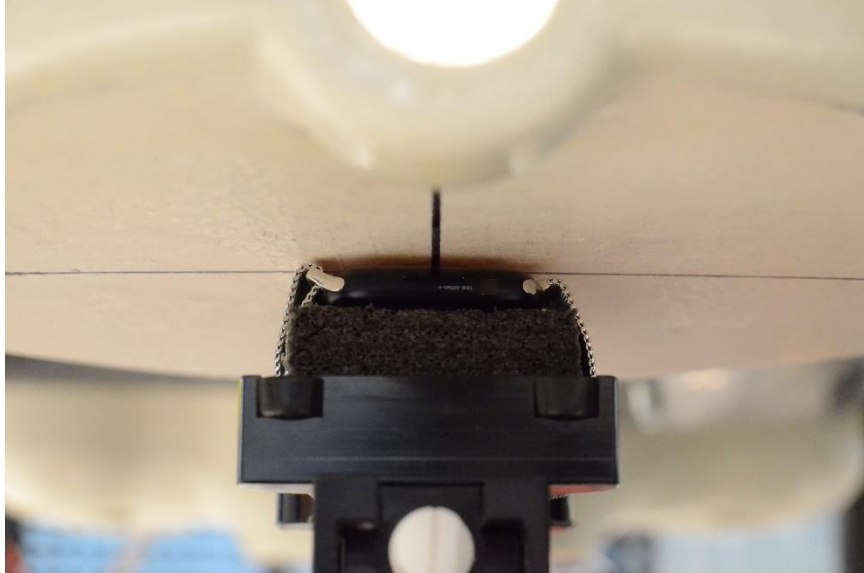
SAR Test Setup Photo 9: Aluminum with Metal Loop Wristband, Extremity, Back Side at 0.0 cm
