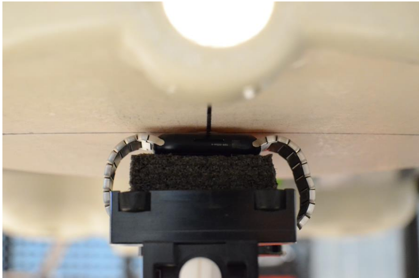
SAR Test Setup Photo 8: Aluminum with Metal Links Wristband, Extremity, Back Side at 0.0 cm
