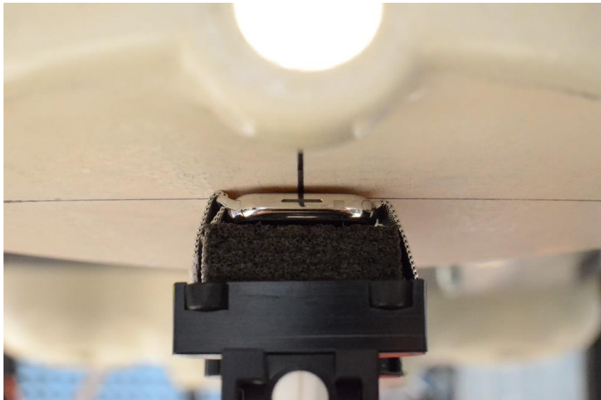
SAR Test Setup Photo 12: Stainless Steel with Metal Loop Wristband, Extremity, Back Side at 0.0 cm
