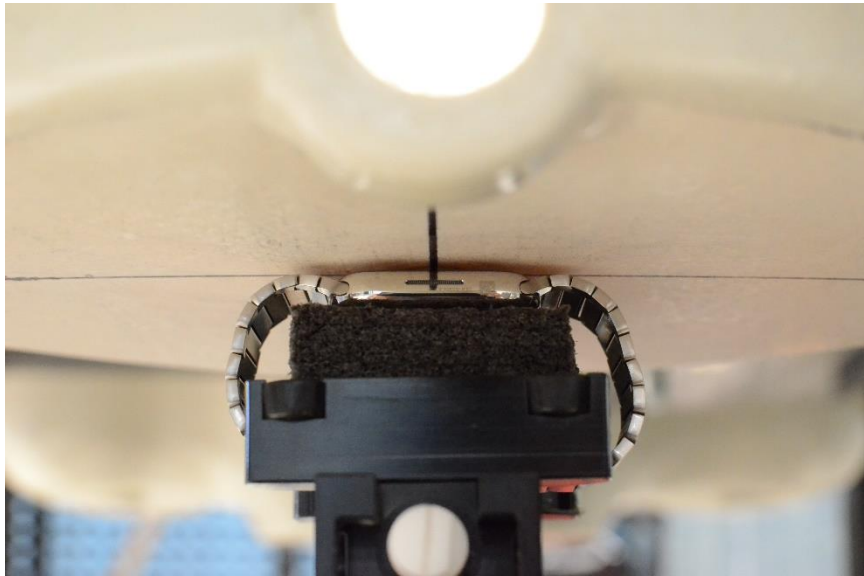
SAR Test Setup Photo 11: Stainless Steel with Metal Links Wristband, Extremity, Back Side at 0.0 cm
