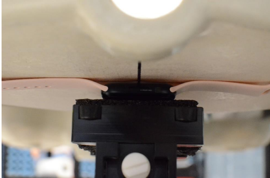
SAR Test Setup Photo 7: Aluminum with Sport Wristband, Extremity, Back Side at 0.0 cm
