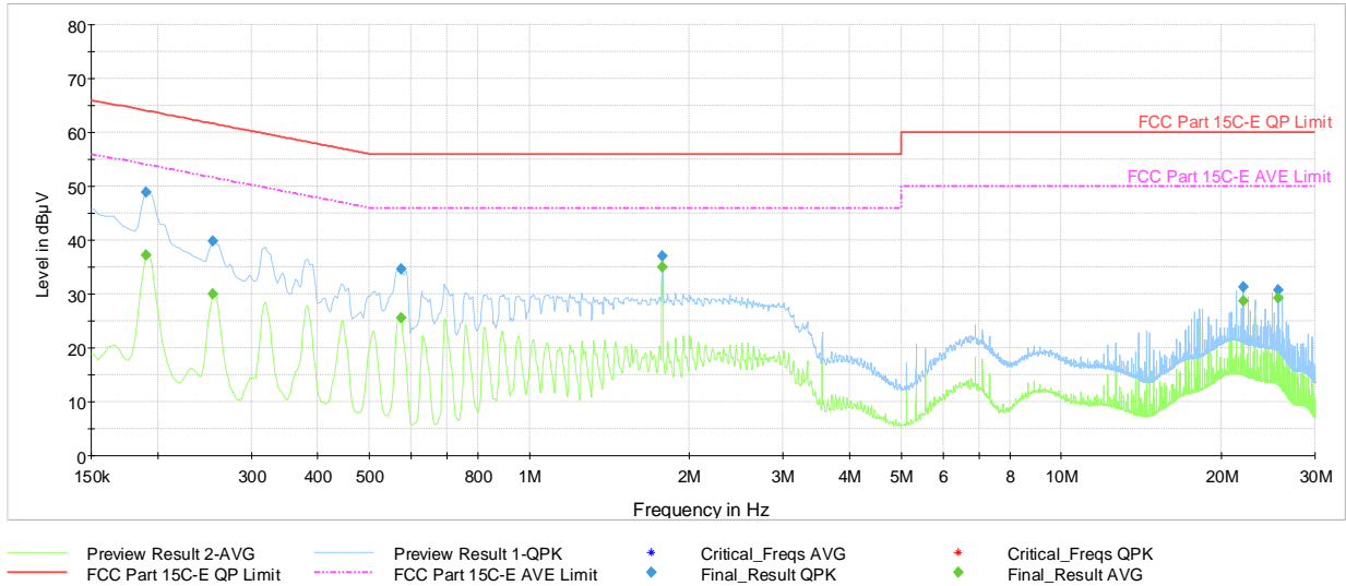
Plot 7-44. AC Line-Conducted Test Plot (N, GFSK ePA – Ch.39, with Laptop & magnetic charger)
