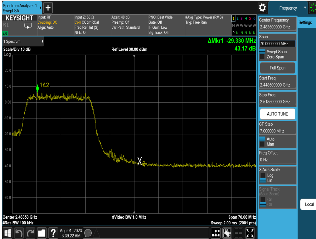
Plot 7-47. Band Edge Plot (802.11n (2.4GHz) – Ch. 11) – MCS7
