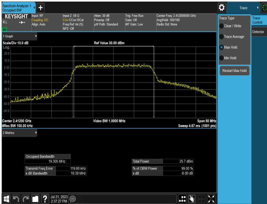
Plot 7-10. 6dB Bandwidth Plot (802.11n (2.4GHz) - Ch. 1) - MCS7
