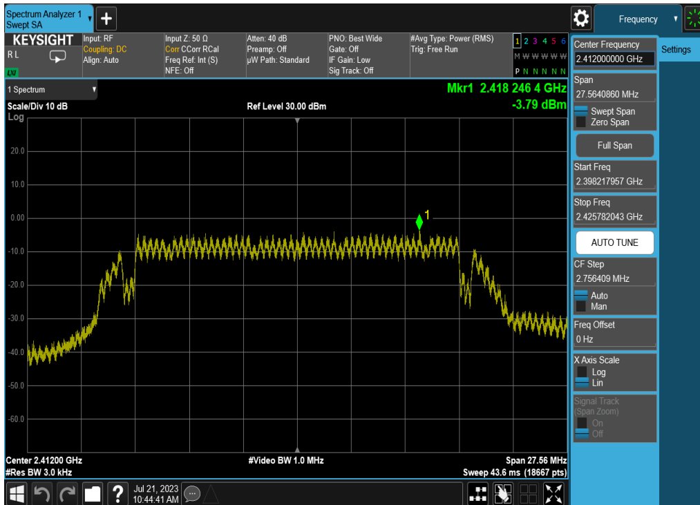
Plot 7-16. Power Spectral Density Plot (802.11g – Ch. 1) – 6Mbps
