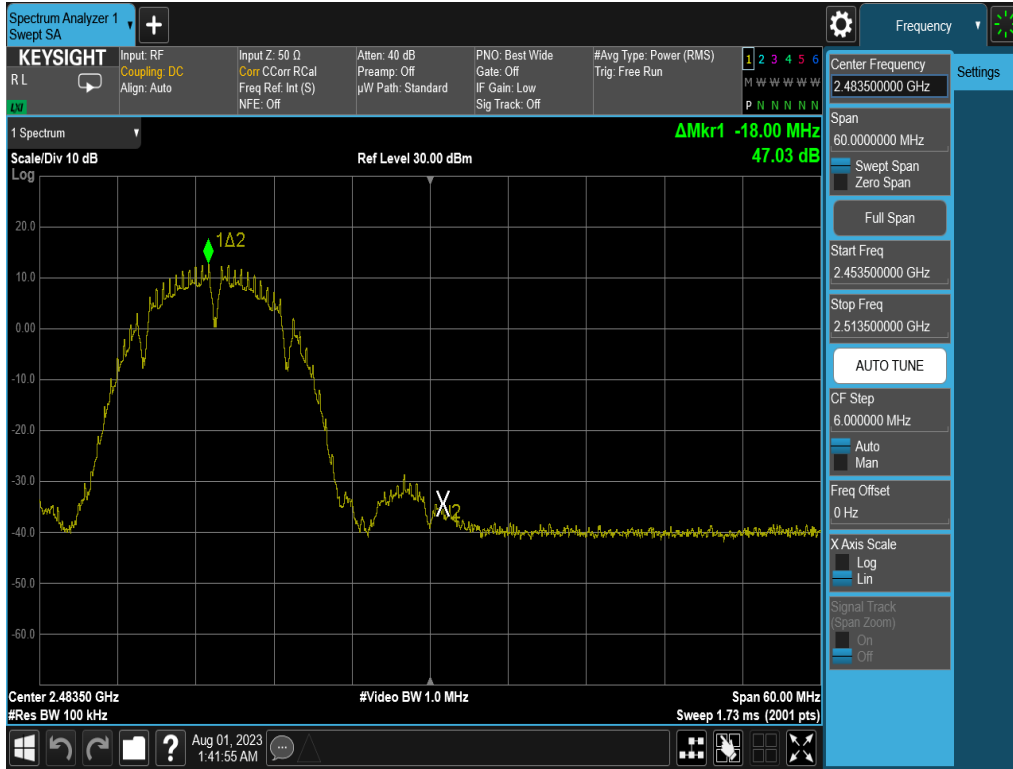
Plot 7-27. Band Edge Plot (802.11b– Ch. 12)
