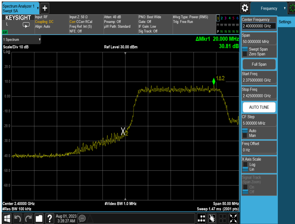
Plot 7-45. Band Edge Plot (802.11n (2.4GHz) – Ch. 1) – MCS7
