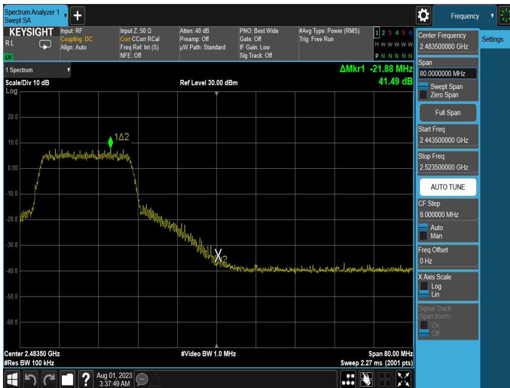
Plot 7-46. Band Edge Plot (802.11n (2.4GHz) – Ch. 10) – MCS7
