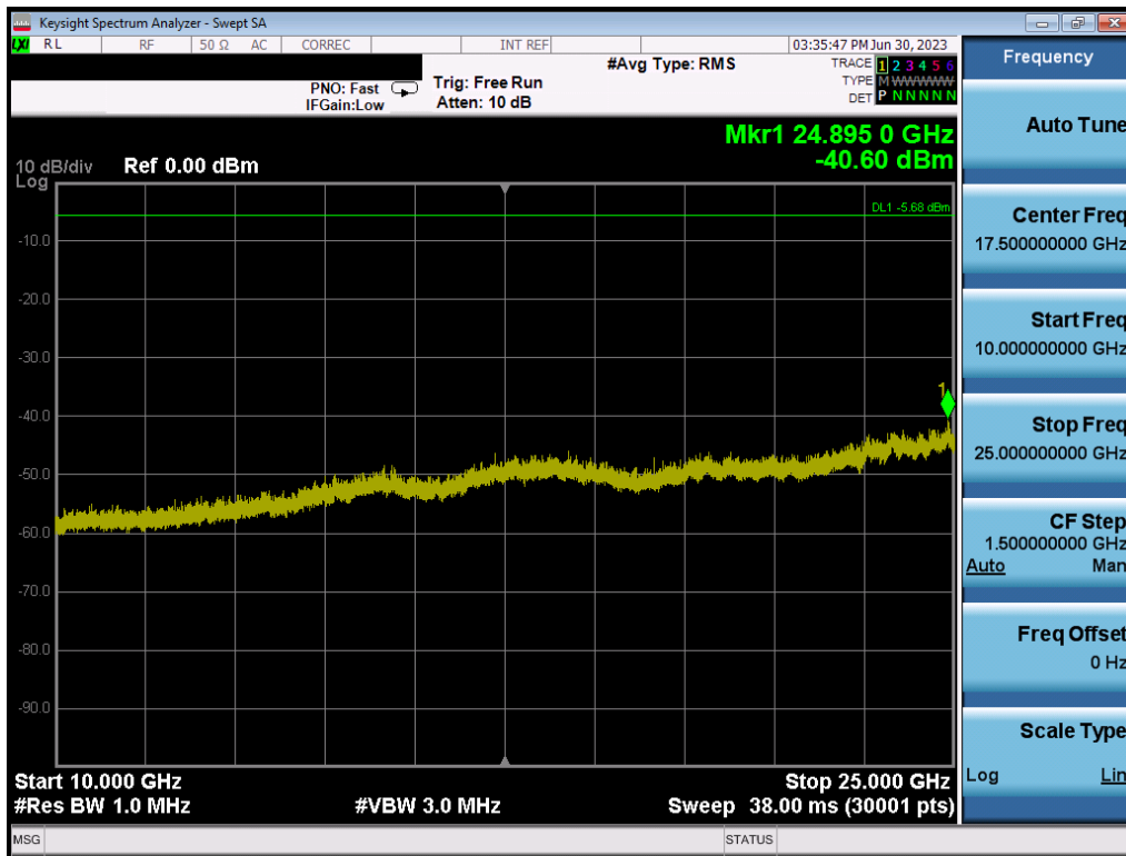
Plot 7-53. Conducted Spurious Plot (802.11b – Ch. 6)
