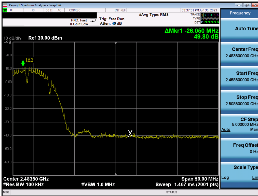
Plot 7-28. Band Edge Plot (802.11b– Ch. 13)
