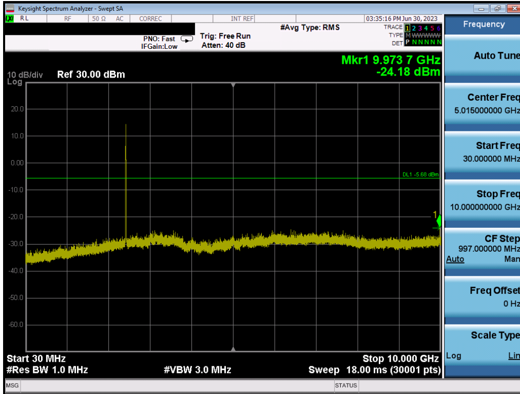
Plot 7-52. Conducted Spurious Plot (802.11b – Ch. 6)
