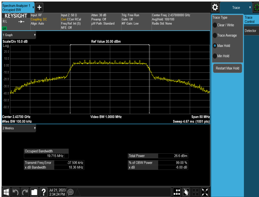
Plot 7-8. 6dB Bandwidth Plot (802.11n (2.4GHz) – Ch. 6) – MCS0
