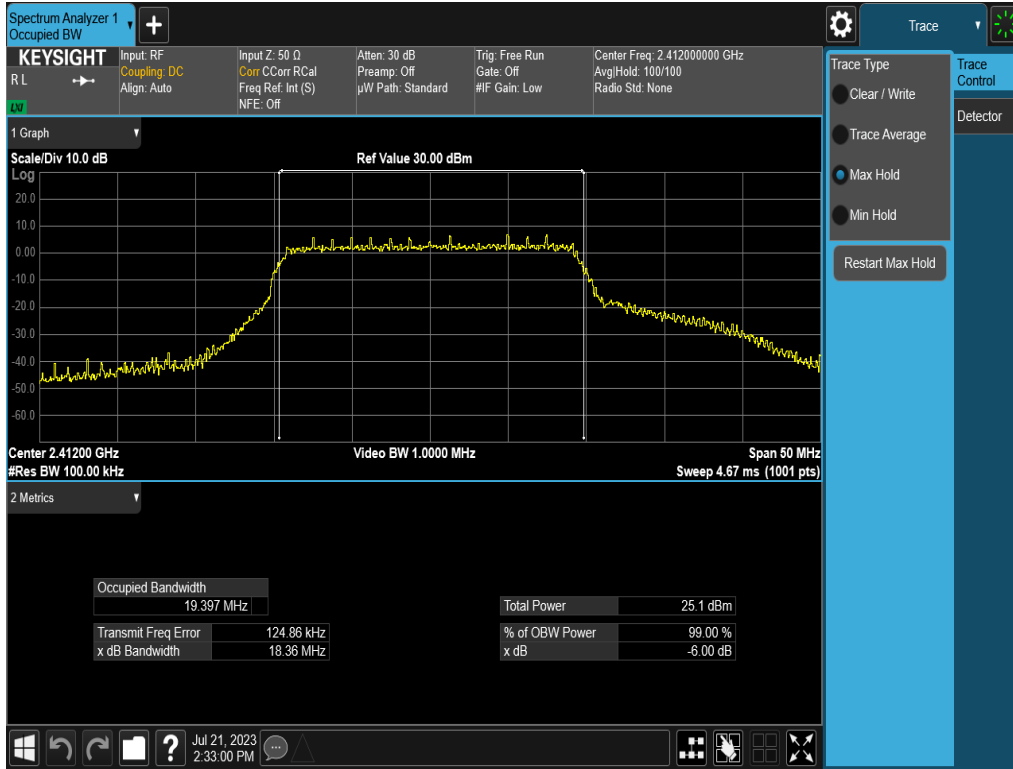
Plot 7-7. 6dB Bandwidth Plot (802.11n (2.4GHz) – Ch. 1) – MCS0
