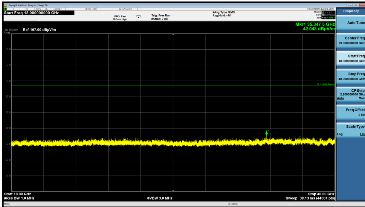
Plot 7-60. Radiated Spurious Plot Above 18GHz (802.11b – Ch. 6 Pol V)
