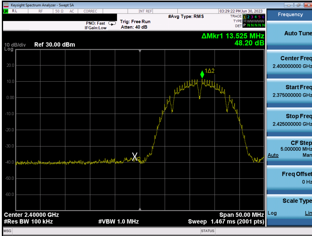
Plot 7-25. Band Edge Plot (802.11b- Ch. 1)
