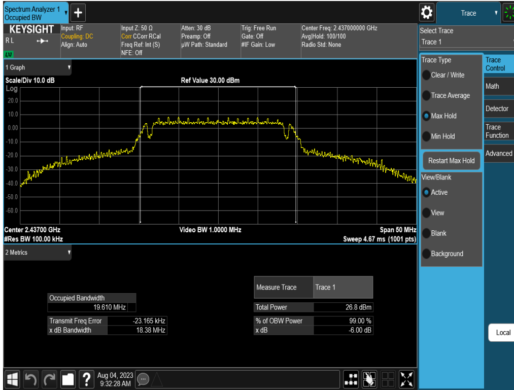
Plot 7-5. 6dB Bandwidth Plot (802.11g – Ch. 6) – 6Mbps
