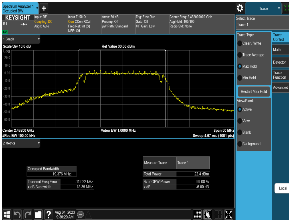
Plot 7-6. 6dB Bandwidth Plot (802.11g – Ch. 11) – 6Mbps
