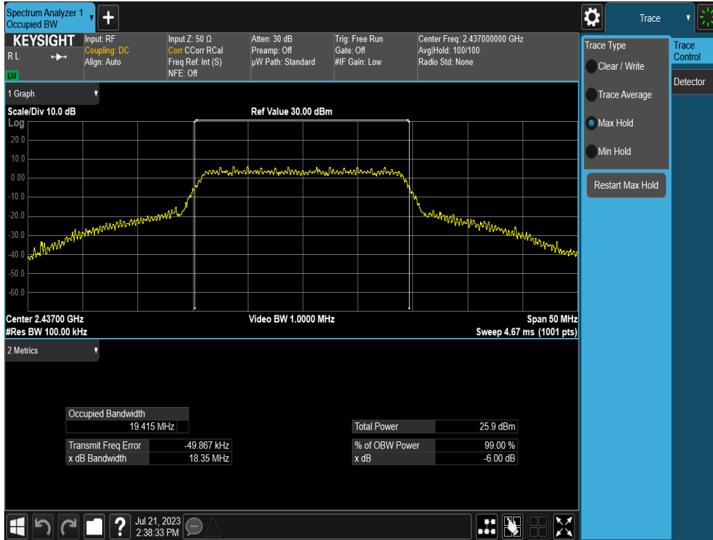
Plot 7-11. 6dB Bandwidth Plot (802.11n (2.4GHz) – Ch. 6) – MCS7
