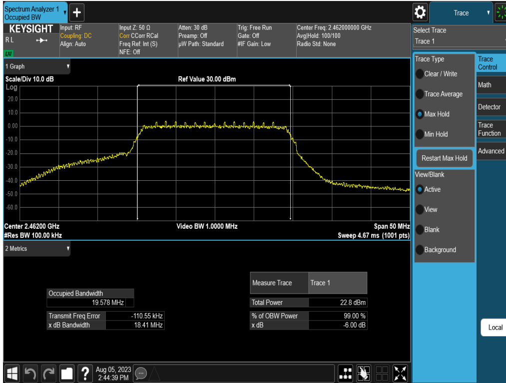
Plot 7-9. 6dB Bandwidth Plot (802.11n (2.4GHz) - Ch. 11) - MCS0
