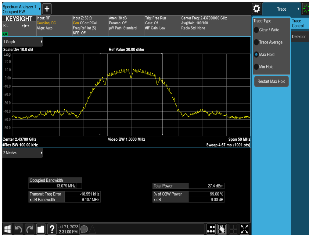
Plot 7-2. 6dB Bandwidth Plot (802.11b – Ch. 6) – 1Mbps
