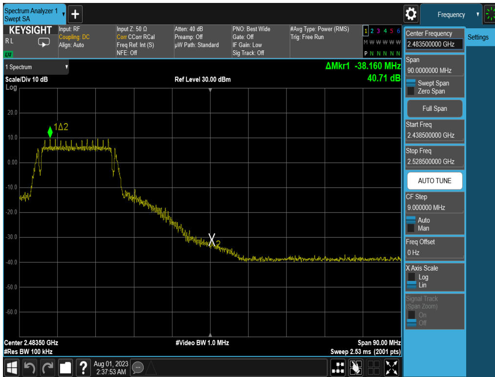
Plot 7-32. Band Edge Plot (802.11g – Ch. 9)
