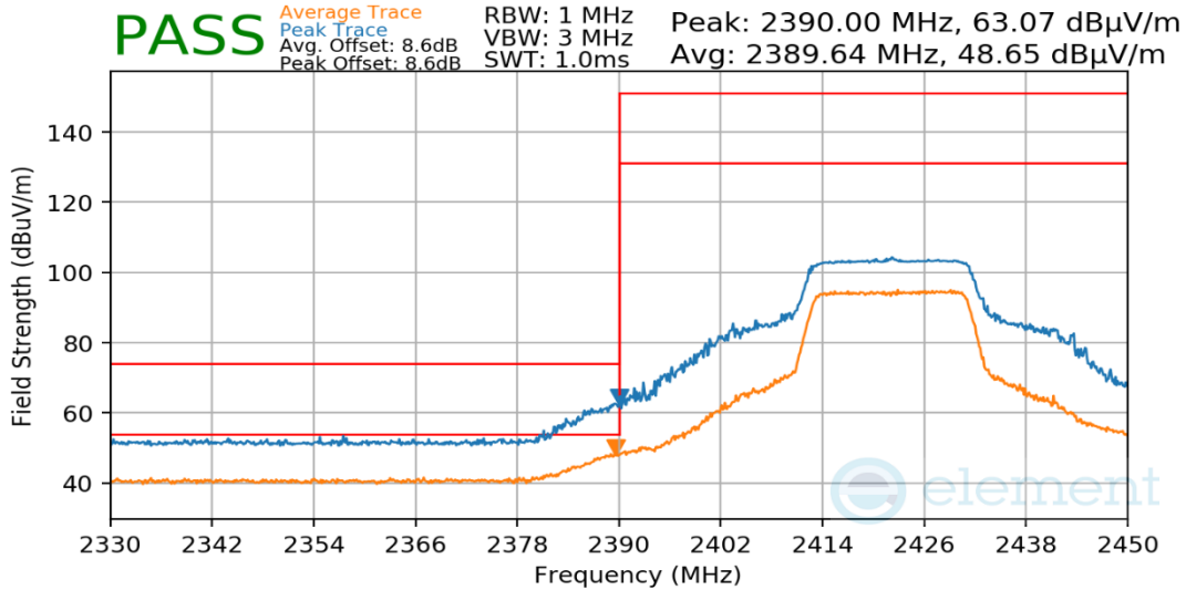
Plot 7-67. Radiated Restricted Lower Band Edge Measurement
