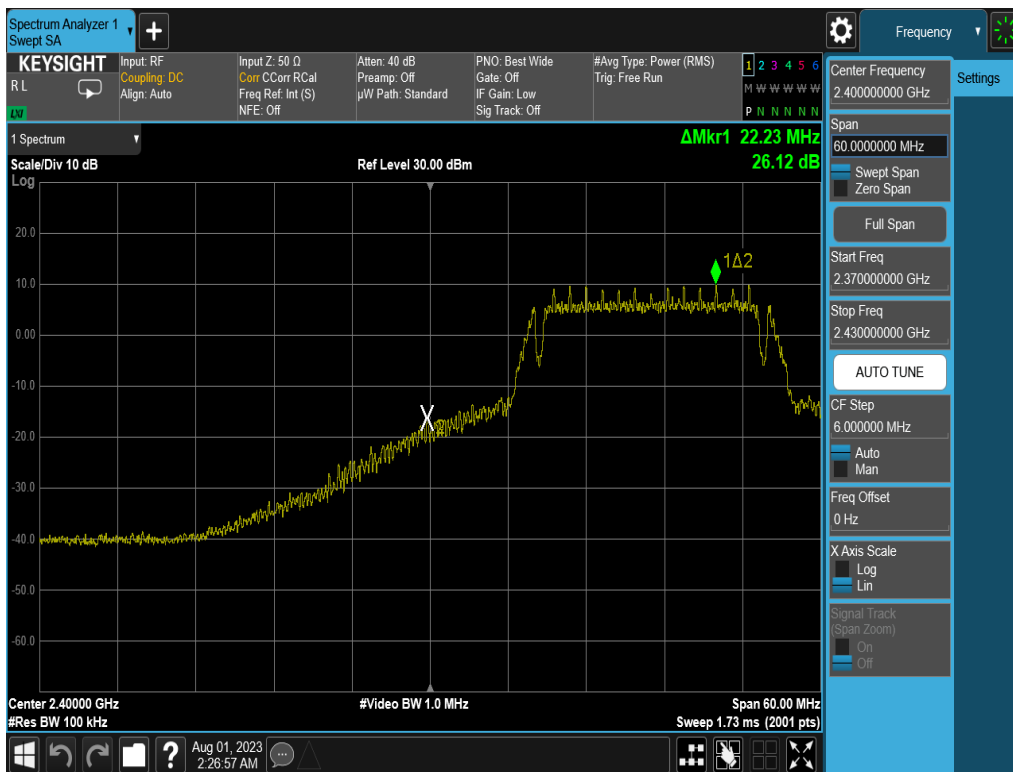
Plot 7-30. Band Edge Plot (802.11g- Ch. 2)
