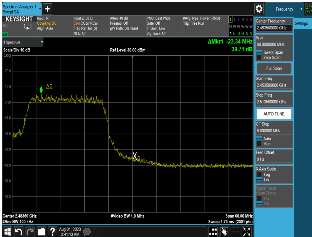
Plot 7-48. Band Edge Plot (802.11n (2.4GHz) – Ch. 12) – MCS7
