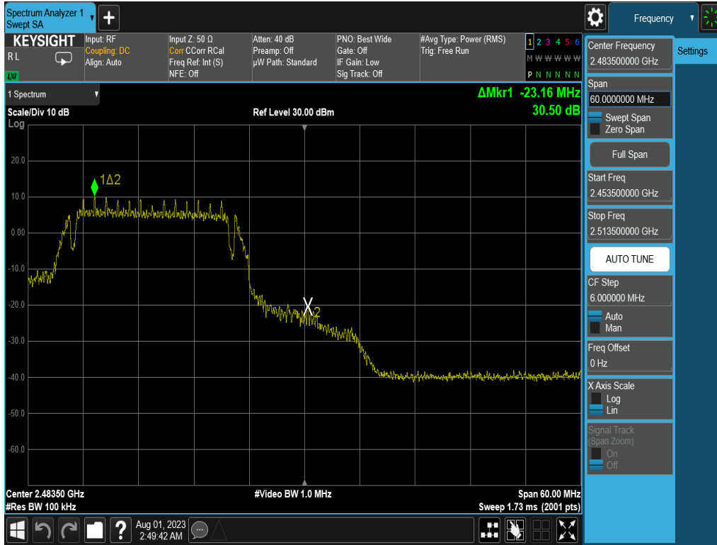
Plot 7-35. Band Edge Plot (802.11g – Ch. 12)
