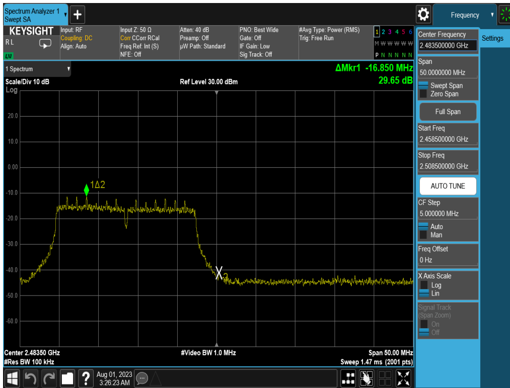
Plot 7-44. Band Edge Plot (802.11n (2.4GHz) – Ch. 13) – MCS0
