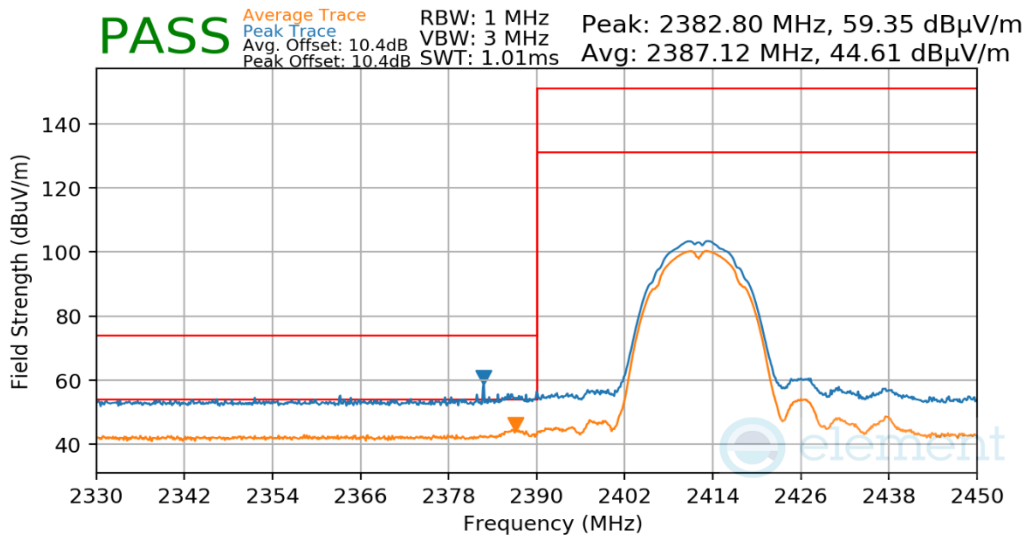
Plot 7-61. Radiated Restricted Lower Band Edge Measurement
