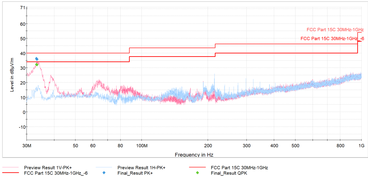
Plot 7-38. Radiated Spurious Emissions Below 1GHz (1Mbps, ePA – Ch.19, Pol. H & V, with AC/DC Adapter + Magnetic Charger)
