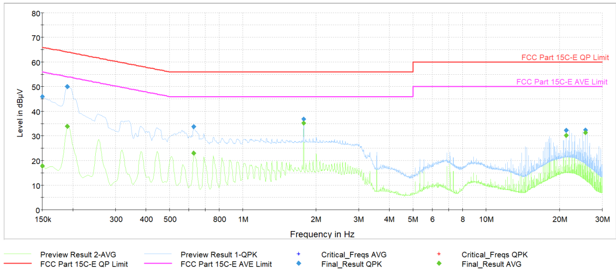
Plot 7-40. AC Line Conducted Plot with Bluetooth LE (N, 1Mbps ePA – Ch.19 with Laptop + Magnetic Charger)
