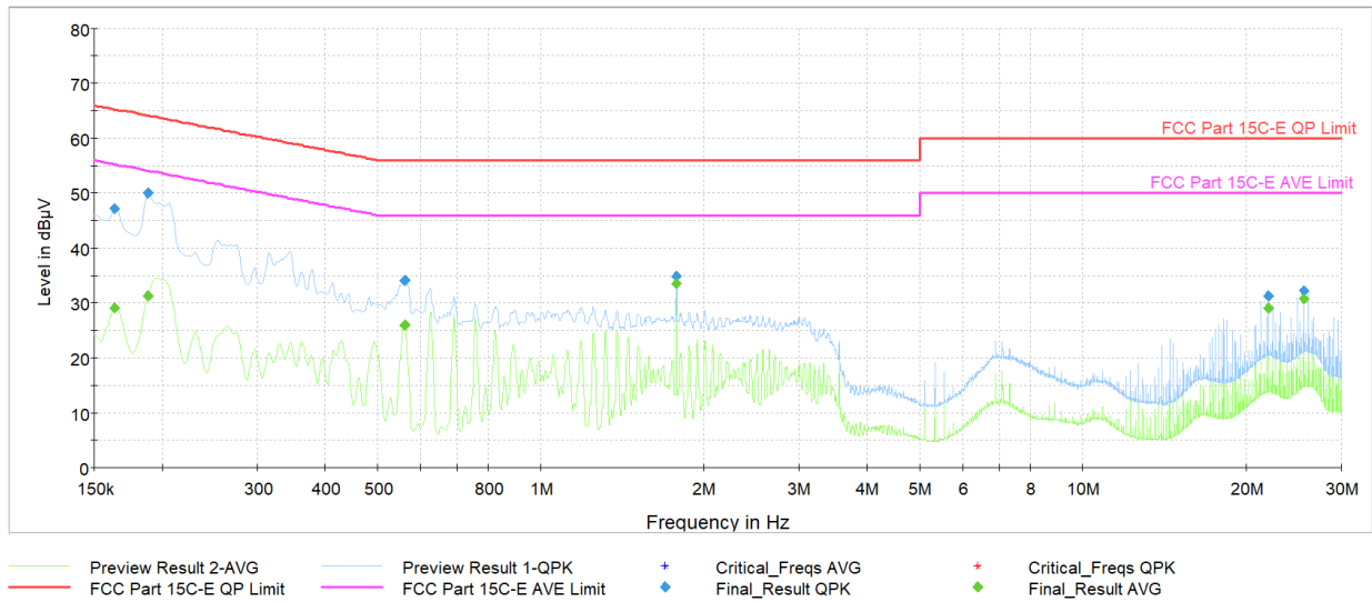
Plot 7-39. AC Line Conducted Plot with Bluetooth LE (L1, 1Mbps ePA – Ch.19 with Laptop + Magnetic Charger)
