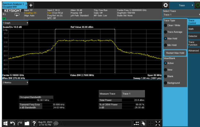
Plot 7-1. 26dB BW & 99% OBW (20MHz BW 802.11n – Ch. 36, MCS0)
