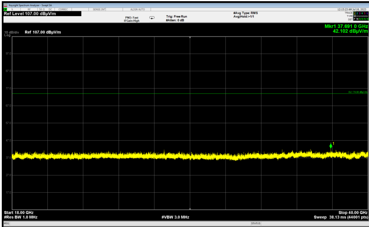
Plot 7-39. Radiated Spurious Emissions 18GHz-40GHz H Polarity (802.11n – Ch. 157)
