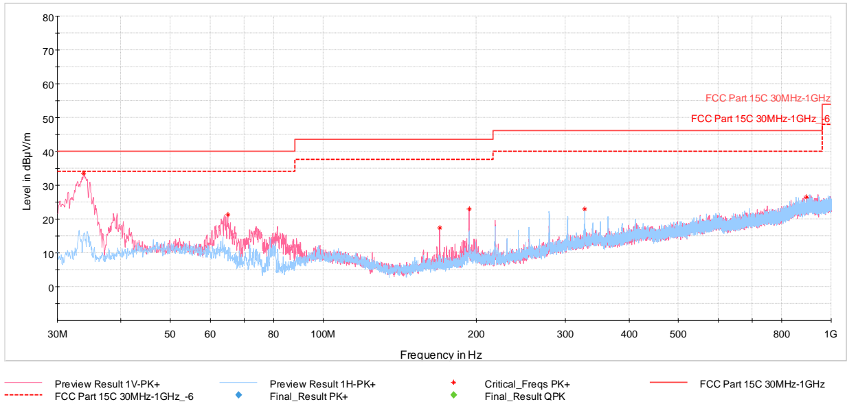
Plot 7-59. Radiated Spurious Emissions below 1GHz, 802.11n, Ch.165 with AC/DC Adapter & magnetic charger
