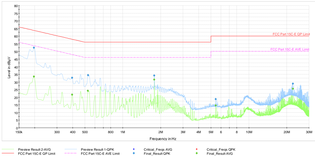
Plot 7-61. AC Line Conducted Plot with 802.11n – Ch.157 (L1), with host PC & magnetic charger
