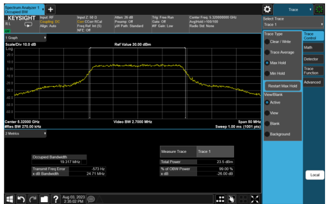
Plot 7-6. 26dB BW & 99% OBW (20MHz BW 802.11n – Ch. 64, MCS0)
