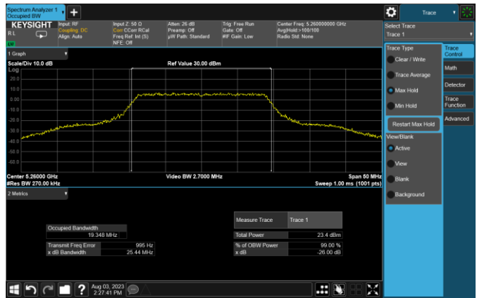
Plot 7-4. 26dB BW & 99% OBW (20MHz BW 802.11n – Ch. 52, MCS0)
