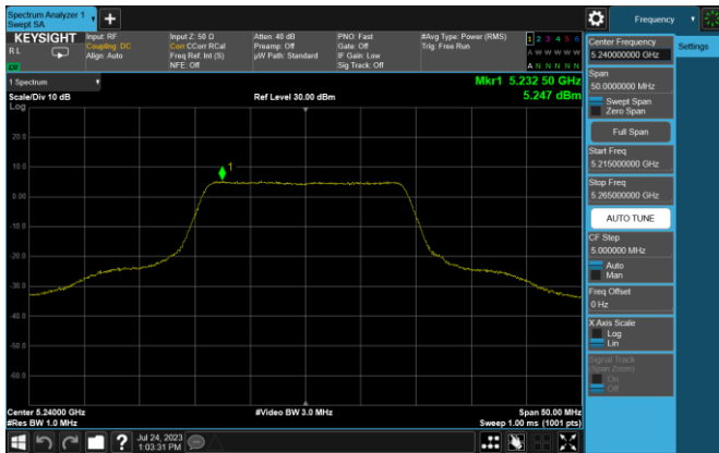
Plot 7-15. PSD (20MHz BW 802.11n - Ch. 48, MCS0)
