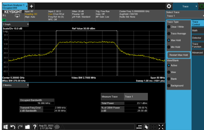
Plot 7-2. 26dB BW & 99% OBW (20MHz BW 802.11n – Ch. 40, MCS0)
