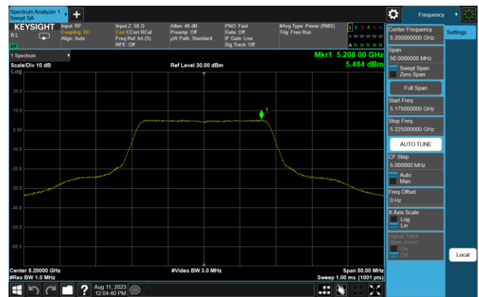
Plot 7-17. ISED PSD (20MHz BW 802.11n - Ch. 40, MCS0)
