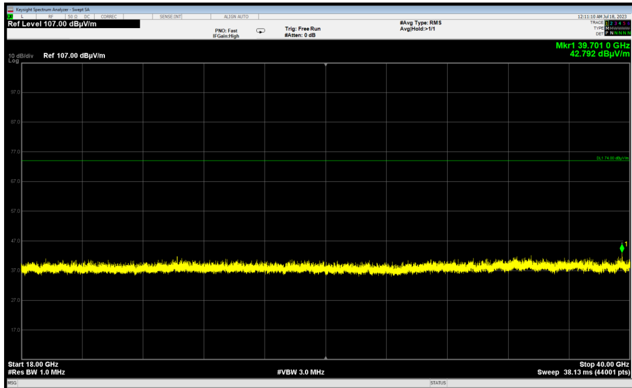
Plot 7-40. Radiated Spurious Emissions 18GHz-40GHz V Polarity (802.11n – Ch. 157)
