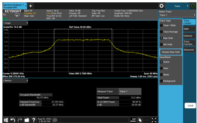
Plot 7-5. 26dB BW & 99% OBW (20MHz BW 802.11n – Ch. 56, MCS0)
