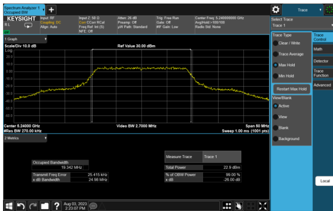
Plot 7-3. 26dB BW & 99% OBW (20MHz BW 802.11n – Ch. 48, MCS0)
