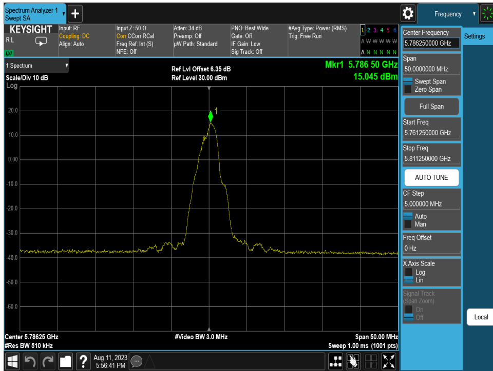
Plot 7-17. PSD (OQPSK, 5786.25MHz, 100kbps)
