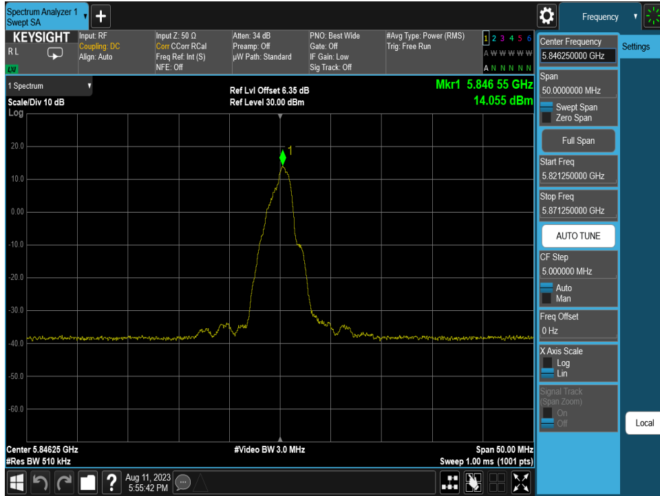
Plot 7-18. PSD (OQPSK, 5846.25MHz, 100kbps)
