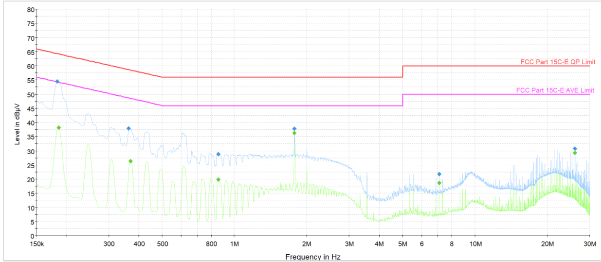
Plot 7-31. AC Line Conducted Plot (OQPSK – Ch. 24) (L1) with Laptop & Magnetic charger
