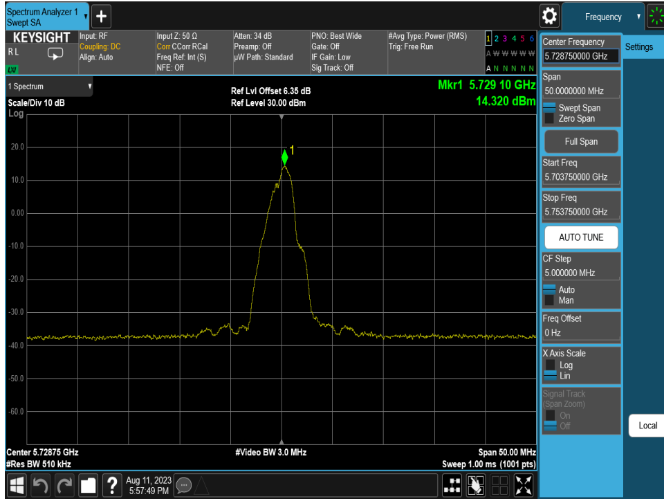
Plot 7-16. PSD (OQPSK, 5728.75MHz, 100kbps)
