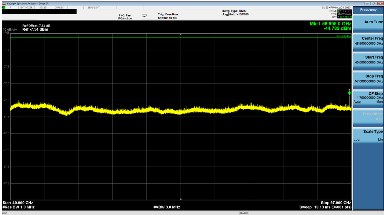
Plot 6-5. Radiated Spurious Emissions 40GHz – 57GHz (Mode 1)
