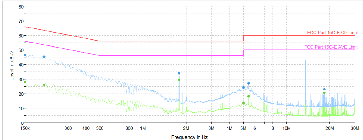
Plot 7-13. AC Line-Conducted Plot (N, CE B 106kbps, with AC/DC Adapter and Magnetic Charger)
