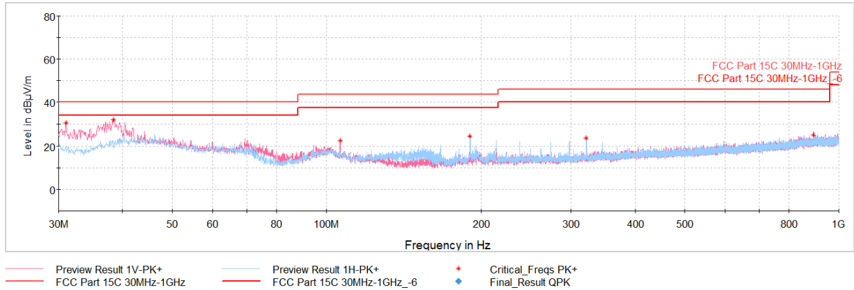
Plot 7-10. Radiated Spurious Emissions 30MHz – 1GHz (CE B 106kbps, with AC/DC Adapter and Magnetic Charger)
