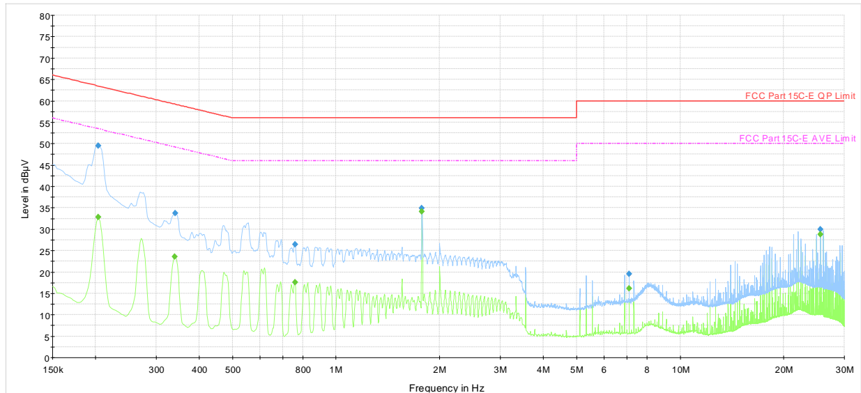
Plot 7-44. AC Line-Conducted Test Plot (N, GFSK ePA – Ch.0, with Laptop)
