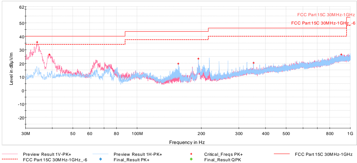
Plot 7-41. Radiated Spurious Emissions Below 1GHz (GFSK ePA – Ch.0, with AC/DC Adapter & Magnet Charger)
