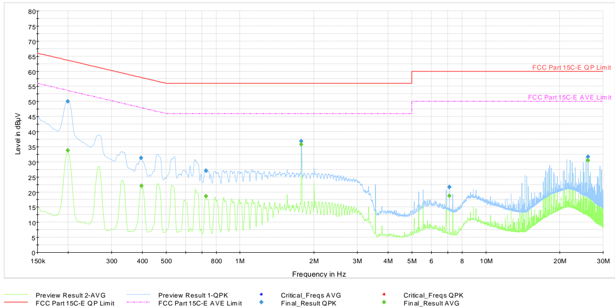
Plot 7-43. AC Line-Conducted Test Plot (L1, GFSK ePA – Ch.0, with Laptop)
