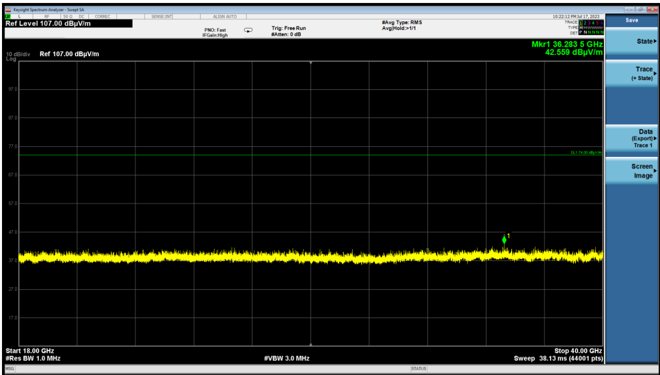
Plot 7-39. Radiated Spurious Emissions 18GHz-40GHz V Polarity (802.11n – Ch. 149)
