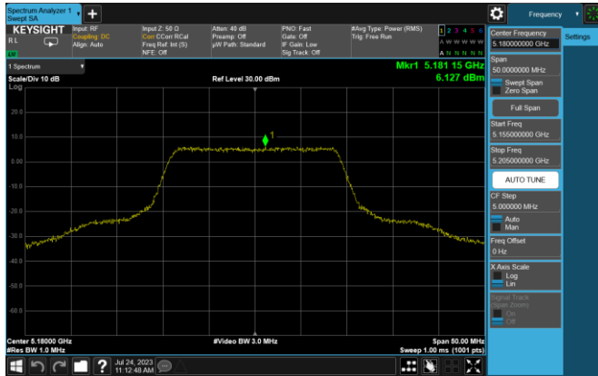
Plot 7-13. PSD (20MHz BW 802.11n – Ch. 36, MCS0)
