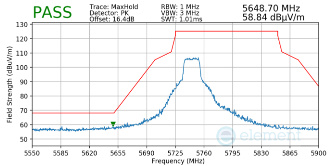
Plot 7-56. (Pk, Ch.149, 802.11n, MCS7)
