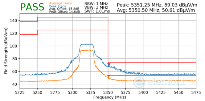
Plot 7-48. (Pk & Avg, Ch.64, 802.11n, MCS7)
