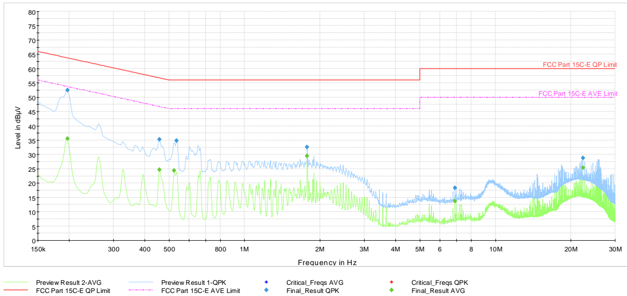
Plot 7-61. AC Line Conducted Plot with 802.11n – Ch.165 (L1), with Laptop & magnetic charger
