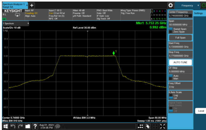
Plot 7-25. PSD (20MHz BW 802.11n – Ch. 149, MCS0)
