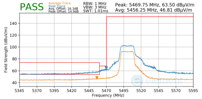
Plot 7-50. (Pk & Avg, Ch.100, 802.11n, MCS7)
