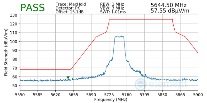
Plot 7-55. (Pk, Ch.149, 802.11n, MCS0)
