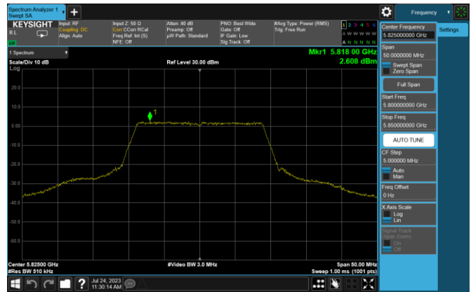
Plot 7-27. PSD (20MHz BW 802.11n – Ch. 165, MCS0)
