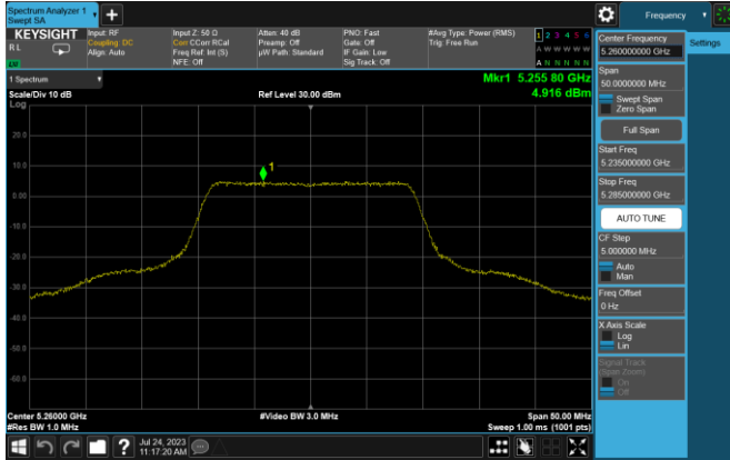
Plot 7-19. PSD (20MHz BW 802.11n – Ch. 52, MCS0)
