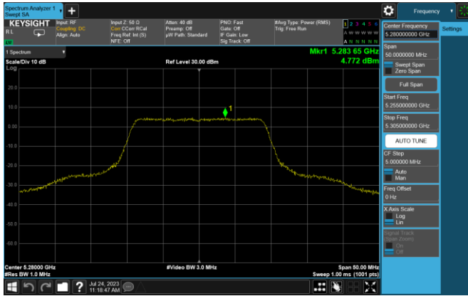
Plot 7-20. PSD (20MHz BW 802.11n – Ch. 56, MCS0)
