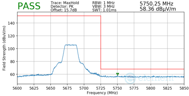
Plot 7-51. (Pk, Ch.136, 802.11n, MCS0)
