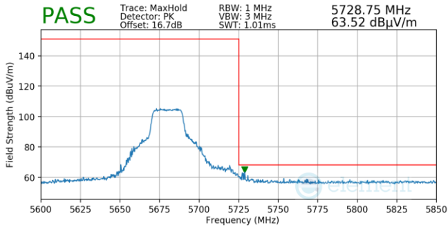
Plot 7-52. (Pk, Ch.136, 802.11n, MCS7)
