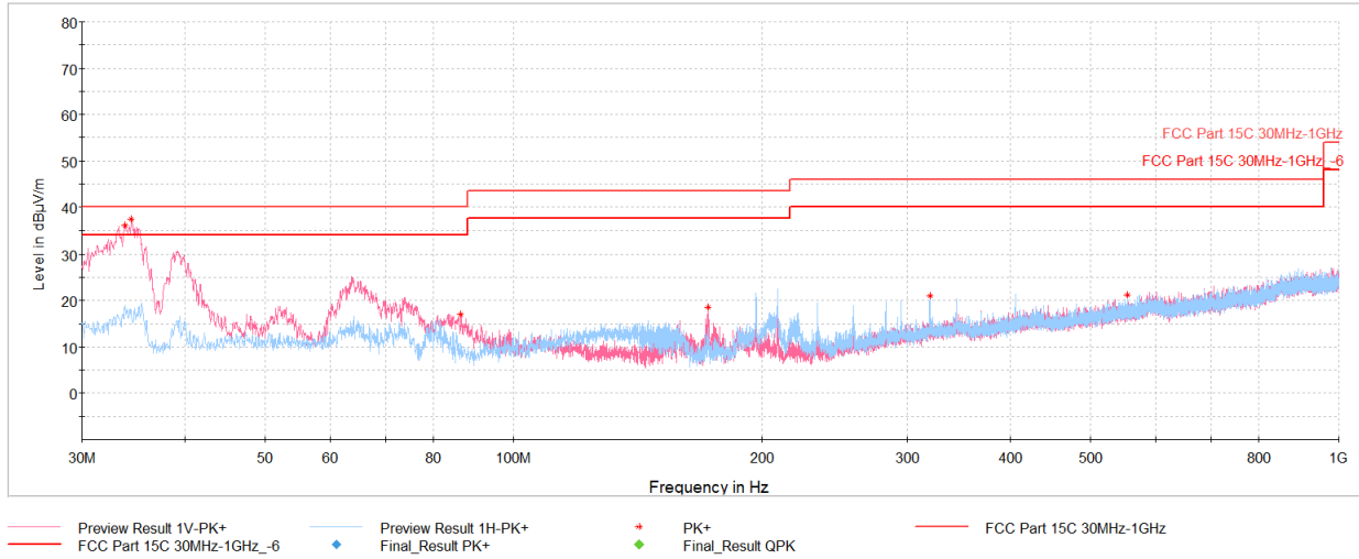
Plot 7-59. Radiated Spurious Emissions below 1GHz, 802.11n, Ch.165 with AC/DC Adapter & magnetic charger
