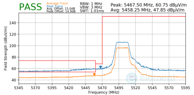
Plot 7-49. (Pk & Avg, Ch.100, 802.11n, MCS0)
