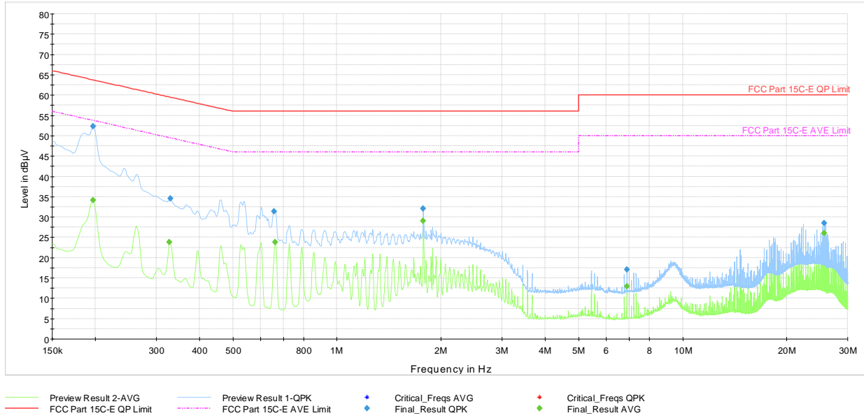
Plot 7-62. AC Line Conducted Plot with 802.11n– Ch.116 (N), with Laptop & magnetic charger
