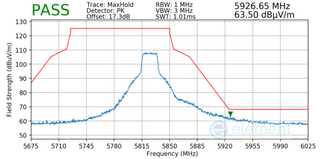
Plot 7-58. (Pk, Ch.165, 802.11n, MCS7)
