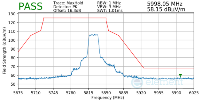
Plot 7-57. (Pk, Ch.165, 802.11n, MCS0)
