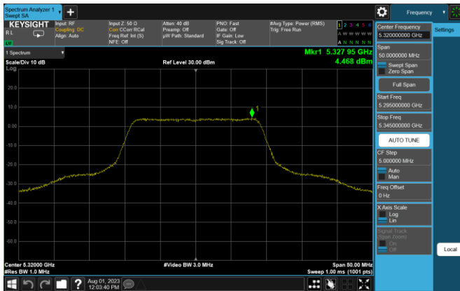
Plot 7-21. PSD (20MHz BW 802.11n – Ch. 64, MCS0)
