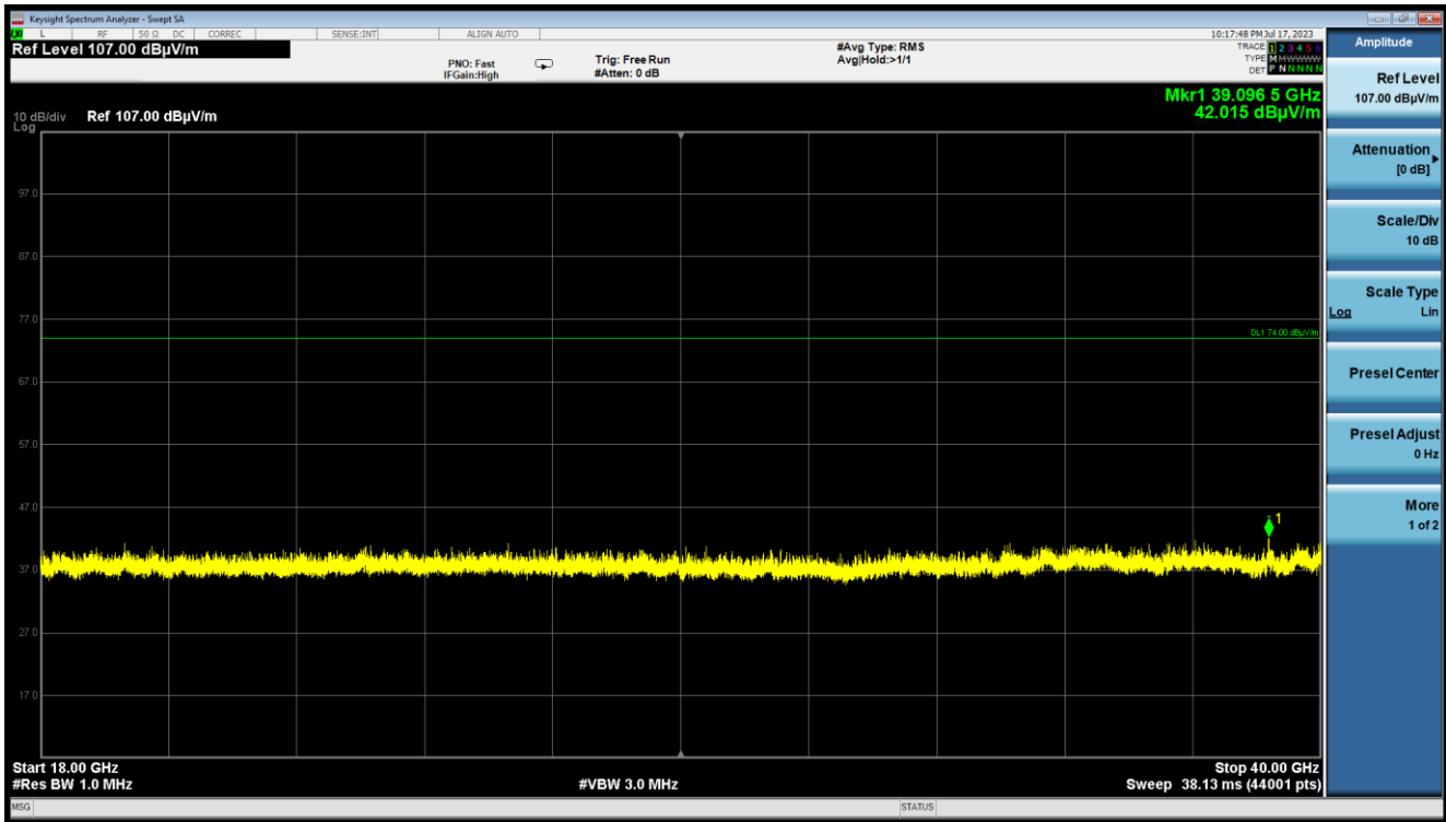
Plot 7-38. Radiated Spurious Emissions 18GHz-40GHz H Polarity (802.11n – Ch. 149)
