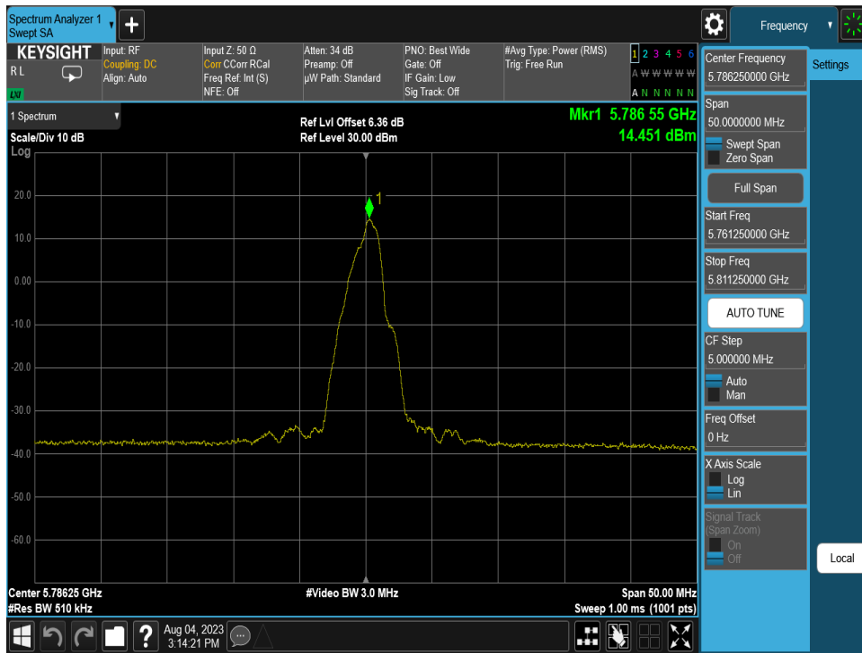
Plot 7-17. PSD (QPSK, 5786.25MHz, 1000kpbs)
