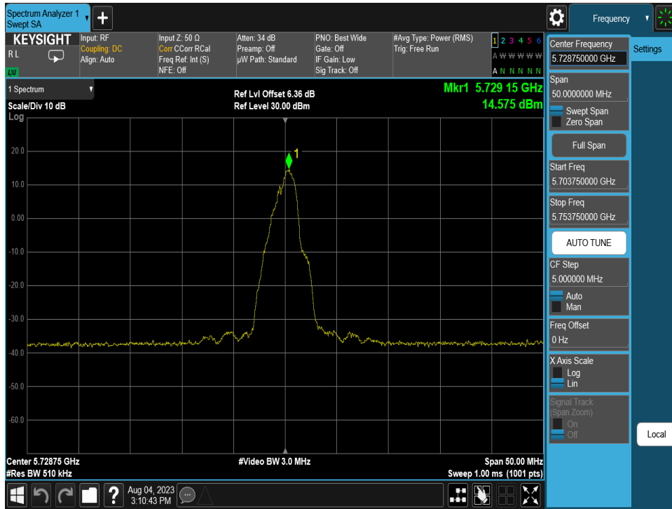
Plot 7-16. PSD (QPSK, 5728.75MHz, 1000kpbs)
