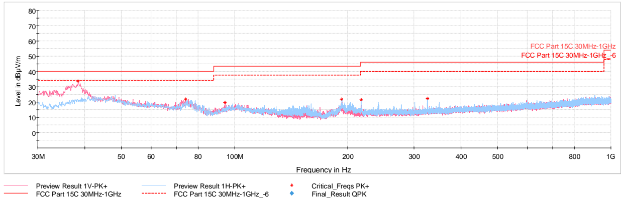
Plot 7-30. RSE 30MHz - 1GHz (OQPSK – Ch. 24), with AC/DC Adapter & magnetic charger
