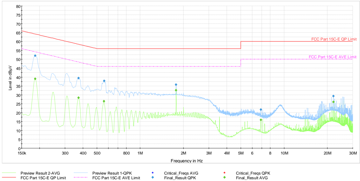
Plot 7-31. AC Line Conducted Plot (OQPSK – Ch. 24) (L1) with Laptop & magnetic charger
