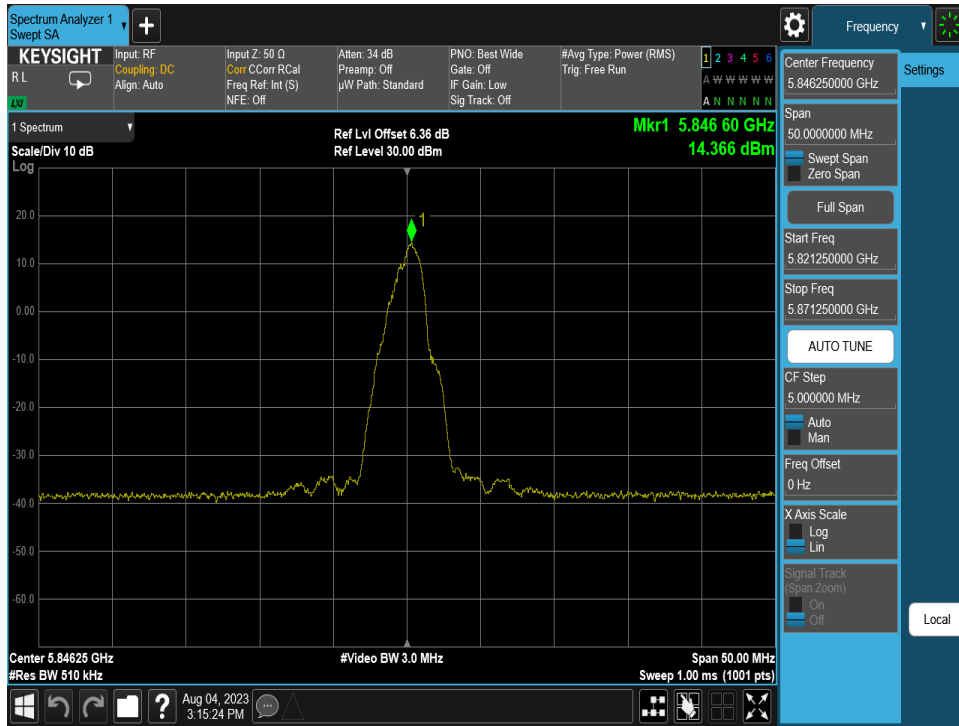
Plot 7-18. PSD (QPSK, 5846.25MHz, 100kbps)
