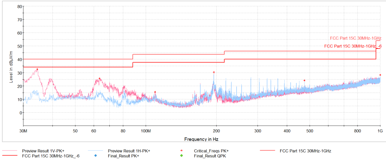
Plot 7-40. Radiated Co-Tx Spurious Emissions Below 1GHz (Pol. H & V, with AC/DC Adapter)
