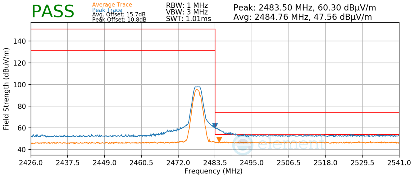
Plot 7-37. Radiated Restricted Upper Band Edge Measurement (Average & Peak)
