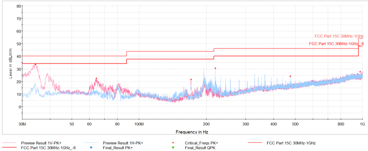
Plot 7-39. Radiated Spurious Simultaneous Transmission Emissions Below 1GHz (Pol. H & V, with AC/DC Adapter)
