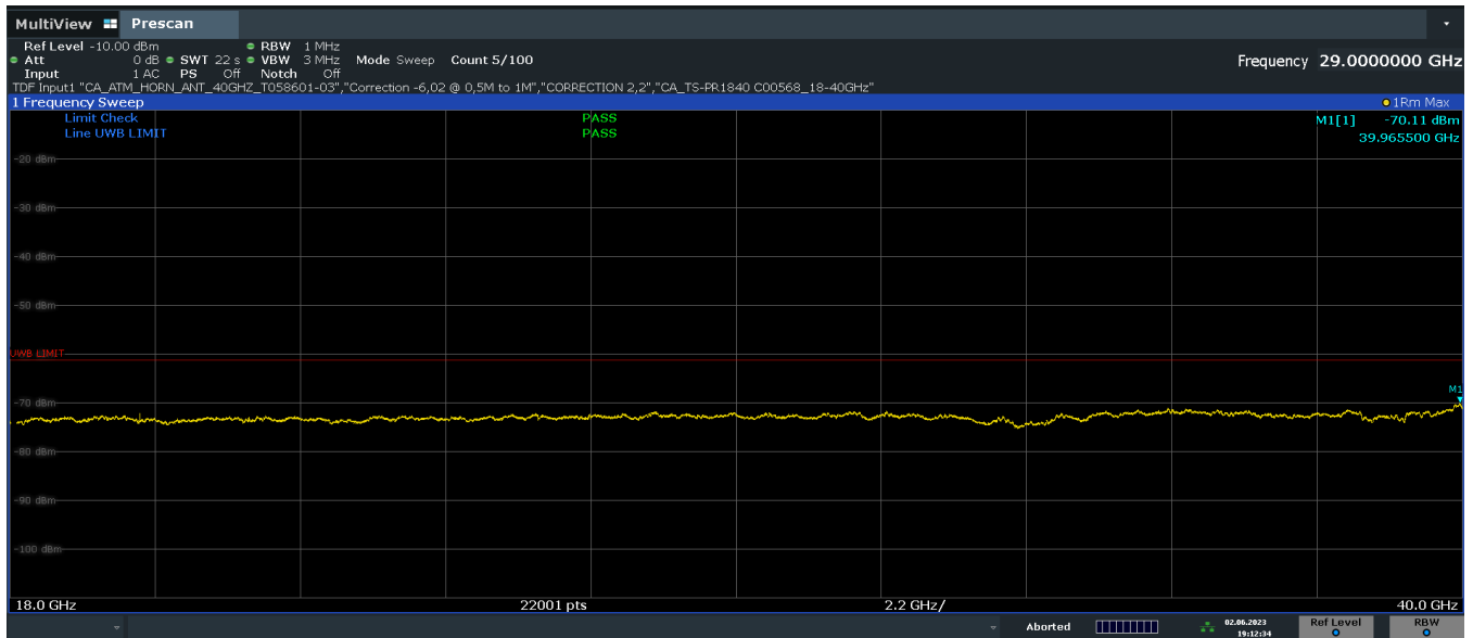
Plot 7-29. Radiated Spurious Simultaneous Transmission Above 18GHz V Polarity (1Mbps – Ch. 0)
