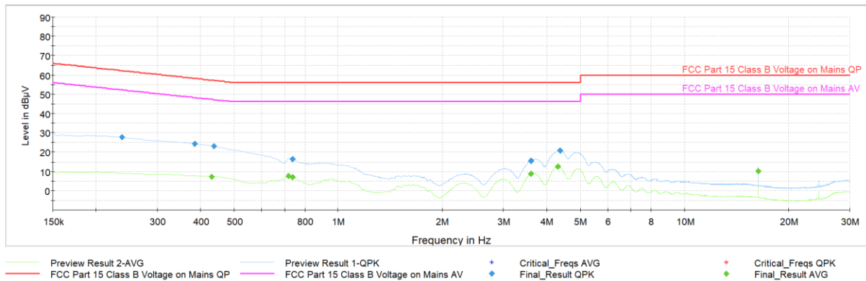
Plot 7-41. AC Line Conducted Plot with Bluetooth LE (L1, 1Mbps – Ch.19 with AC/DC Adapter)
