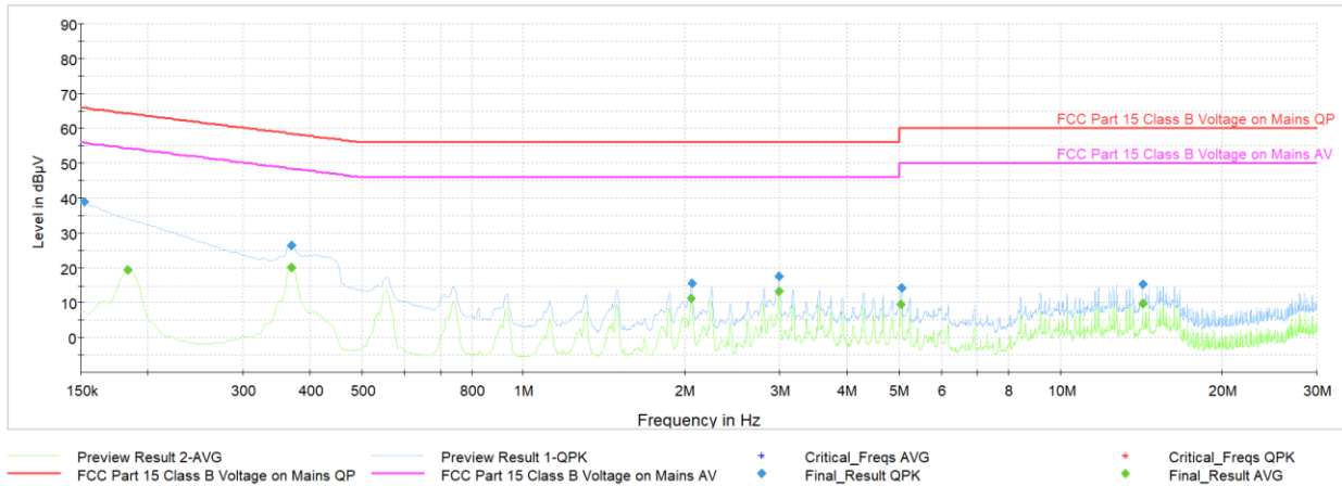
Plot 7-42. AC Line Conducted Plot with Bluetooth LE (N, 1Mbps – Ch.19, with Laptop and AC/DC Adapter)
