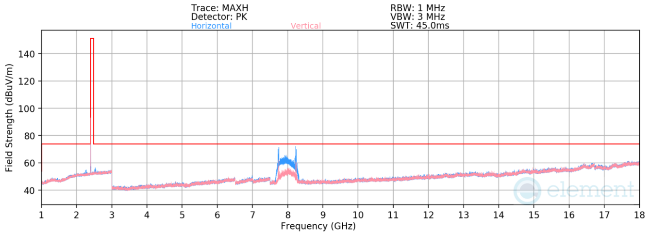
Plot 7-28. Radiated Spurious Simultaneous Transmission 1-18GHz
