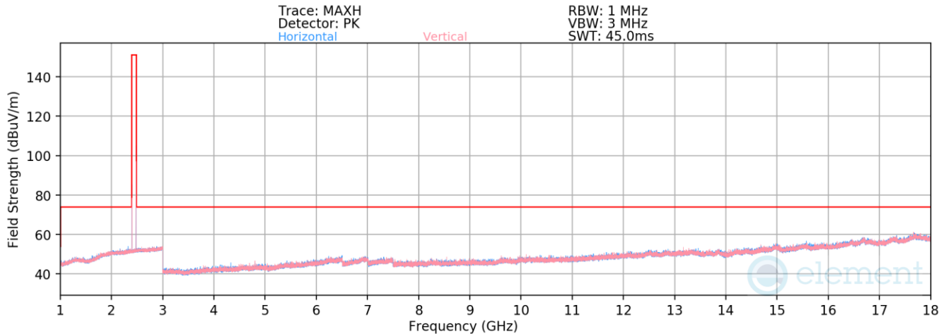
Plot 7-31. Radiated Spurious Emission – Co-Tx 1-18GHz
