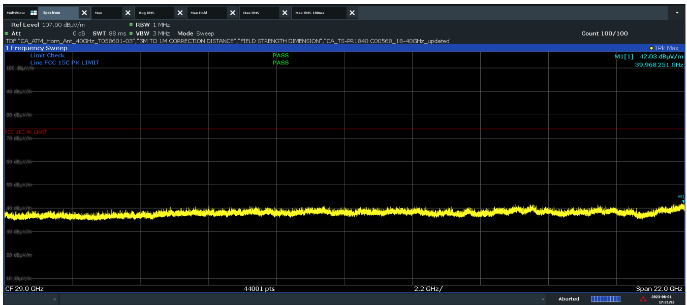
Plot 7-27. Radiated Spurious Emissions Above 18GHz H Polarity (1Mbps – Ch. 19)
