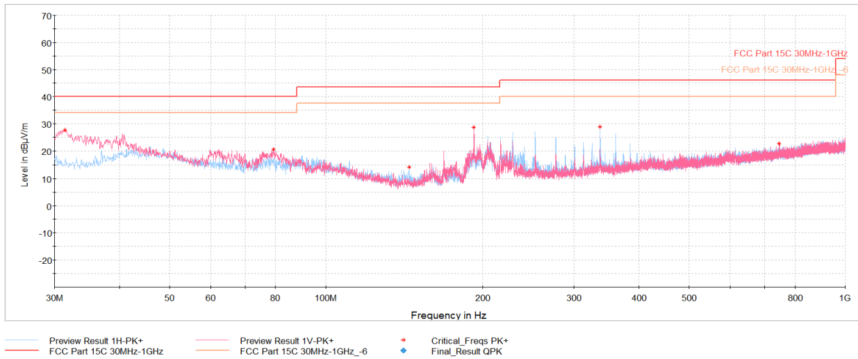
Plot 7-38. Radiated Spurious Emissions Below 1GHz (1Mbps – Ch.19, Pol. H & V, with AC/DC Adapter)
