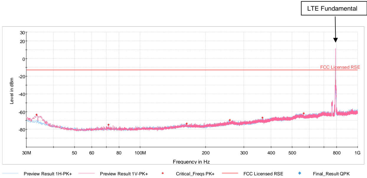
Plot 7-48. Antenna BCM Radiated Spurious Plot below 1GHz (LTE Band 14)
