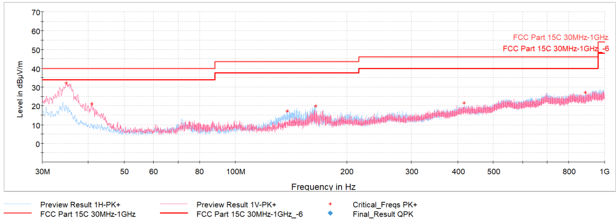
Plot 7-38. Radiated Spurious Emissions Below 1GHz (1Mbps, ePA – Ch.19, Pol. H & V, with AC/DC Adapter + Magnetic Charger)
