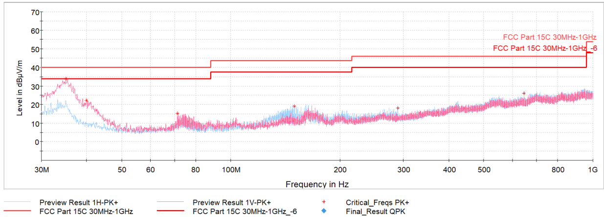
Plot 7-38. Radiated Spurious Emissions Below 1GHz (HDR4 ePA – Ch.38 with AC/DC Adapter + Magnetic Charger)
