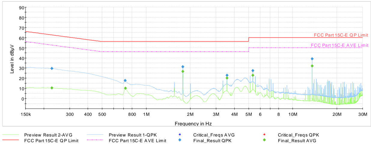
Plot 7-15. AC Line-Conducted Plot (N, Reader A 848kbps, with Laptop and Magnetic Charger)
