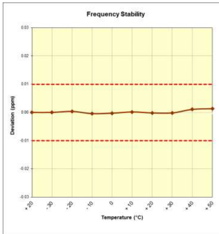
Figure 7-4. Frequency Stability Plot (Reader 10% ASK 1 out of 256)
