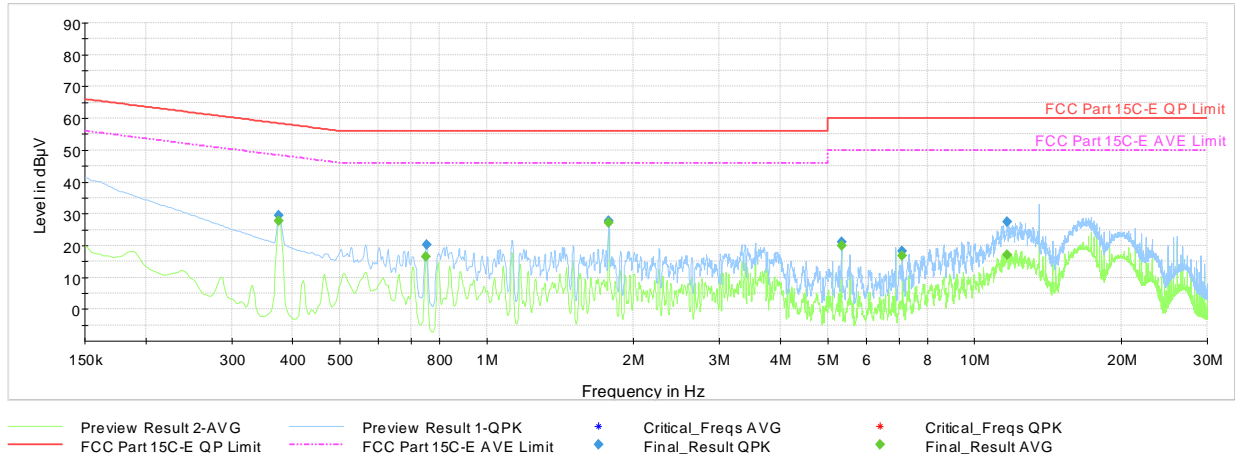
Plot 7-12. AC Line-Conducted Plot (L1, CE B 106kbps, with Laptop and Magnetic Charger)
