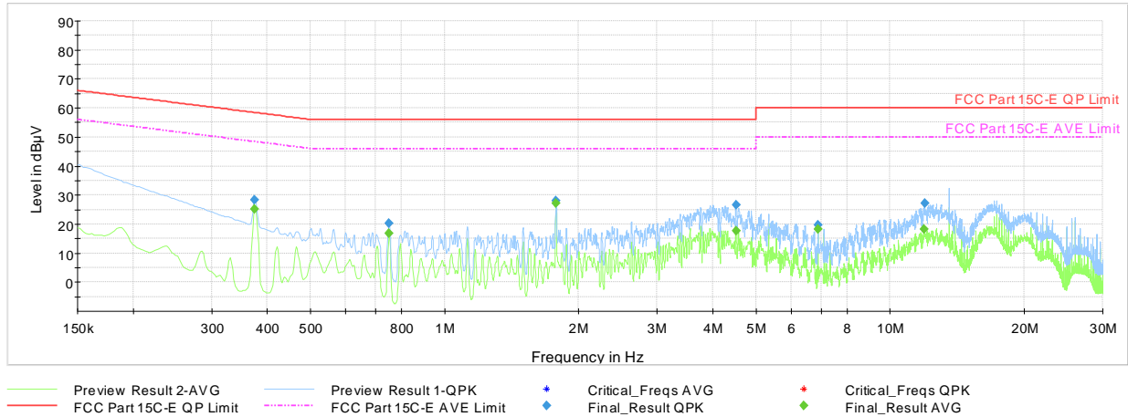
Plot 7-13. AC Line-Conducted Plot (N, CE B 106kbps, with Laptop and Magnetic Charger)
