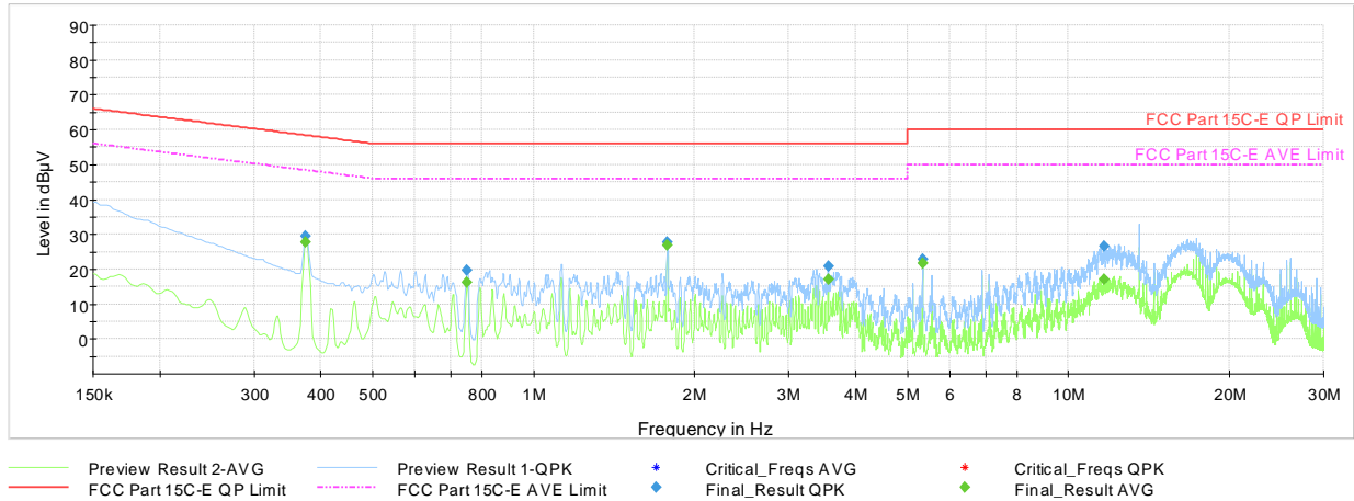
Plot 7-14. AC Line-Conducted Plot (L1, Reader A 848kbps, with Laptop and Magnetic Charger)
