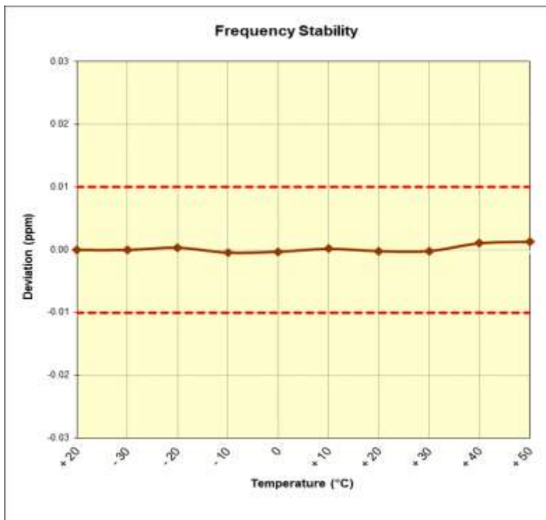
Figure 7-3. Frequency Stability Plot (CE B 106kbps)
