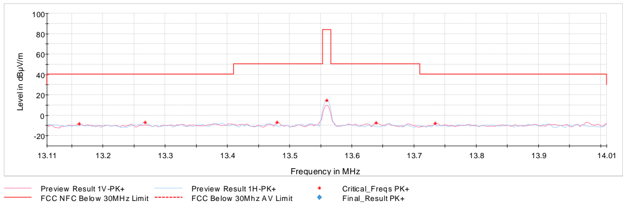
Plot 7-6. In Band Radiated Spurious Emissions (CE B 106kbps, with AC/DC Adapter and Magnetic Charger)
