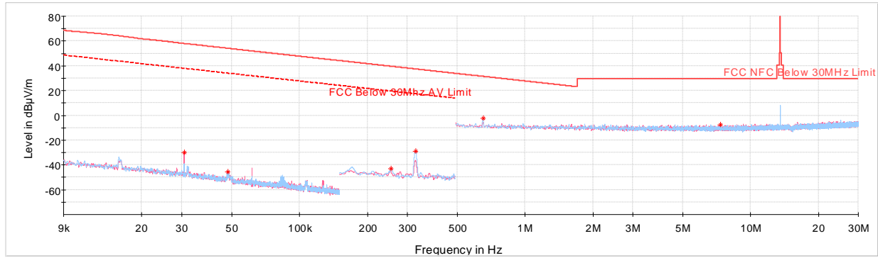
Plot 7-8. Radiated Spurious Emissions 9kHz – 30MHz (CE F 212kbps, with AC/DC Adapter and Magnetic Charger)
