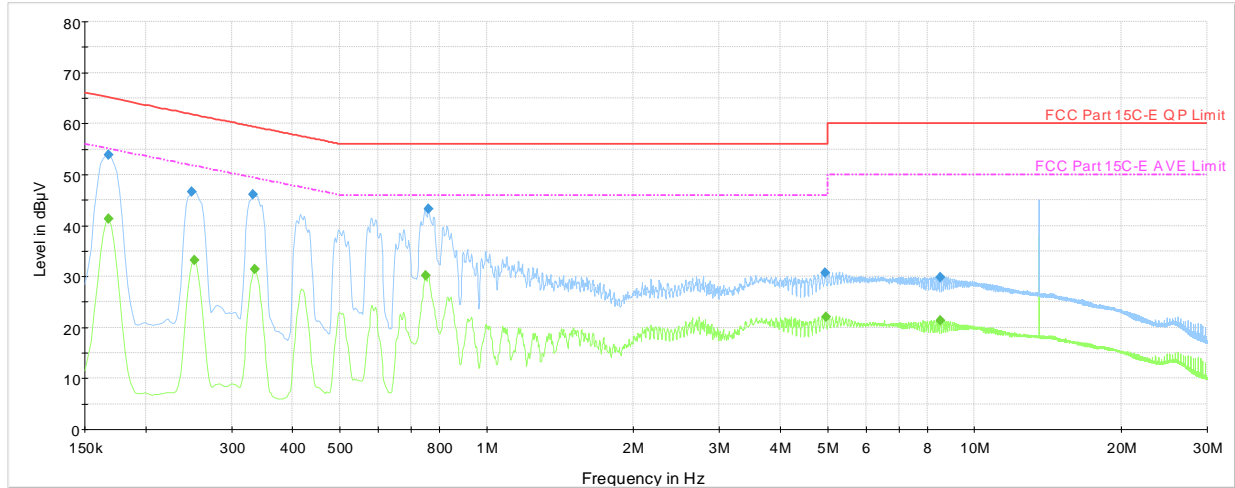
Plot 7-13. AC Line-Conducted Plot (N, CE F 212kbps, with AC/DC Adapter and Magnetic Charger)
