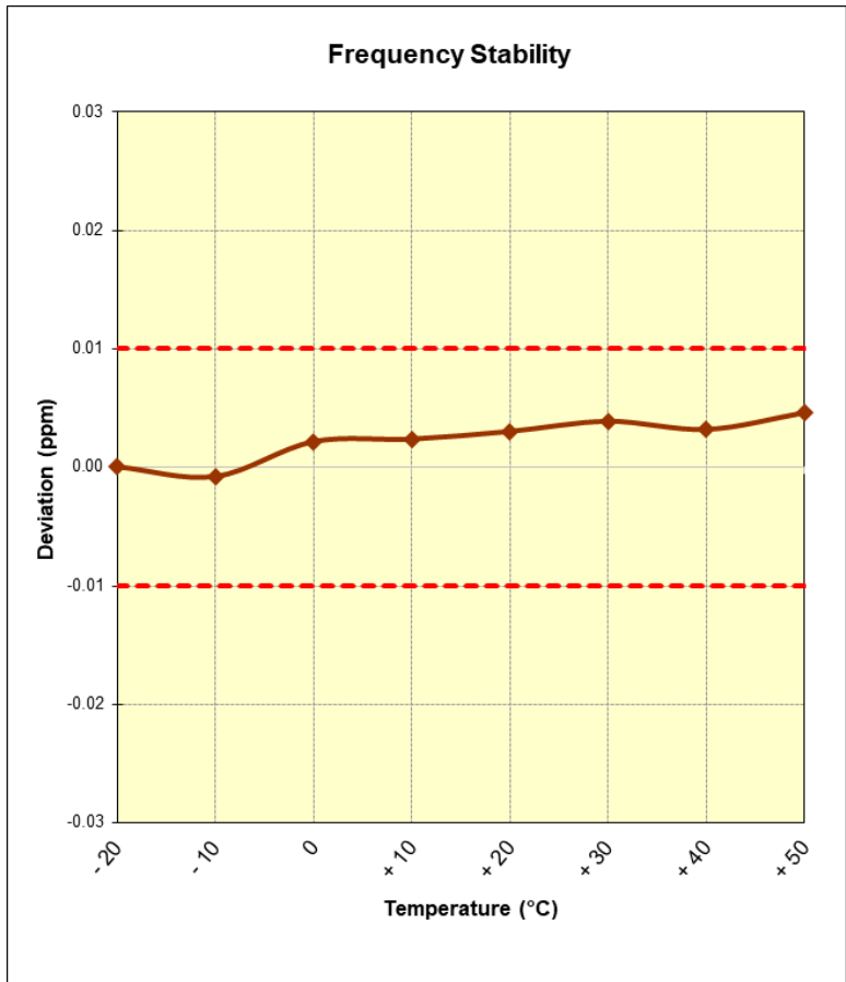
Figure 7-4. Frequency Stability Plot (Reader 100% ASK 1 out of 4)
