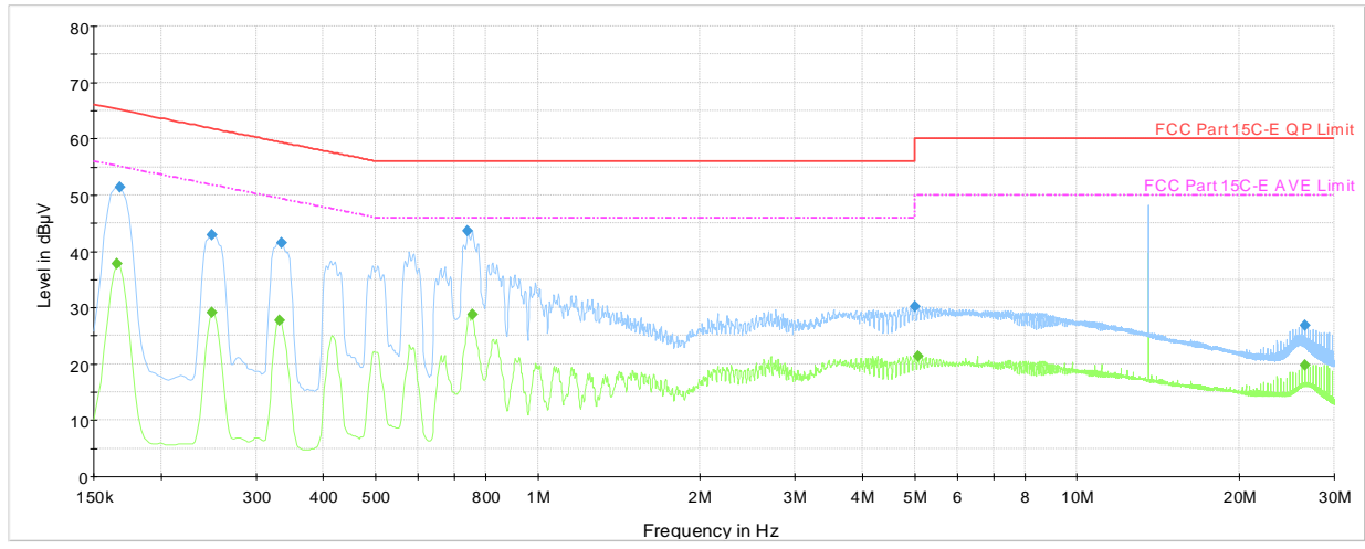
Plot 7-12. AC Line-Conducted Plot (L1, CE F 212kbps, with AC/DC Adapter and Magnetic Charger)
