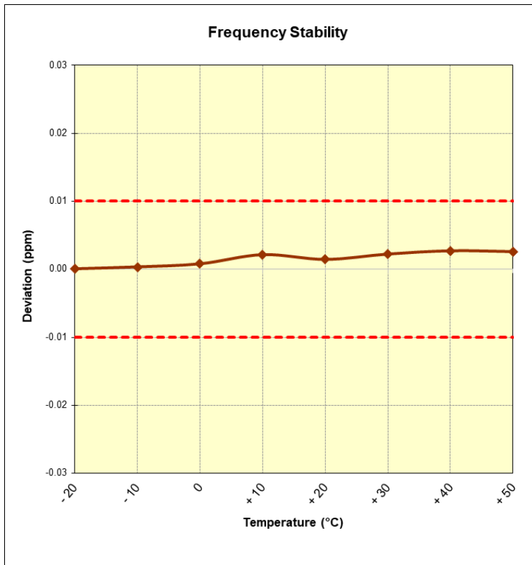
Figure 7-3. Frequency Stability Plot (CE F 212kbps)
