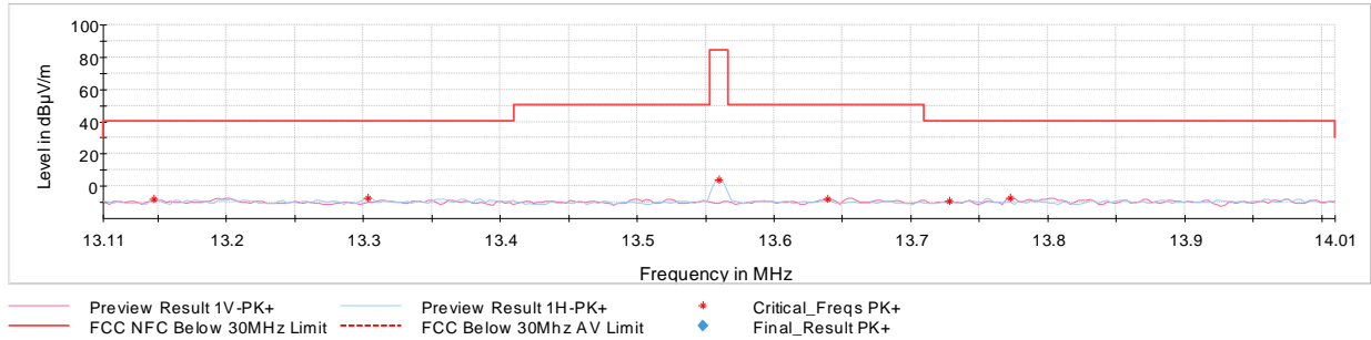
Plot 7-6. In Band Radiated Spurious Emissions (CE F 212kbps, with AC/DC Adapter and Magnetic Charger)
