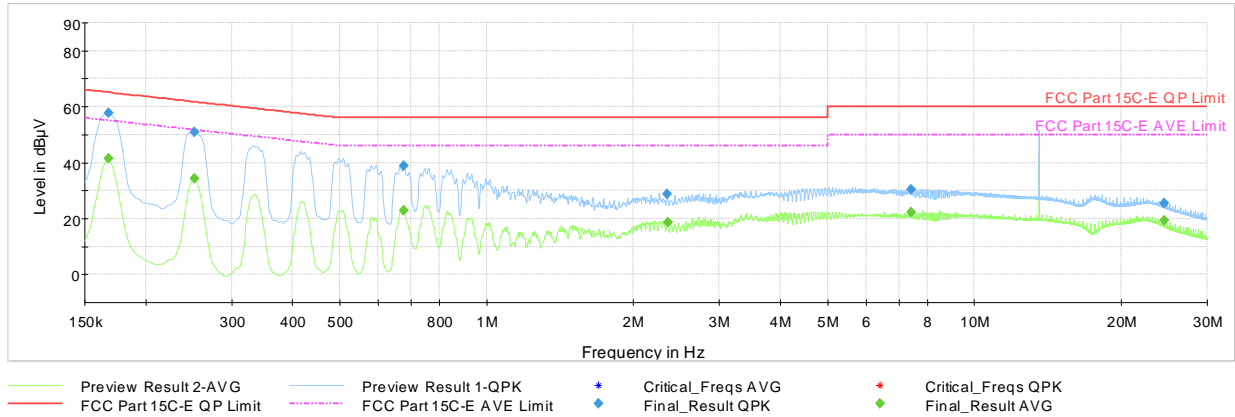
Plot 7-13. AC Line-Conducted Plot (N, CE F 212kbps, with AC/DC Adapter and Magnetic Charger)
