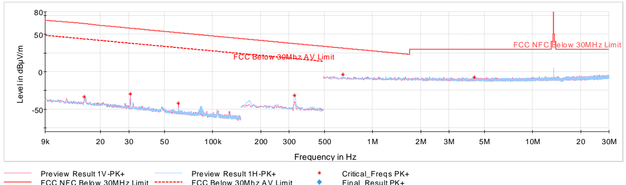
Plot 7-9. Radiated Spurious Emissions 9kHz – 30MHz (Reader A 848kbps, with AC/DC Adapter and Magnetic Charger)
