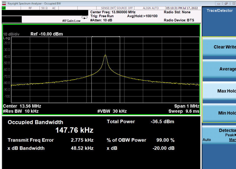
Plot 7-2. 20dB and 99% Bandwidth Plot (CE B 106kbps)
