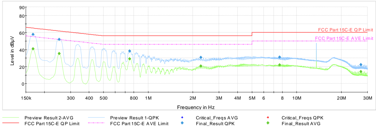
Plot 7-12. AC Line-Conducted Plot (L1, CE F 212kbps, with AC/DC Adapter and Magnetic Charger)
