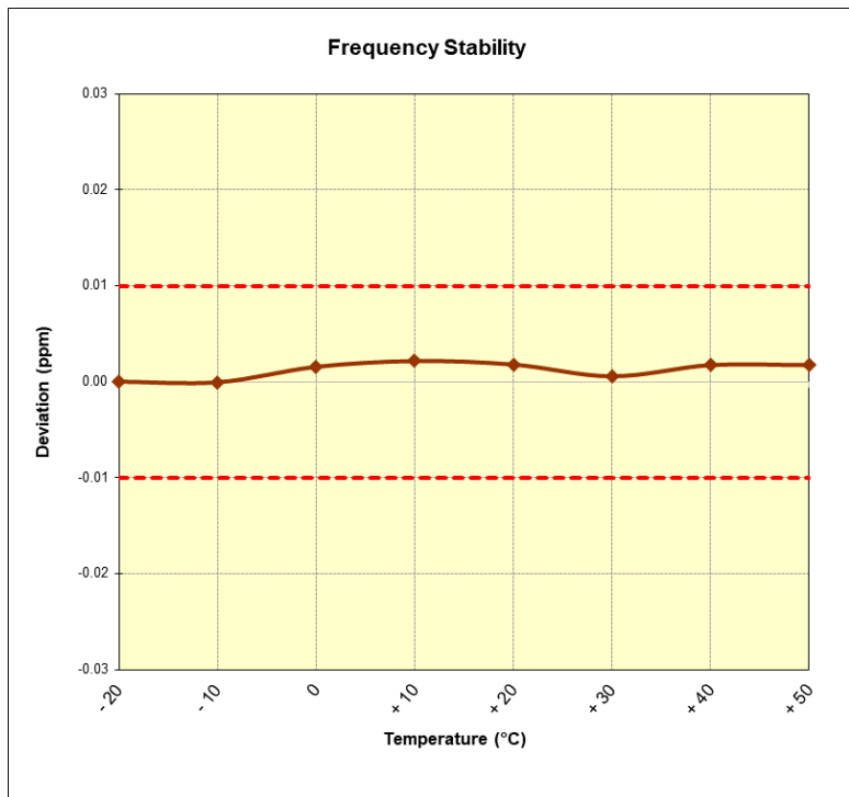
Figure 7-4. Frequency Stability Plot (Reader 100% ASK 1 out of 4)
