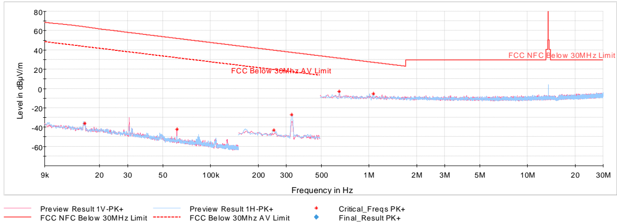
Plot 7-8. Radiated Spurious Emissions 9kHz – 30MHz (CE F 212kbps, with AC/DC Adapter and Magnetic Charger)
