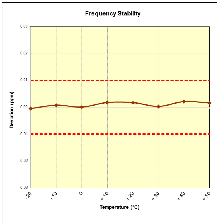
Figure 7-3. Frequency Stability Plot (CE F 212kbps)
