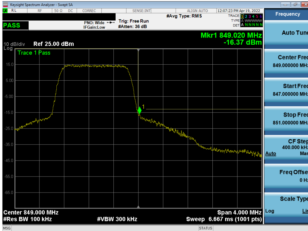
Plot 7-29. Upper BE Plot (LTE Band 5 – 1.4MHz QPSK – Full RB Configuration)
