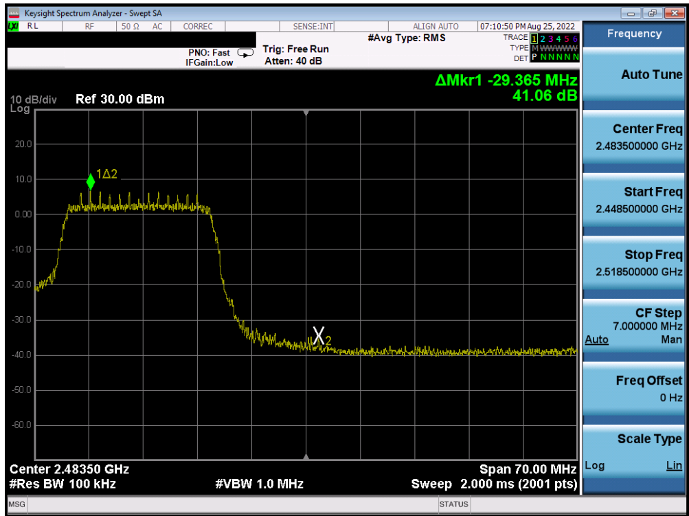
Plot 7-37. Band Edge Plot (802.11n MCS0 – Ch. 11)
