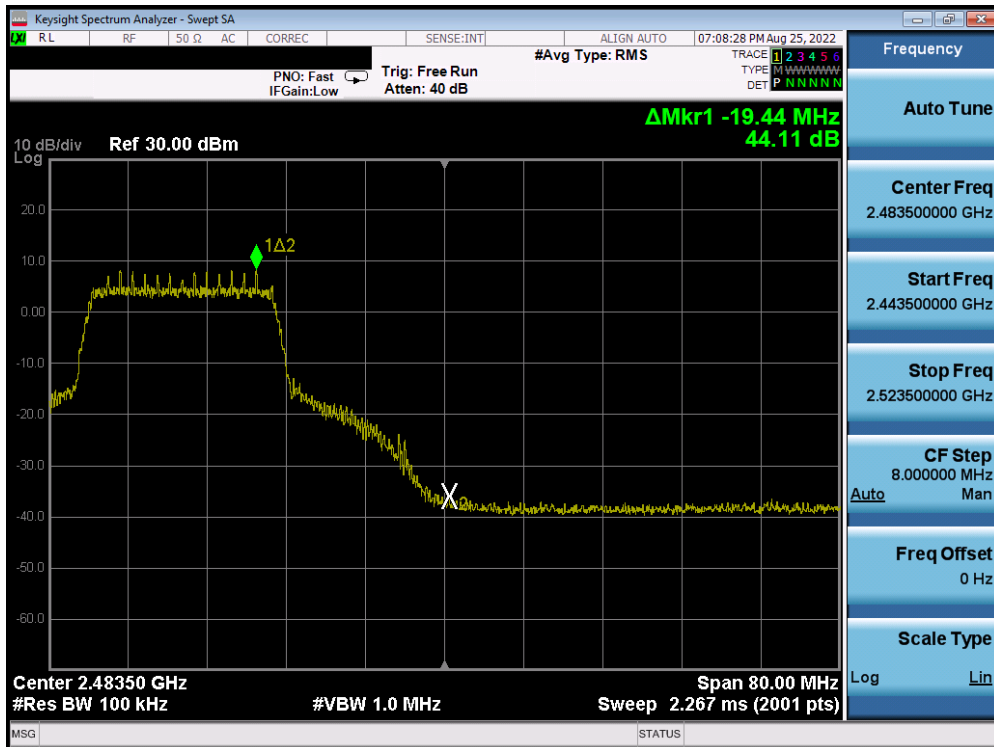
Plot 7-36. Band Edge Plot (802.11n MCS0 – Ch. 10)
