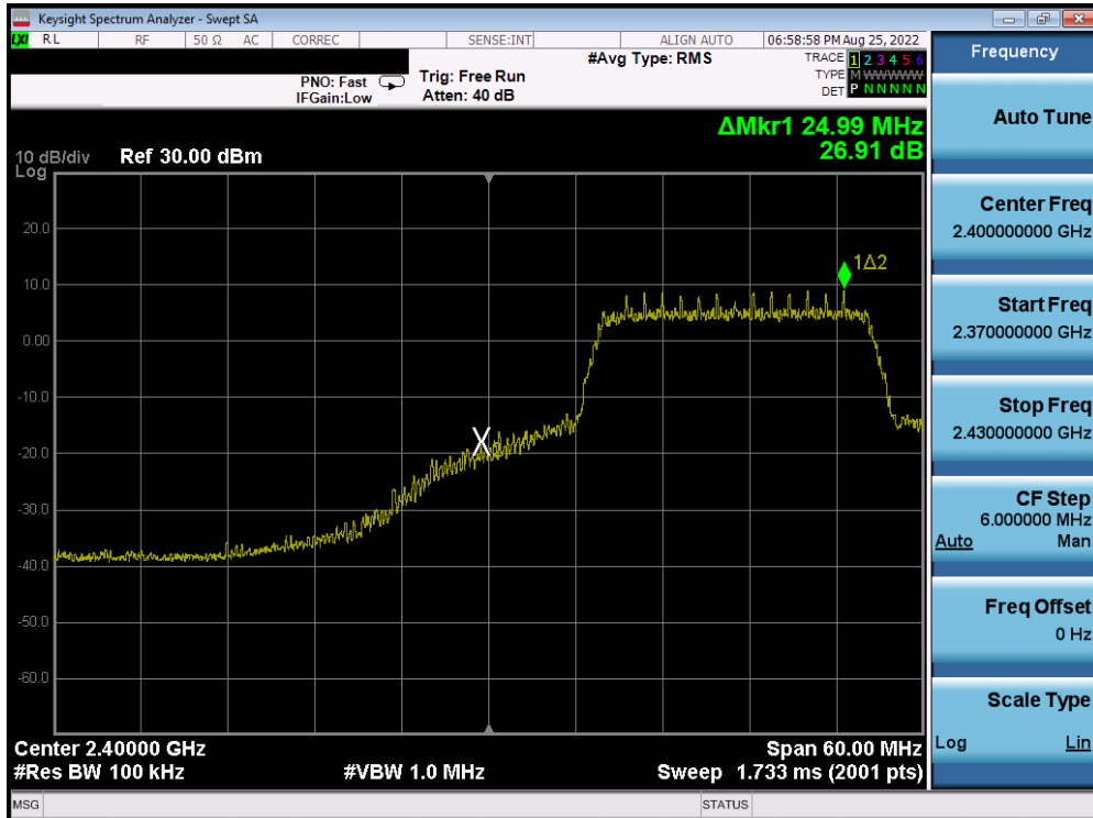
Plot 7-35. Band Edge Plot (802.11n MCS0 – Ch. 2)
