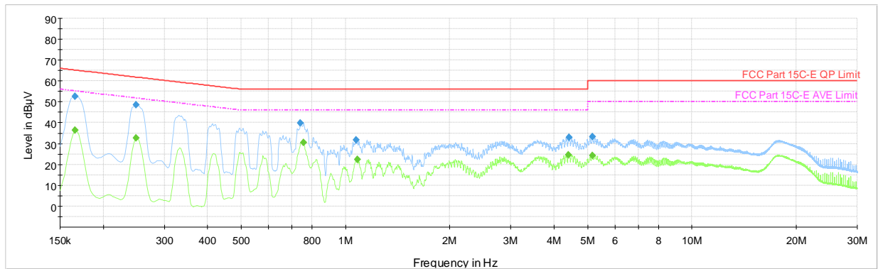
Plot 7-74. AC Line Conducted Plot 802.11b - Ch.6 (L1, with AC/DC Adapter + Laptop Charger)
