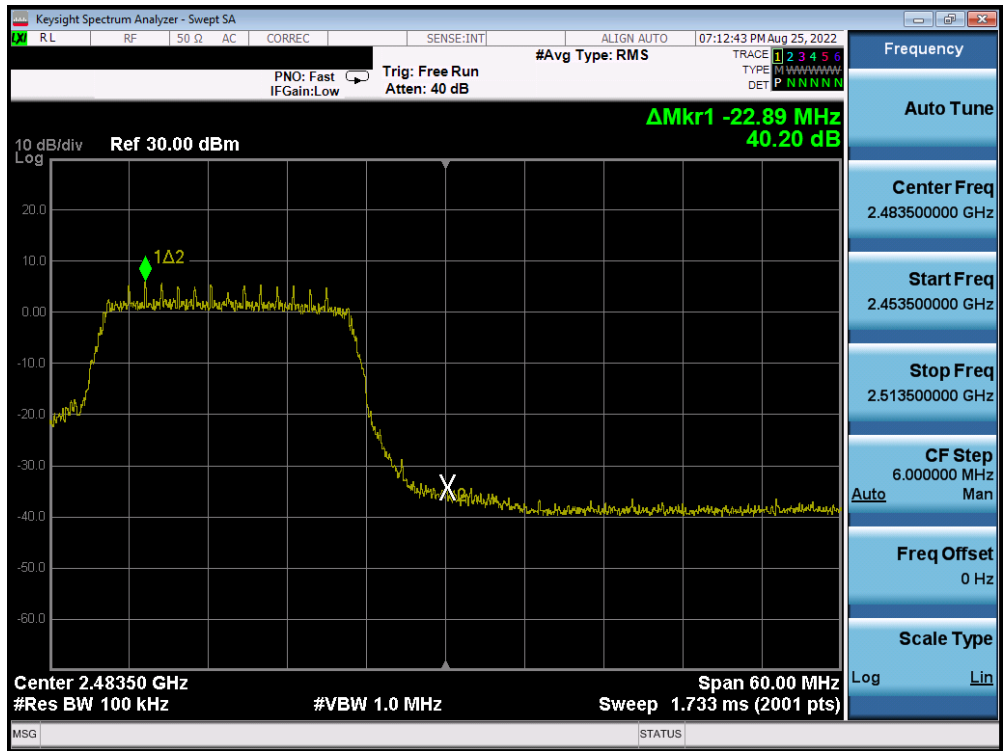
Plot 7-38. Band Edge Plot (802.11n MCS0 – Ch. 12)
