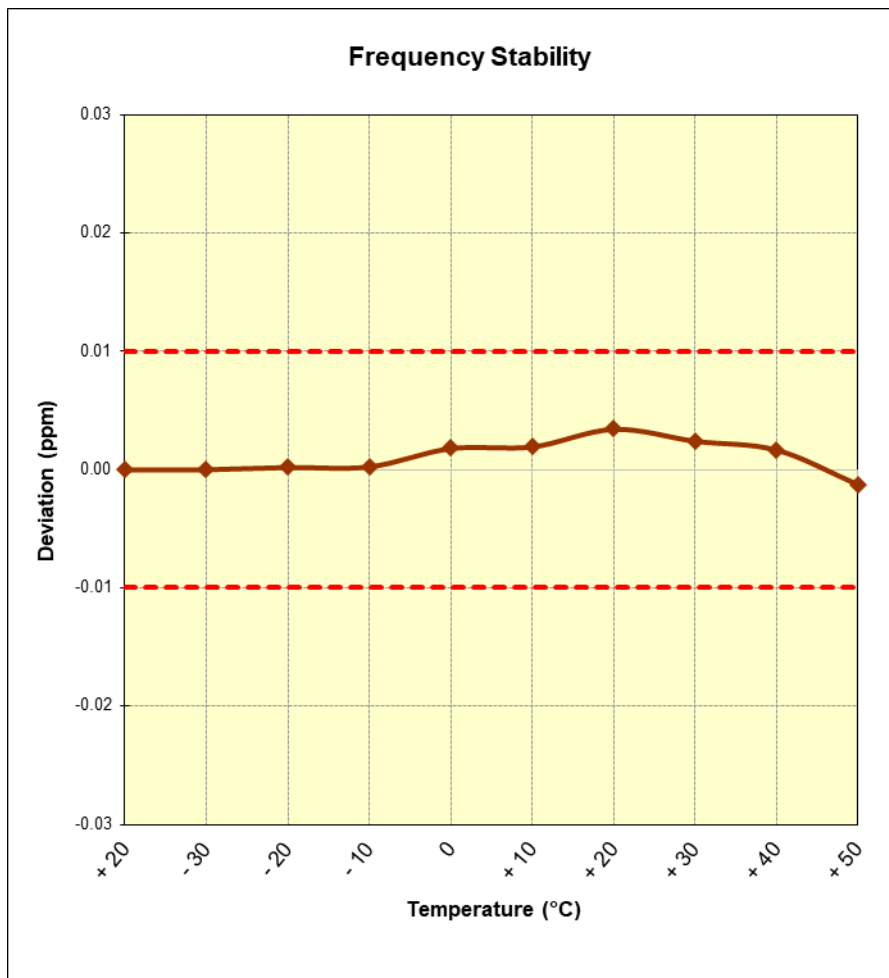
Figure 7-4. Frequency Stability Plot (Reader 100% ASK 1 out of 256)
