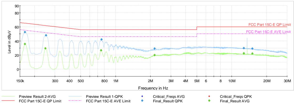
Plot 7-15. AC Line-Conducted Plot (N, Reader A 848kbps, with AC/DC Adapter and Magnetic Charger)
