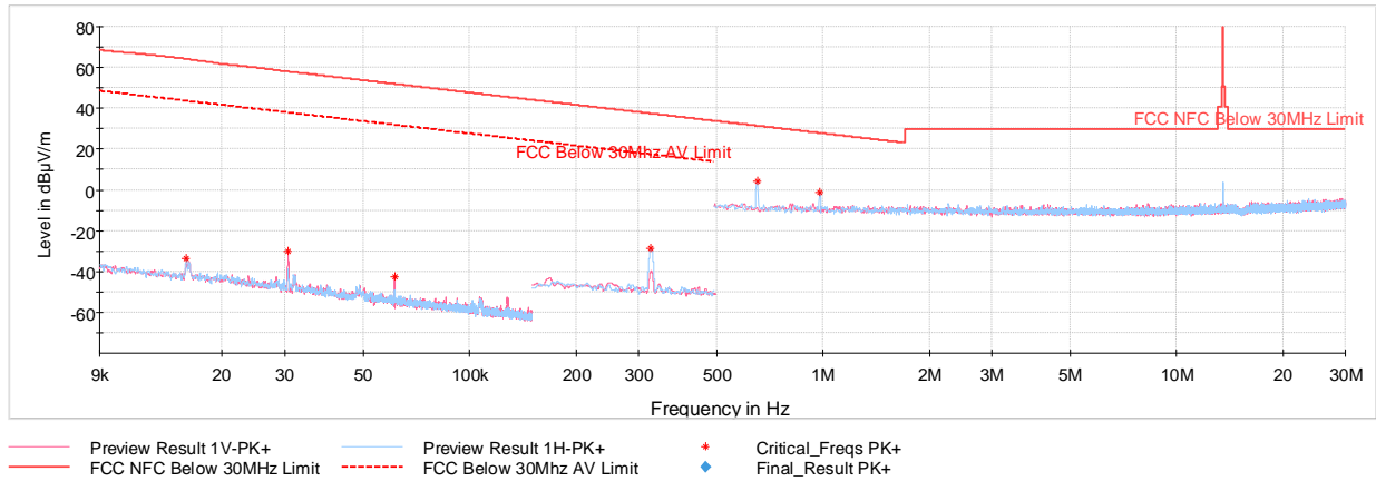
Plot 7-8. Radiated Spurious Emissions 9kHz – 30MHz (CE A 848kbps, with AC/DC Adapter and Magnetic Charger)
