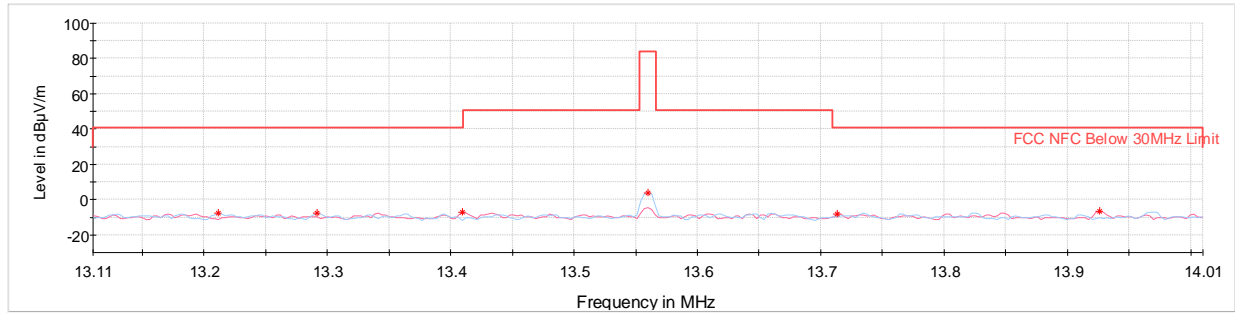
Plot 7-7. In Band Radiated Spurious Emissions (Reader A 848kbps, AC/DC Adapter and Magnetic Charger)
