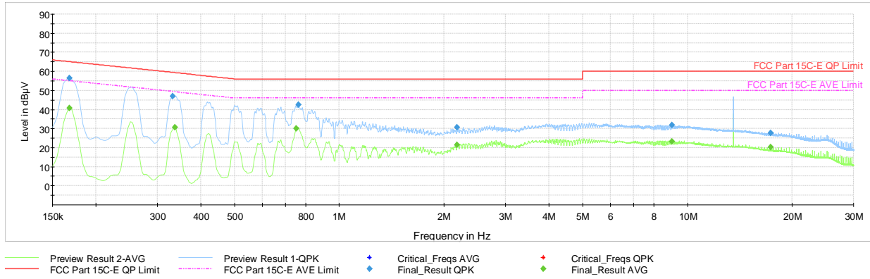
Plot 7-12. AC Line-Conducted Plot (L1, CE A 848kbps, with AC/DC Adapter and Magnetic Charger)
