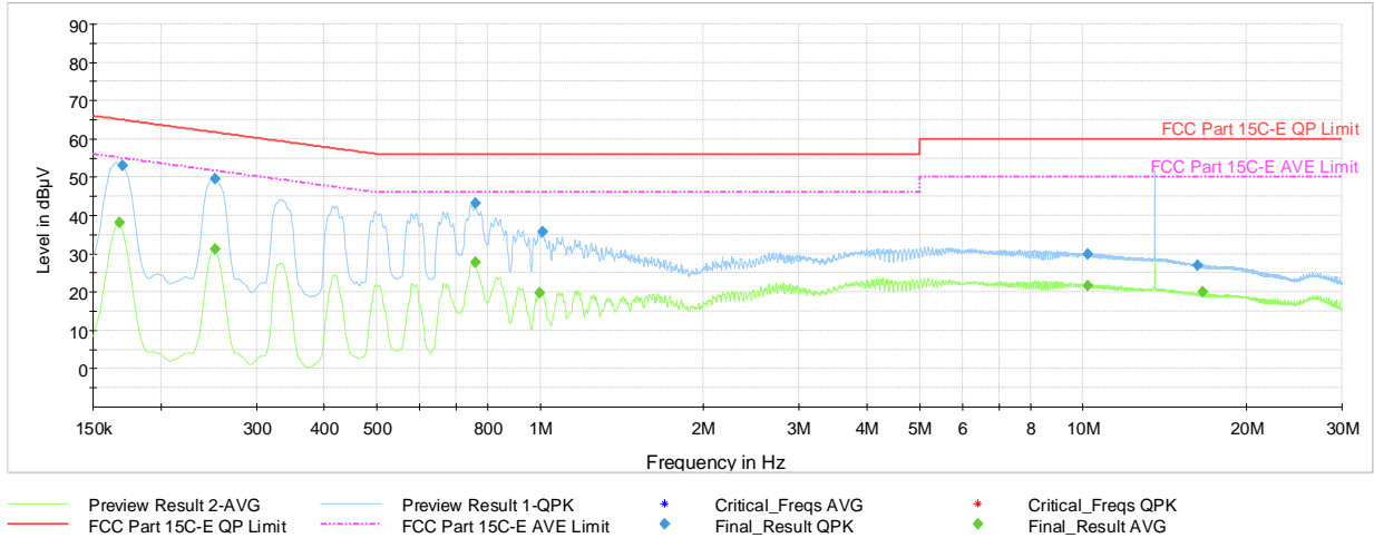
Plot 7-14. AC Line-Conducted Plot (L1, Reader A 848kbps, with AC/DC Adapter and Magnetic Charger)
