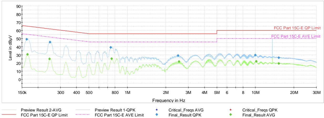
Plot 7-13. AC Line-Conducted Plot (N, CE A 848kbps, with AC/DC Adapter and Magnetic Charger)
