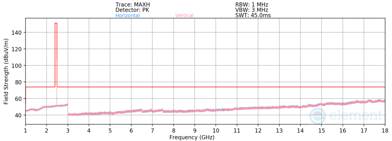
Plot 7-31. Radiated Spurious Emissions above 1GHz (BT GFSK – 2480MHz)
