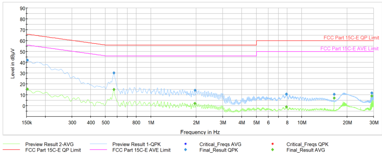
Plot 7-39. AC Line-Conducted Plot (L1, GFSK – 2480MHz, with host PC and lightning cable)
