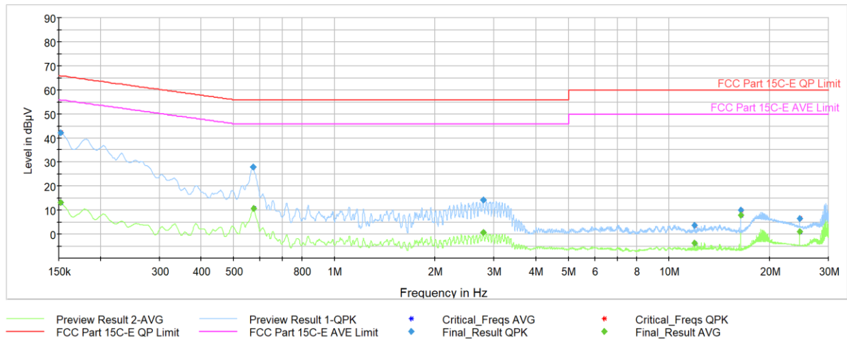
Plot 7-40. AC Line-Conducted Plot (N, GFSK – 2480MHz, with host PC and lightning cable)
