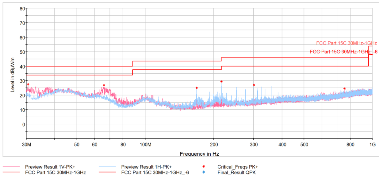
Plot 7-38. Radiated Spurious Emissions Below 1GHz (GFSK – 2480MHz) with AC/DC Adapter and lightning cable
