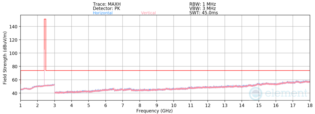
Plot 7-29. Radiated Spurious Emissions above 1GHz (BT GFSK – 2402MHz)
