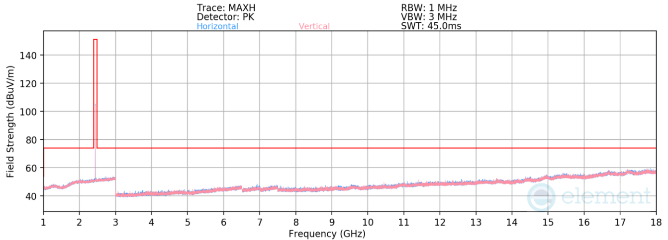
Plot 7-30. Radiated Spurious Emissions above 1GHz (BT GFSK – 2441MHz)
